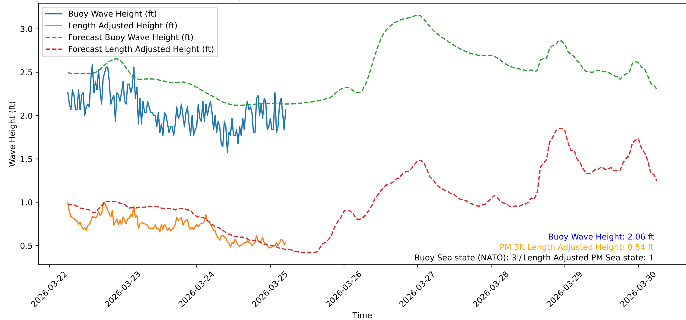
Wave Heights over Time for Oceanside Harbor at 2026-03-25 05:50:31
