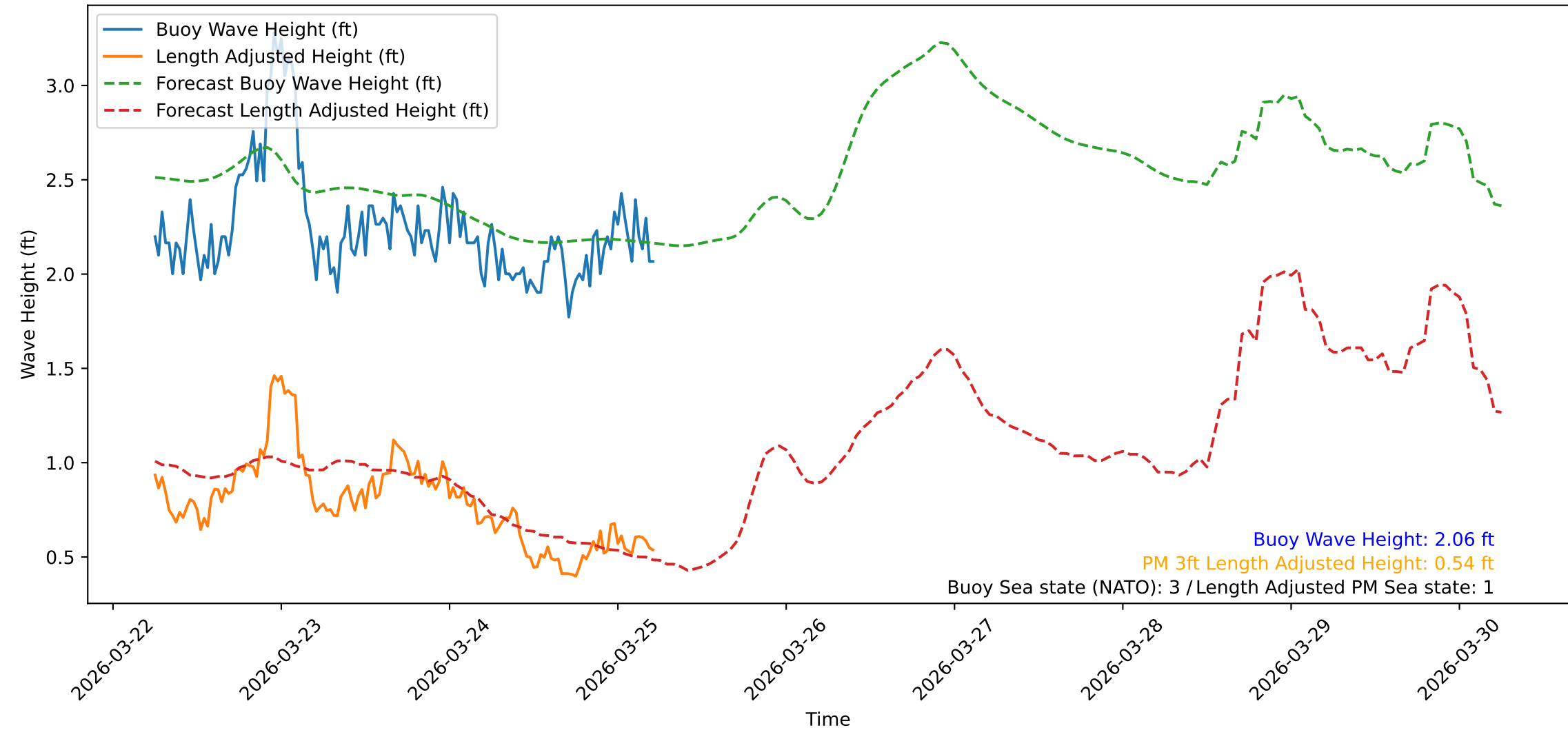
Wave Heights over Time for Green Beach at 2026-03-25 05:51:09
