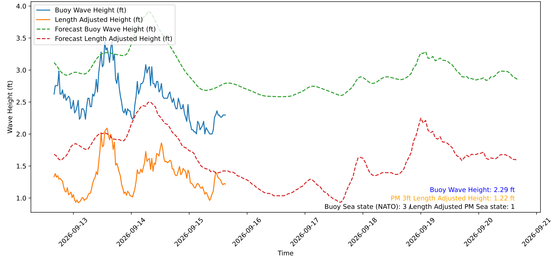
Wave Heights over Time for Red Beach at 2026-09-15 15:40:49
