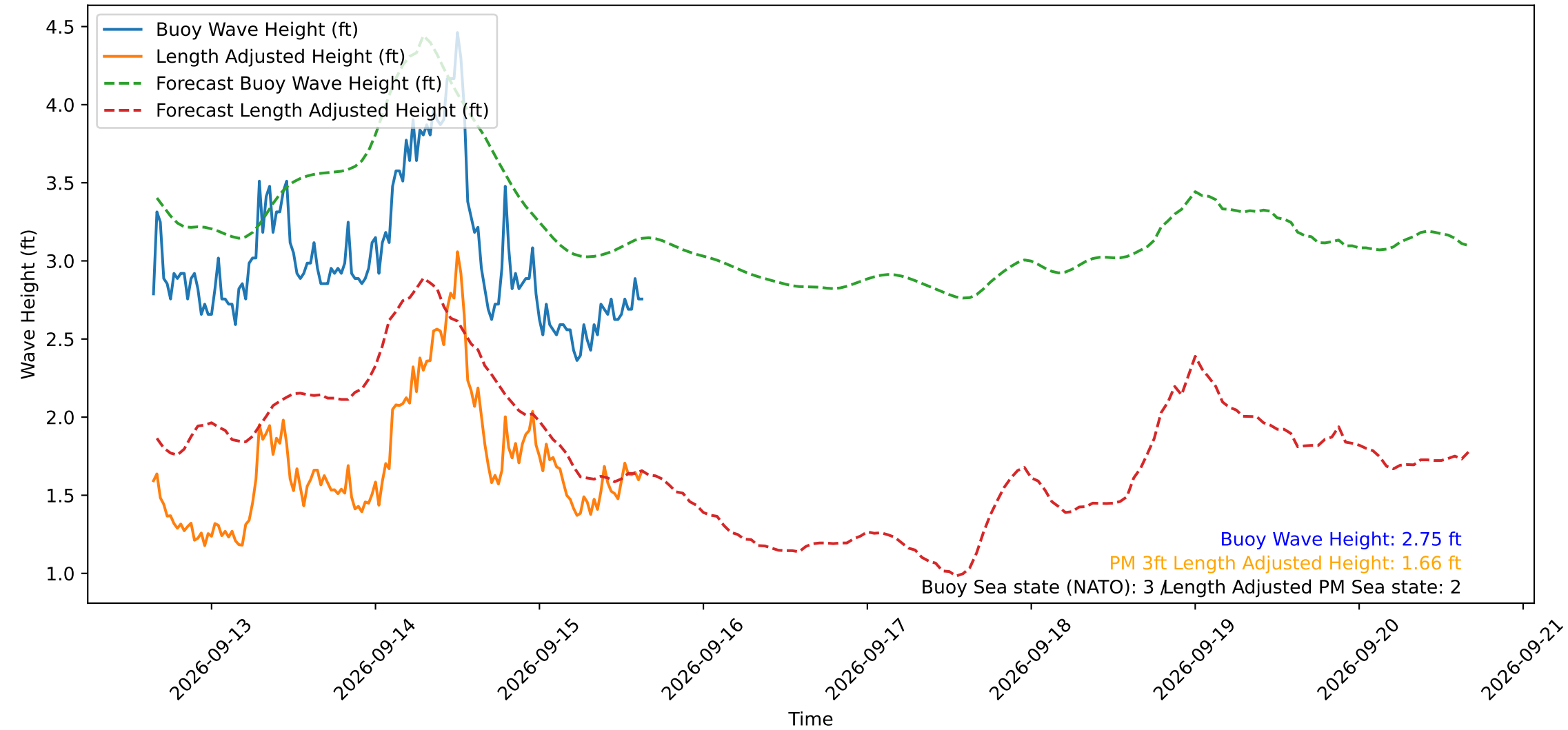
Wave Heights over Time for Oceanside Harbor at 2026-09-15 15:40:29
