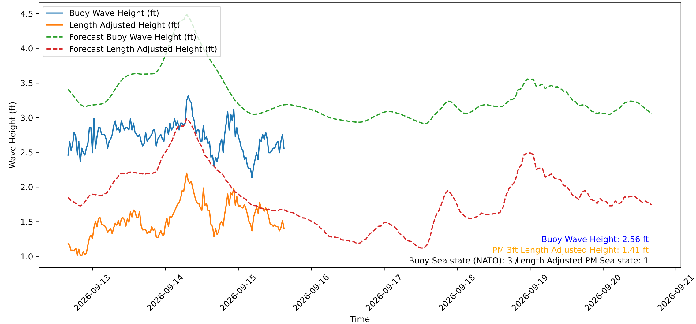
Wave Heights over Time for Green Beach at 2026-09-15 15:41:11
