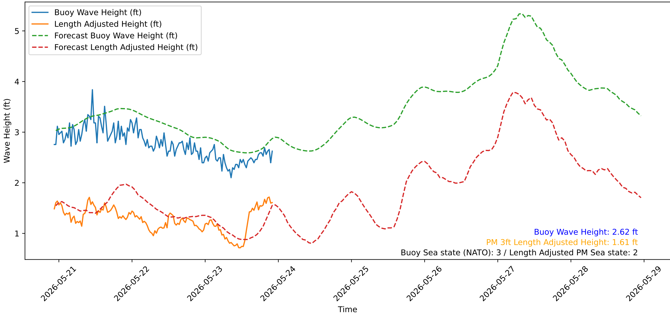
Wave Heights over Time for Oceanside Harbor at 2026-05-23 22:40:32
