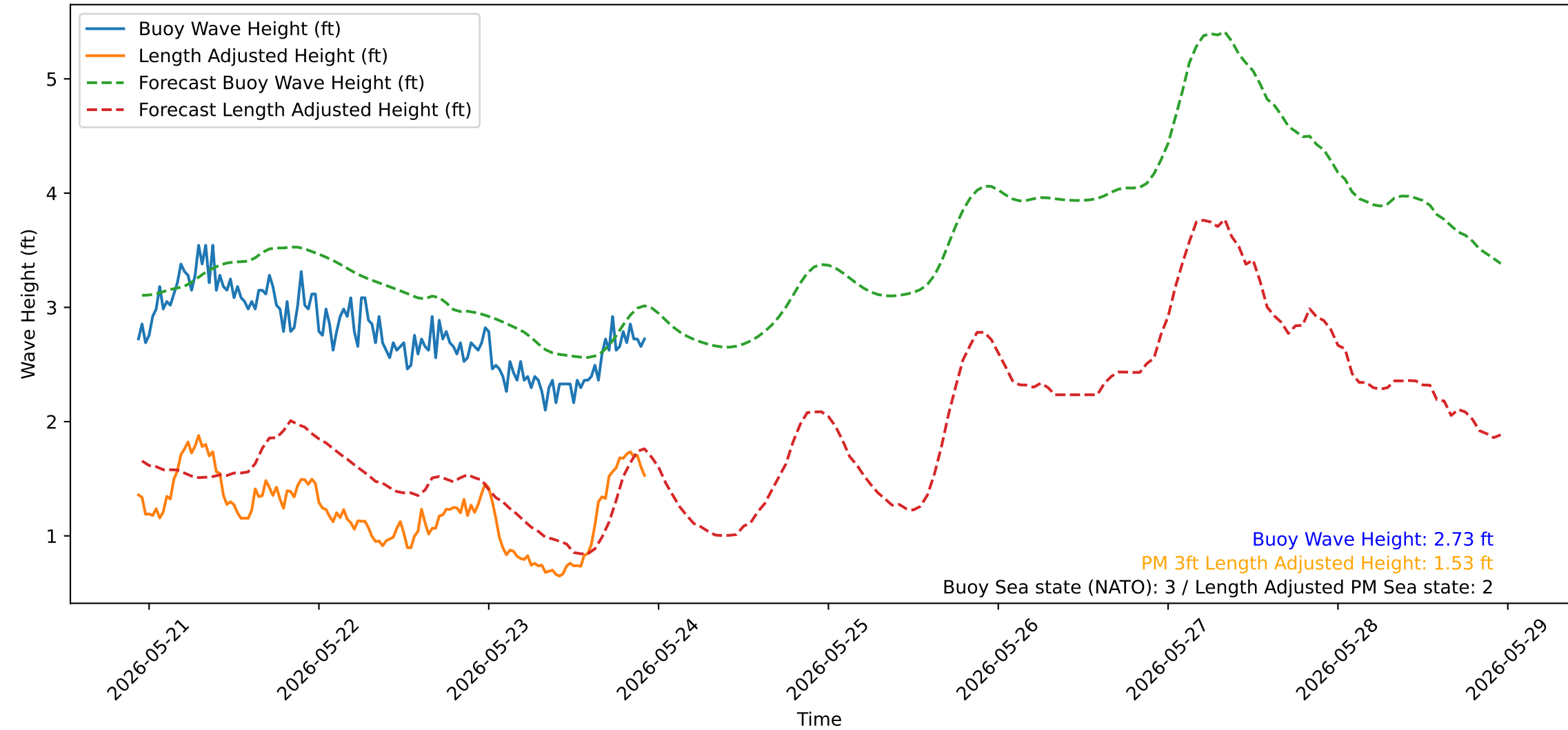
Wave Heights over Time for Green Beach at 2026-05-23 22:41:14
