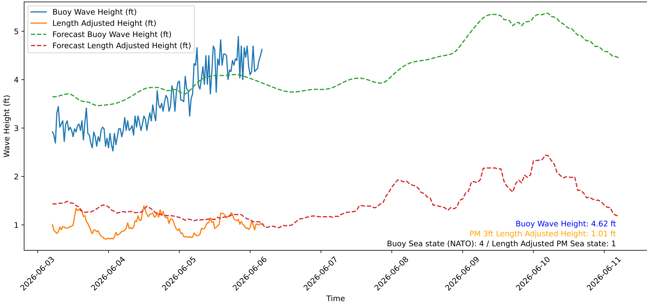
Wave Heights over Time for Red Beach at 2026-06-06 04:50:46
