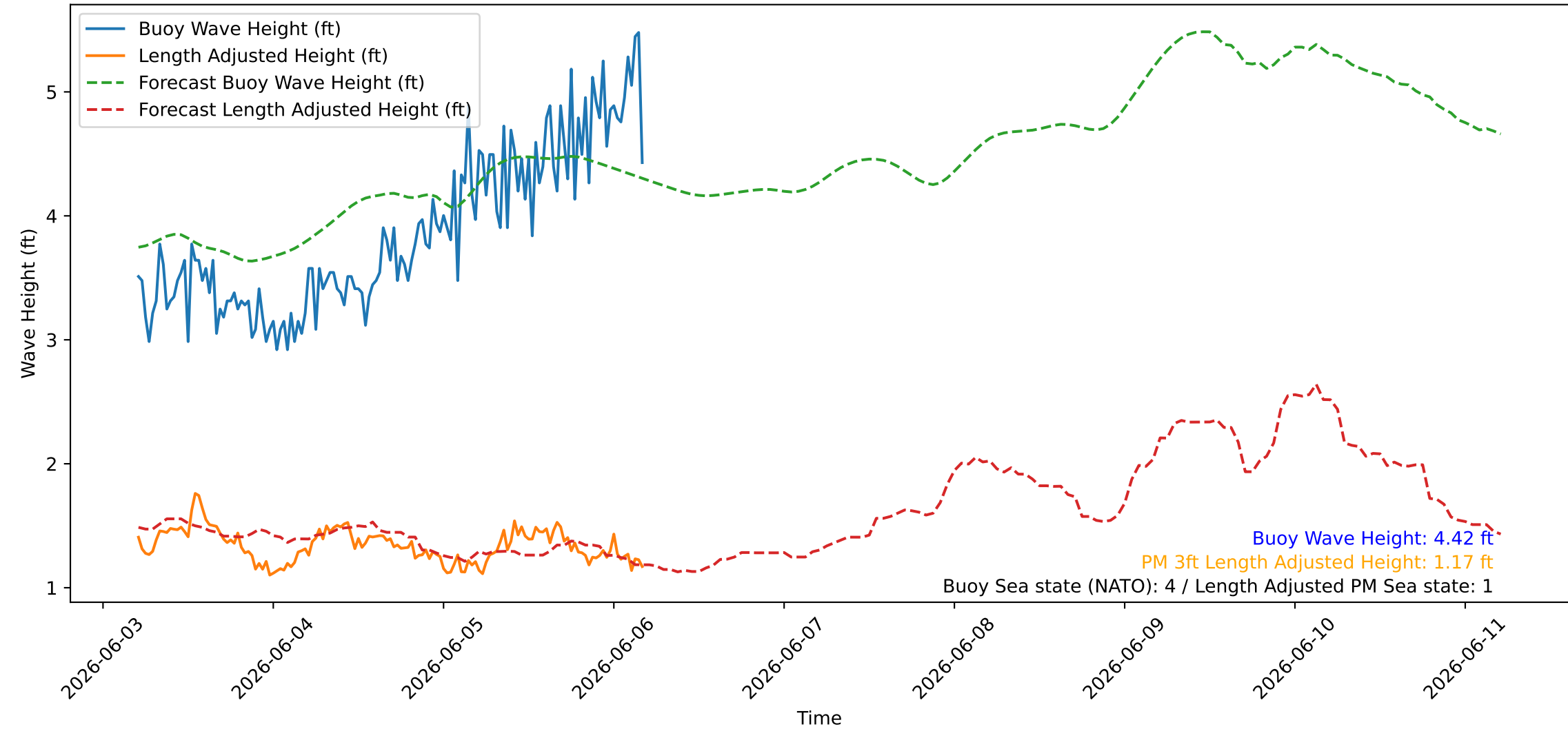
Wave Heights over Time for Oceanside Harbor at 2026-06-06 04:50:26
