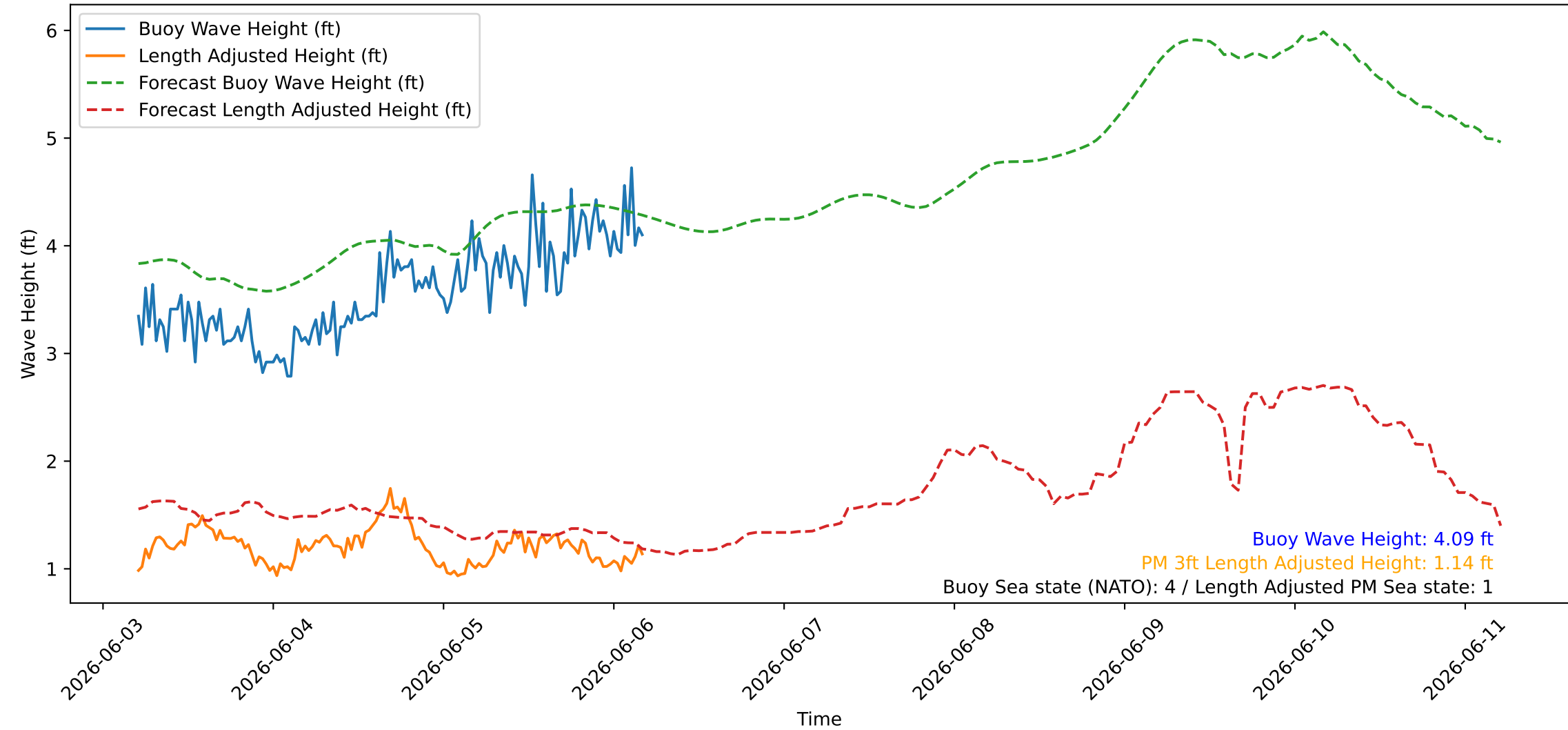
Wave Heights over Time for Green Beach at 2026-06-06 04:51:09
