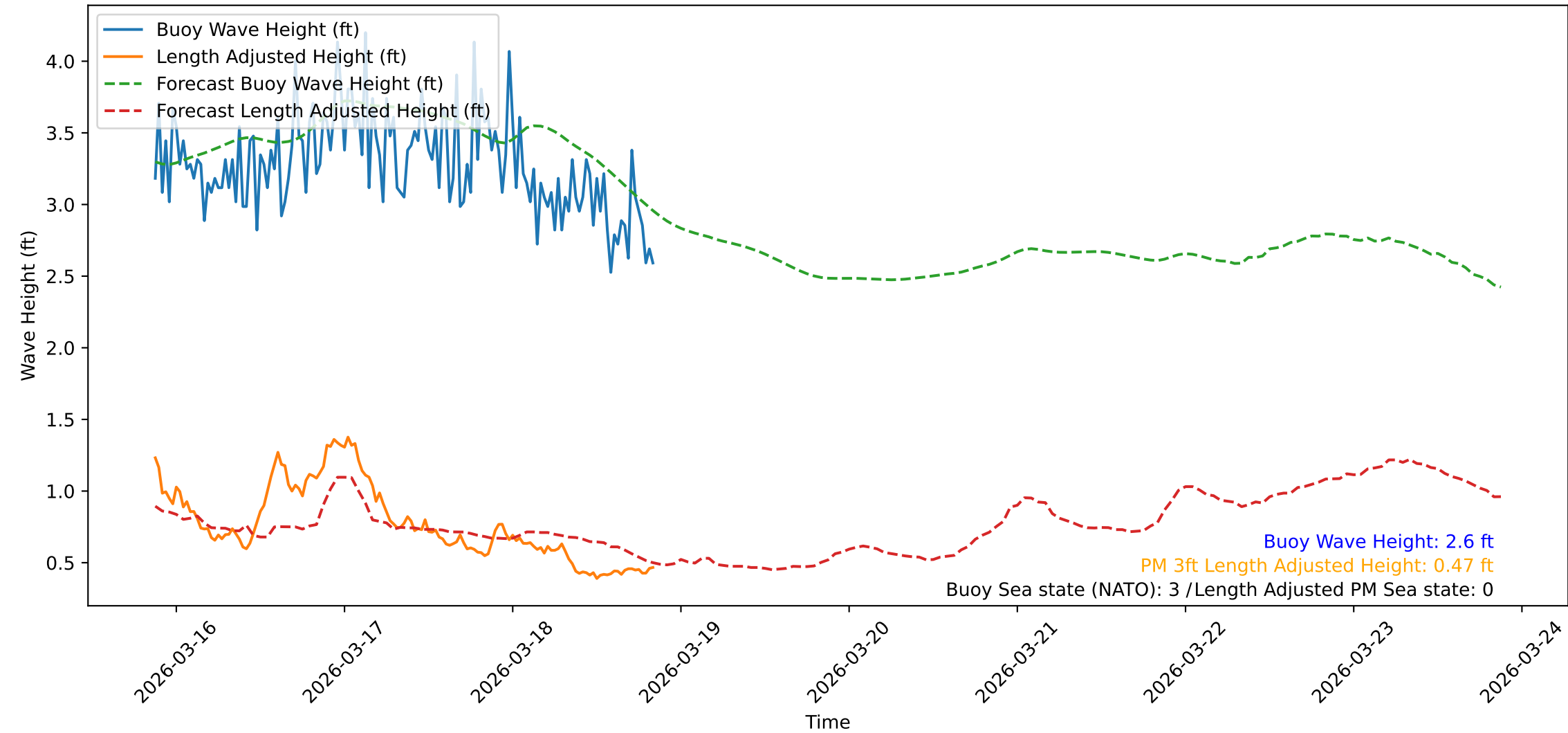
Wave Heights over Time for Green Beach at 2026-03-18 20:51:09
