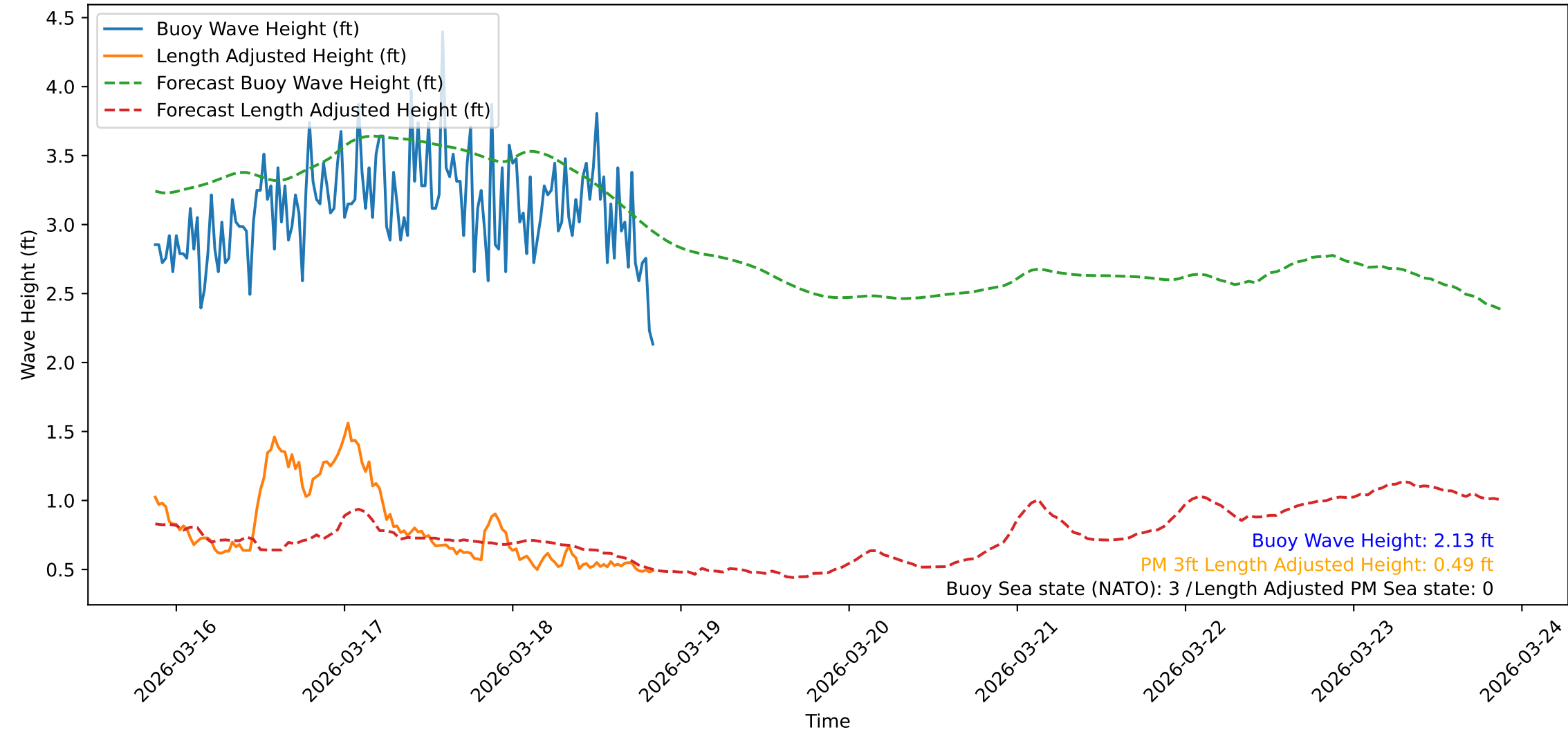
Wave Heights over Time for Oceanside Harbor at 2026-03-18 20:50:31
