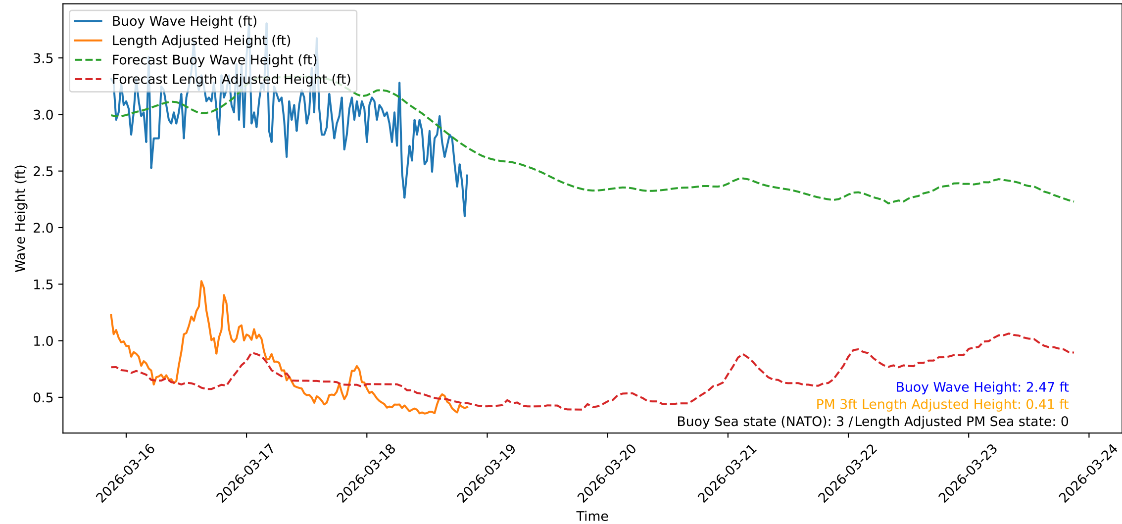
Wave Heights over Time for Red Beach at 2026-03-18 20:50:47
