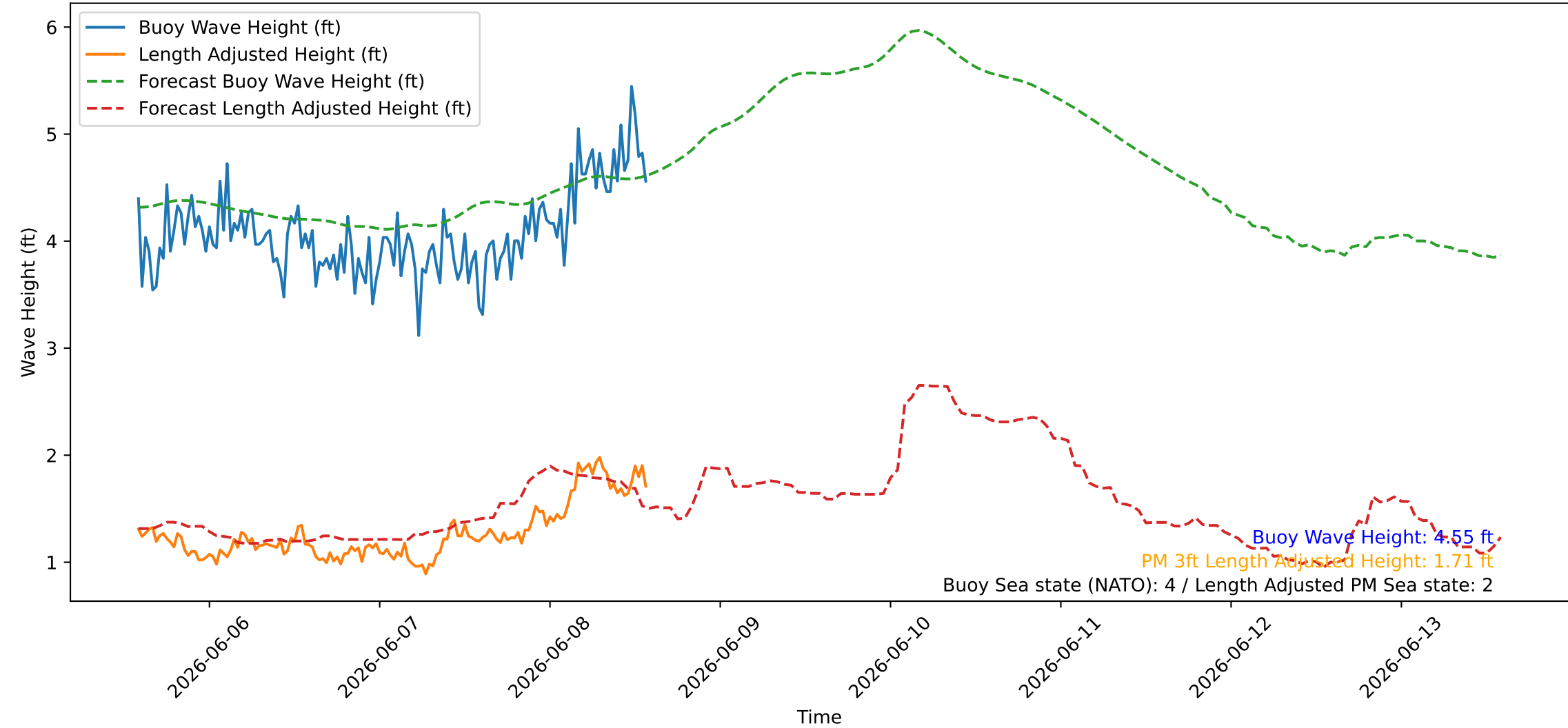
Wave Heights over Time for Green Beach at 2026-06-08 14:11:08
