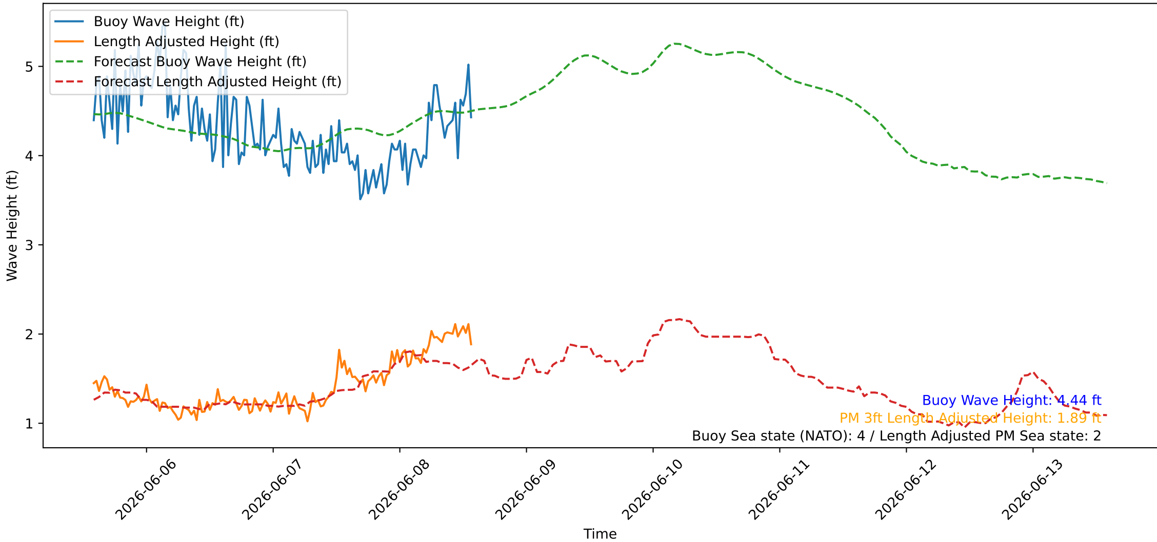
Wave Heights over Time for Oceanside Harbor at 2026-06-08 14:10:26
