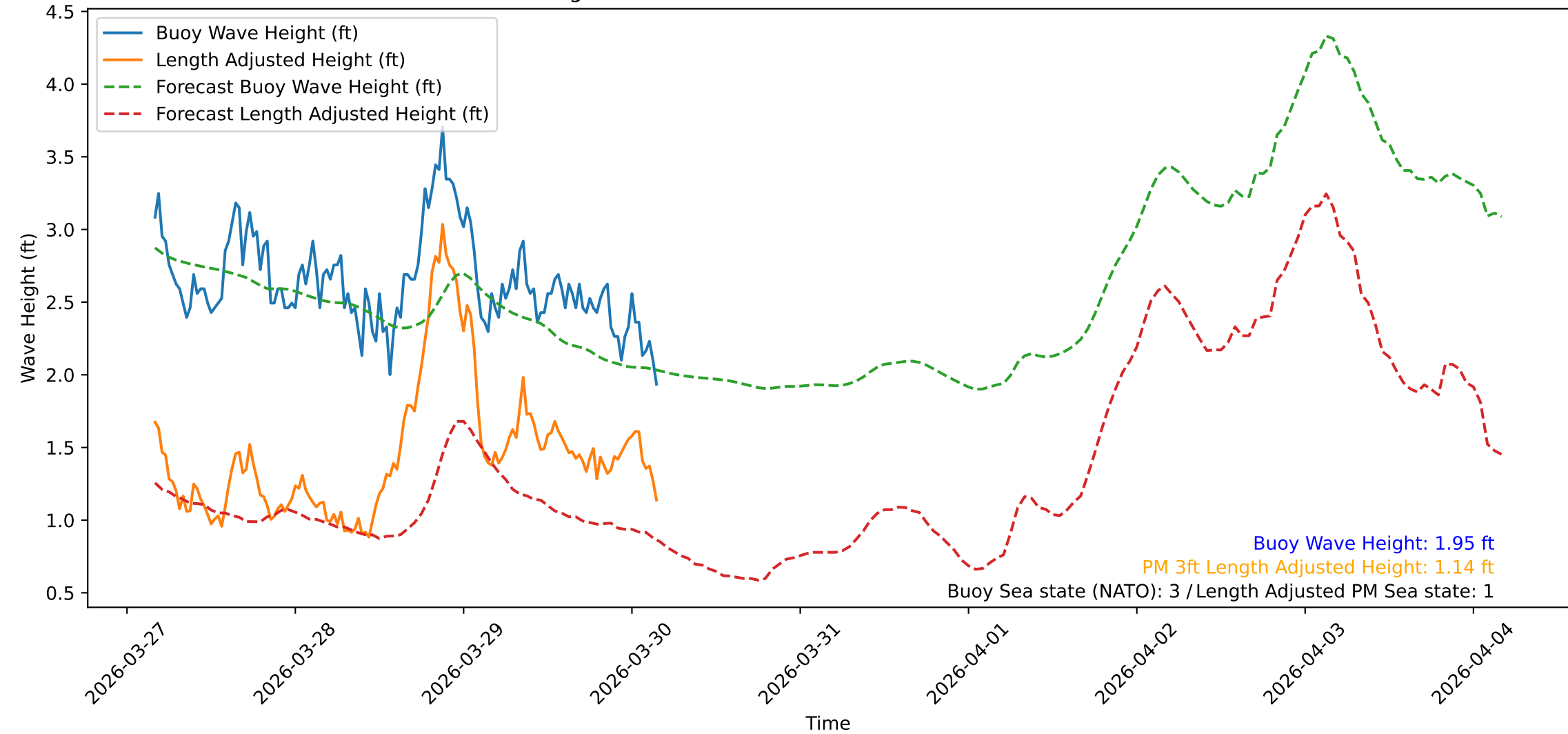
Wave Heights over Time for Green Beach at 2026-03-30 04:11:10
