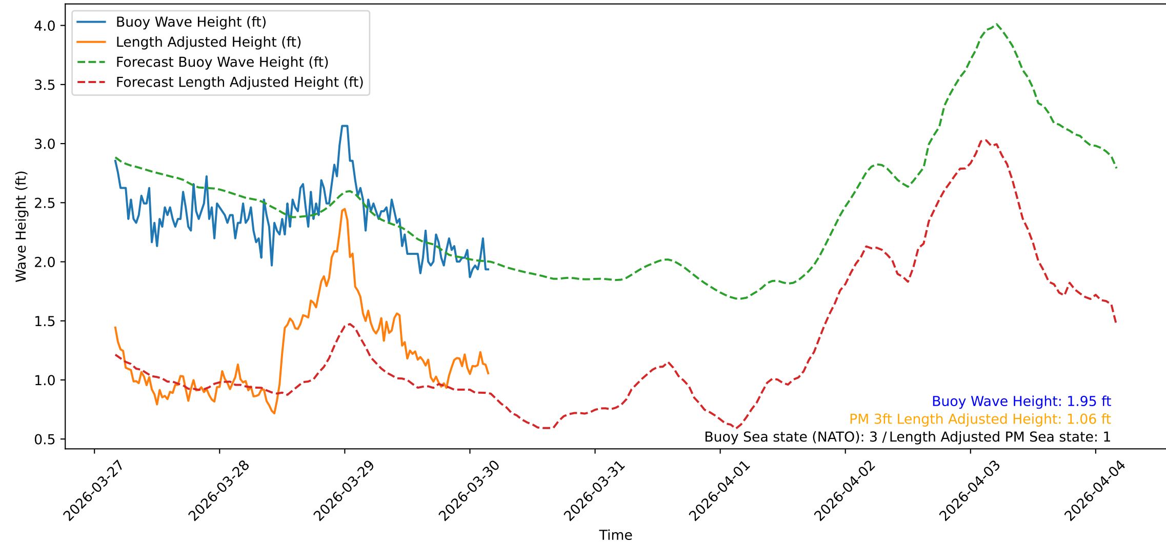
Wave Heights over Time for Oceanside Harbor at 2026-03-30 04:10:31
