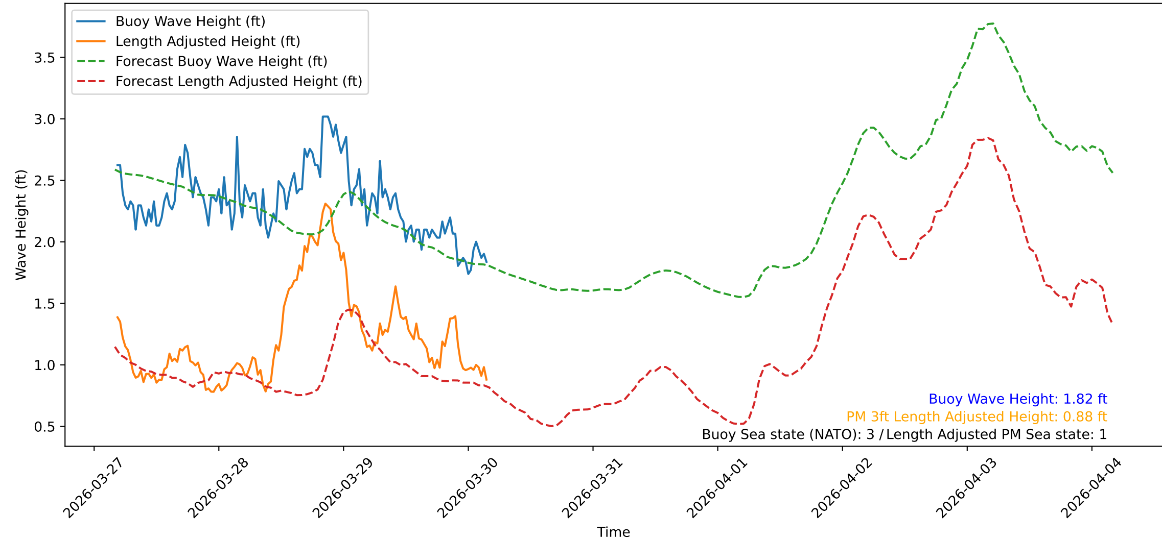
Wave Heights over Time for Red Beach at 2026-03-30 04:10:47
