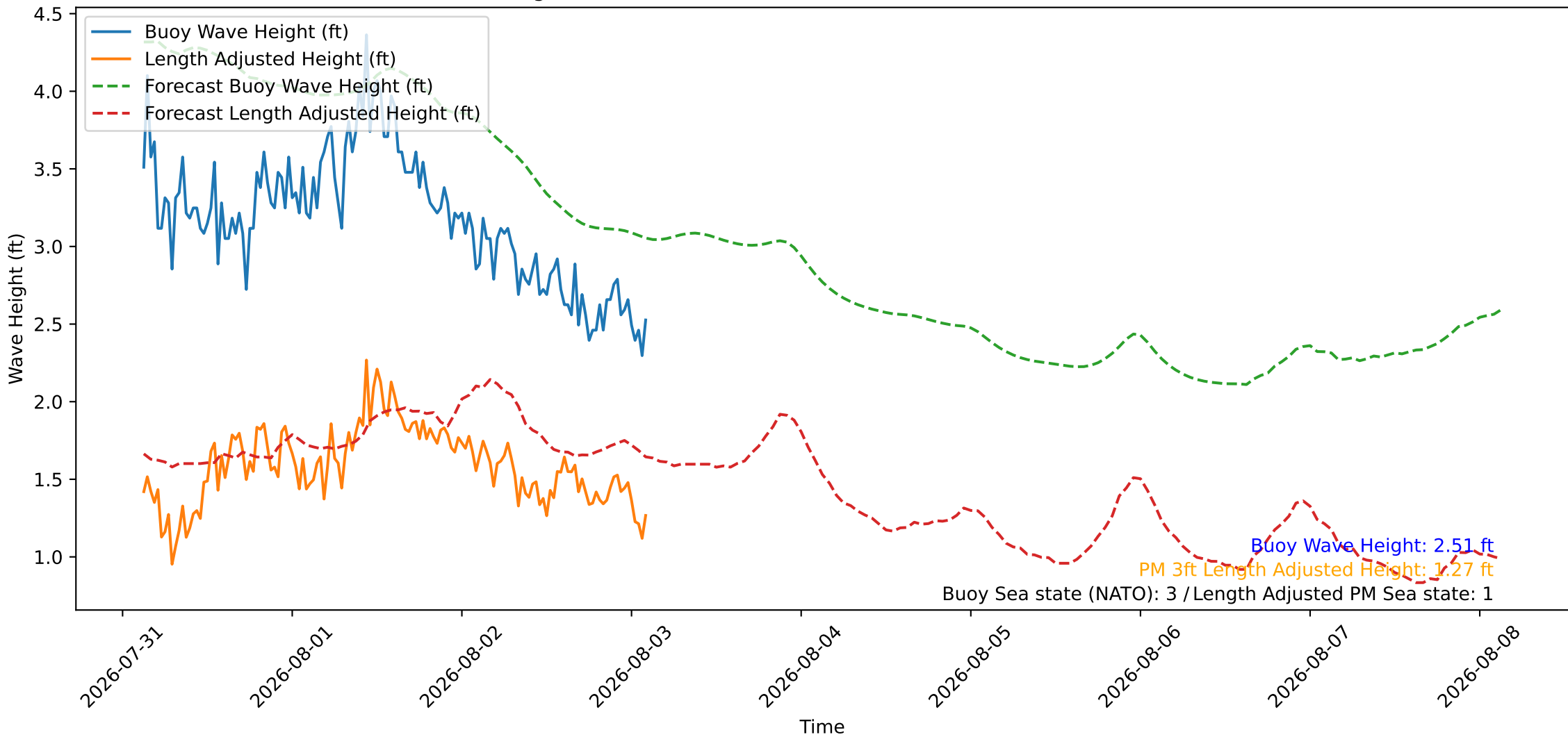
Wave Heights over Time for Oceanside Harbor at 2026-08-03 03:00:26
