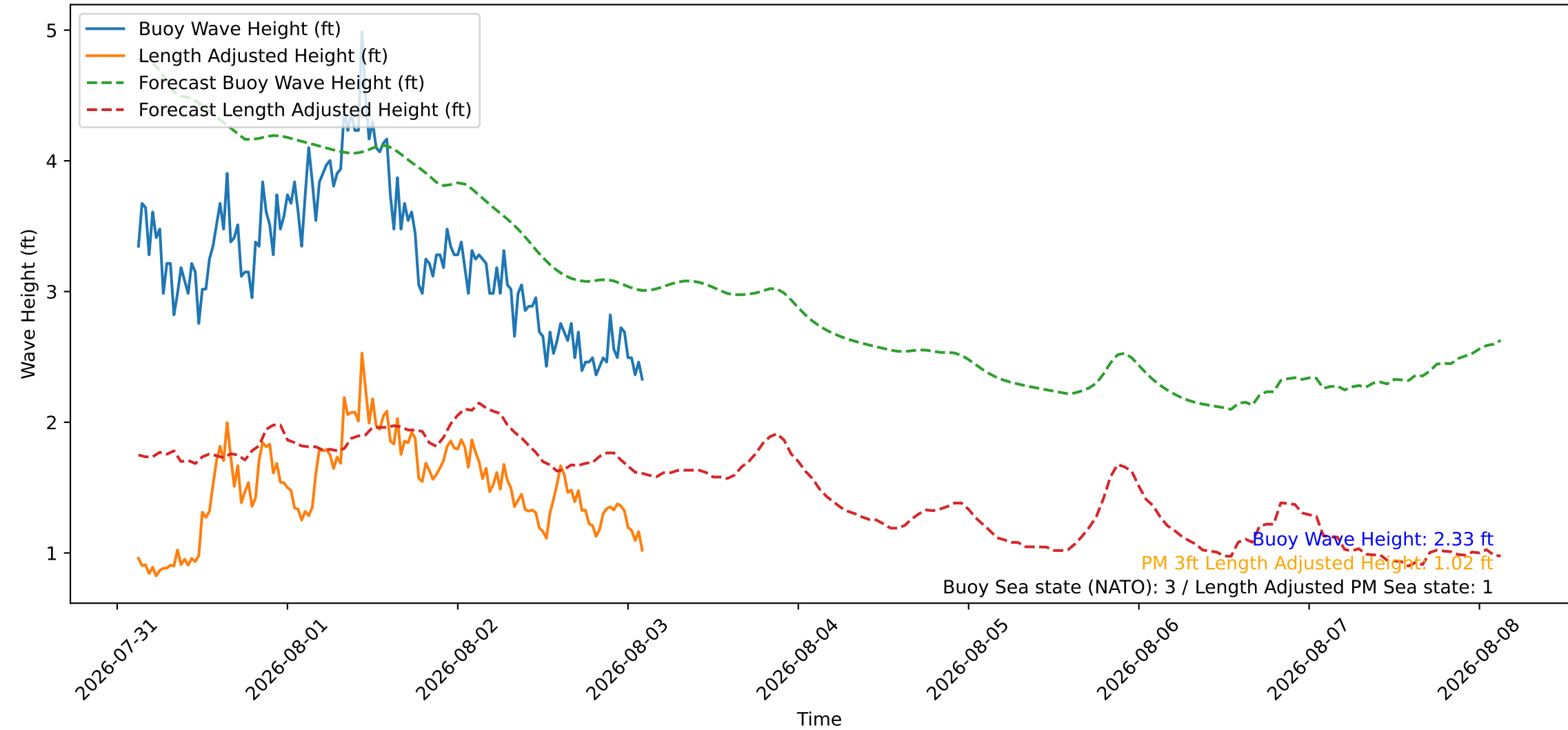
Wave Heights over Time for Green Beach at 2026-08-03 03:01:08
