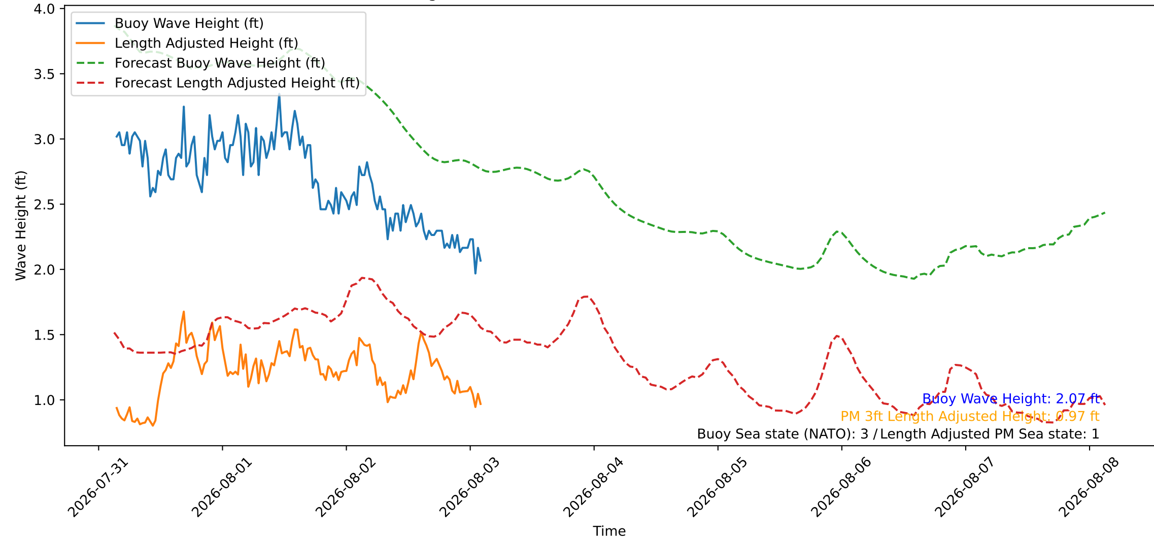
Wave Heights over Time for Red Beach at 2026-08-03 03:00:46
