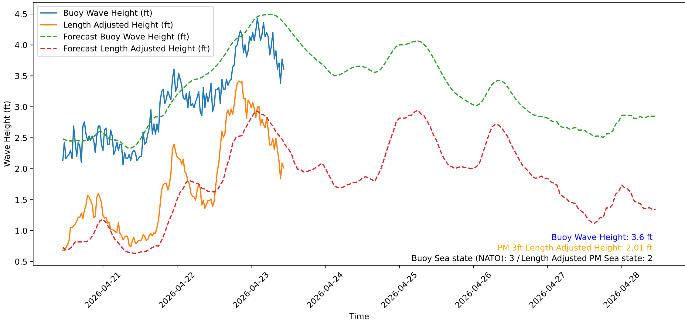
Wave Heights over Time for Oceanside Harbor at 2026-04-23 11:00:31
