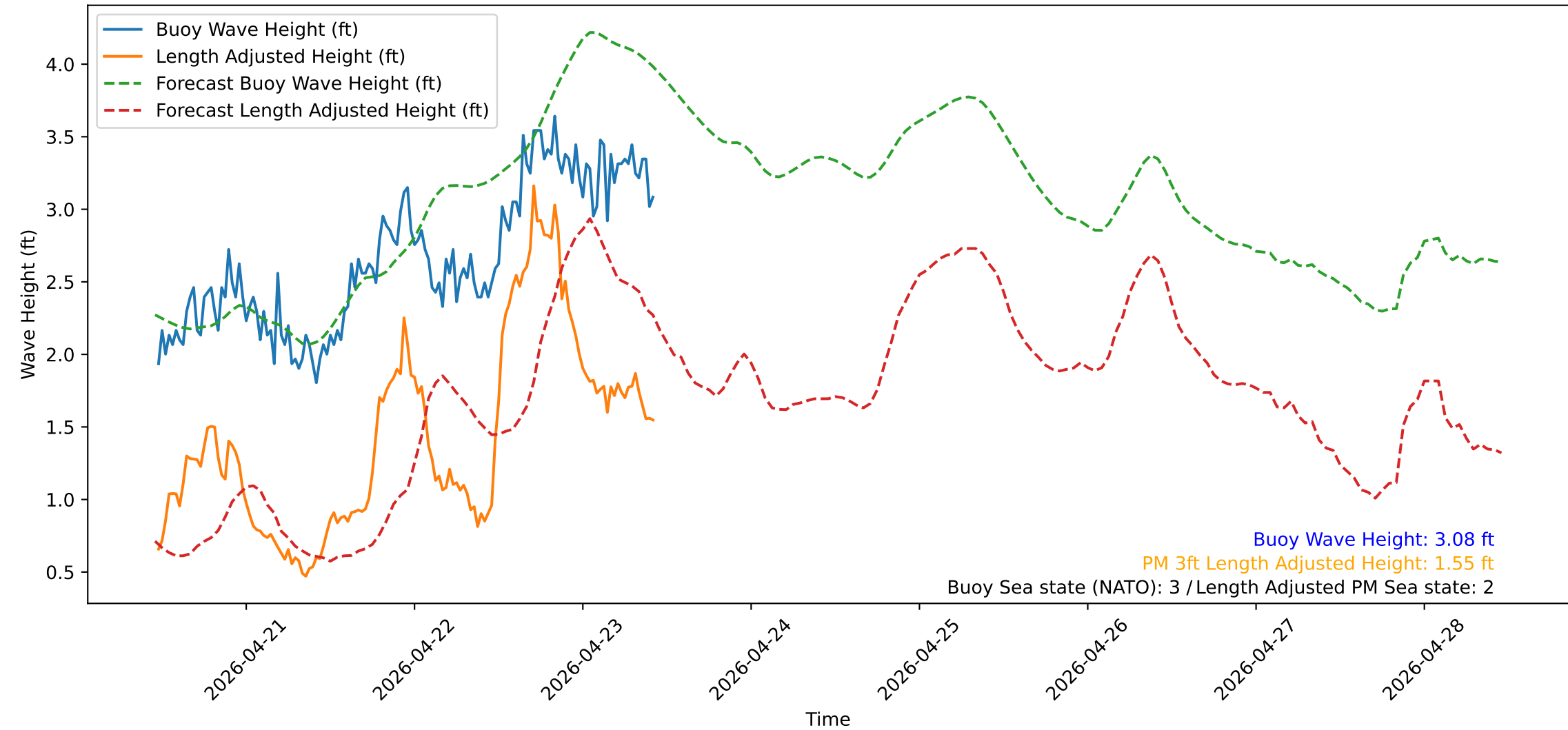
Wave Heights over Time for Red Beach at 2026-04-23 11:00:50
