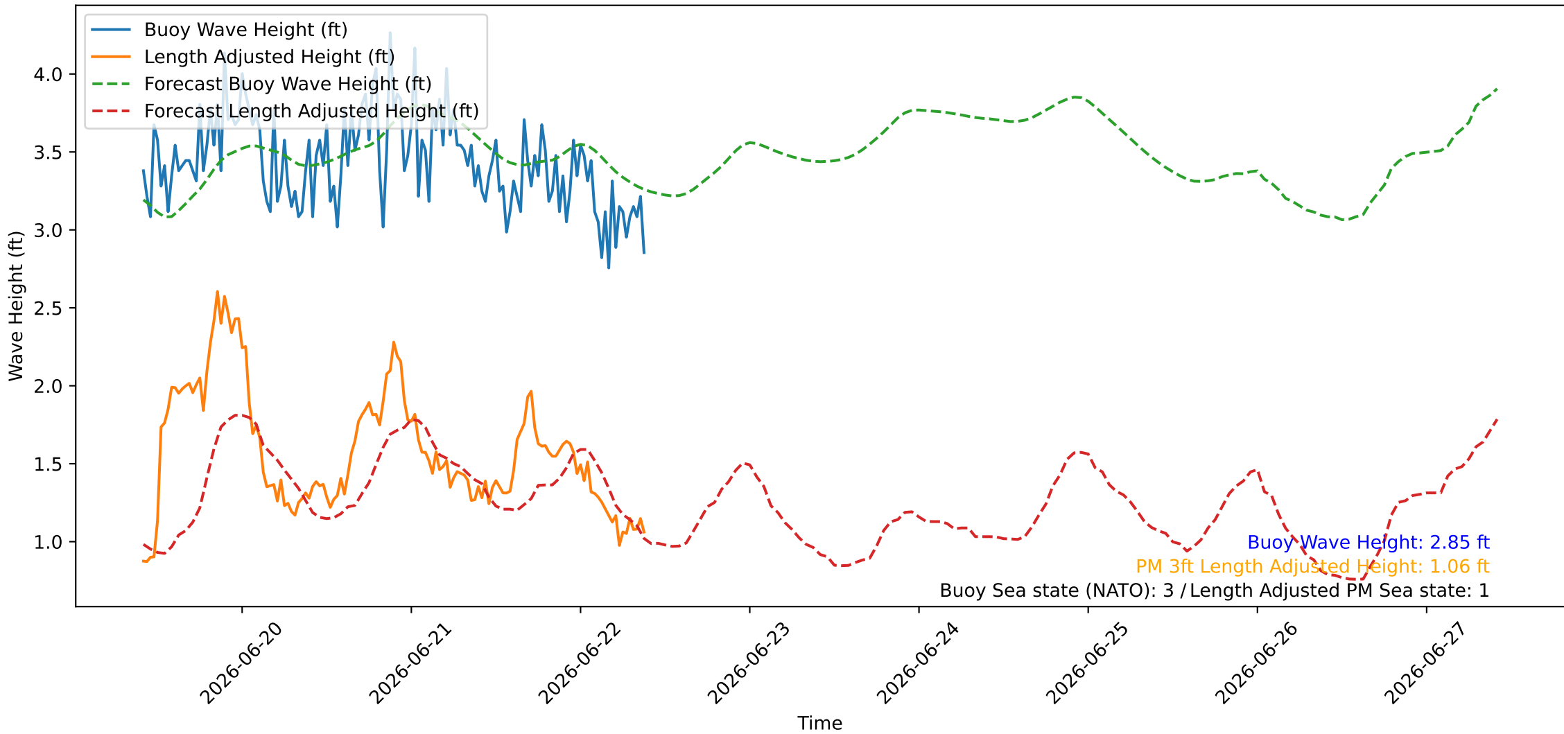
Wave Heights over Time for Oceanside Harbor at 2026-06-22 10:00:26
