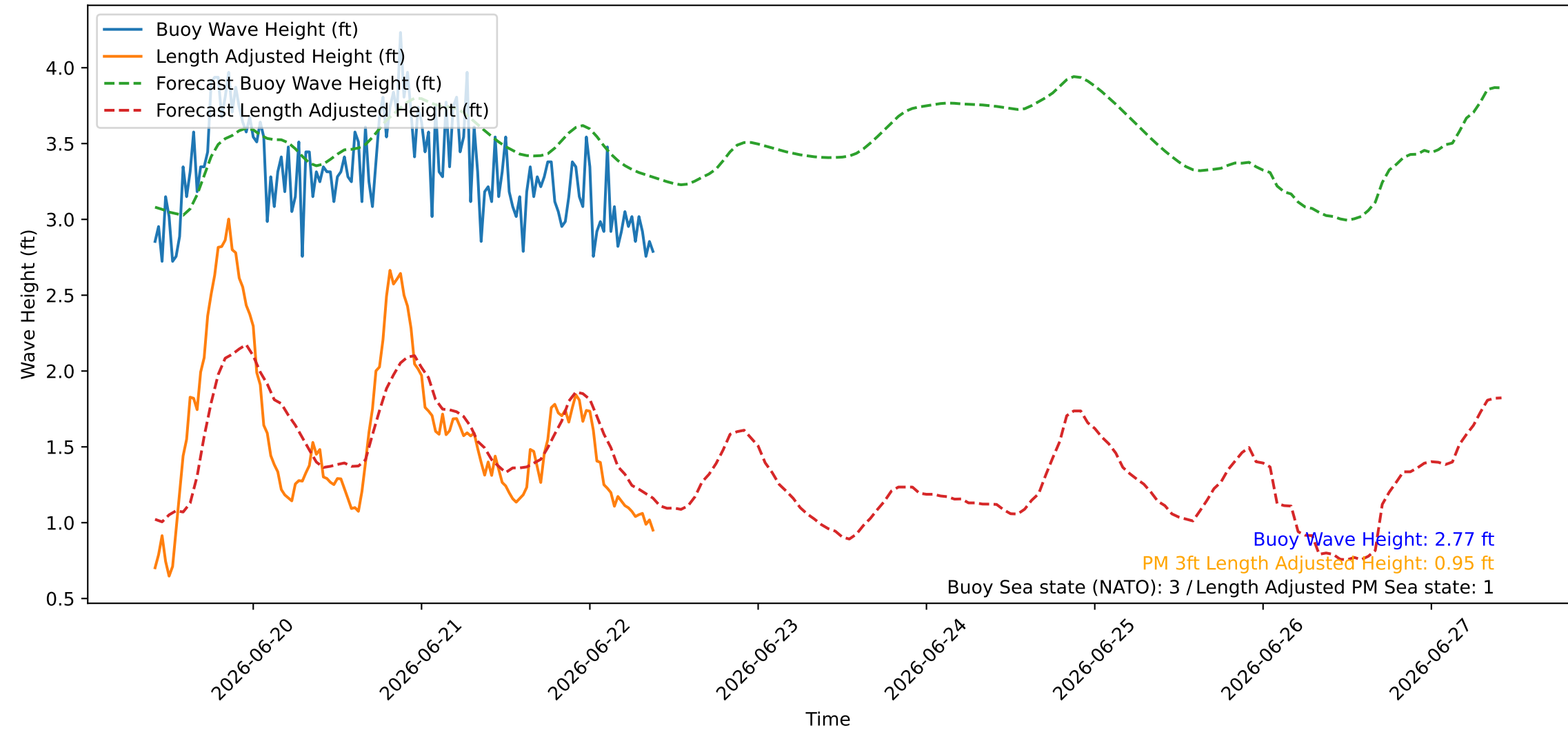
Wave Heights over Time for Green Beach at 2026-06-22 10:01:08
