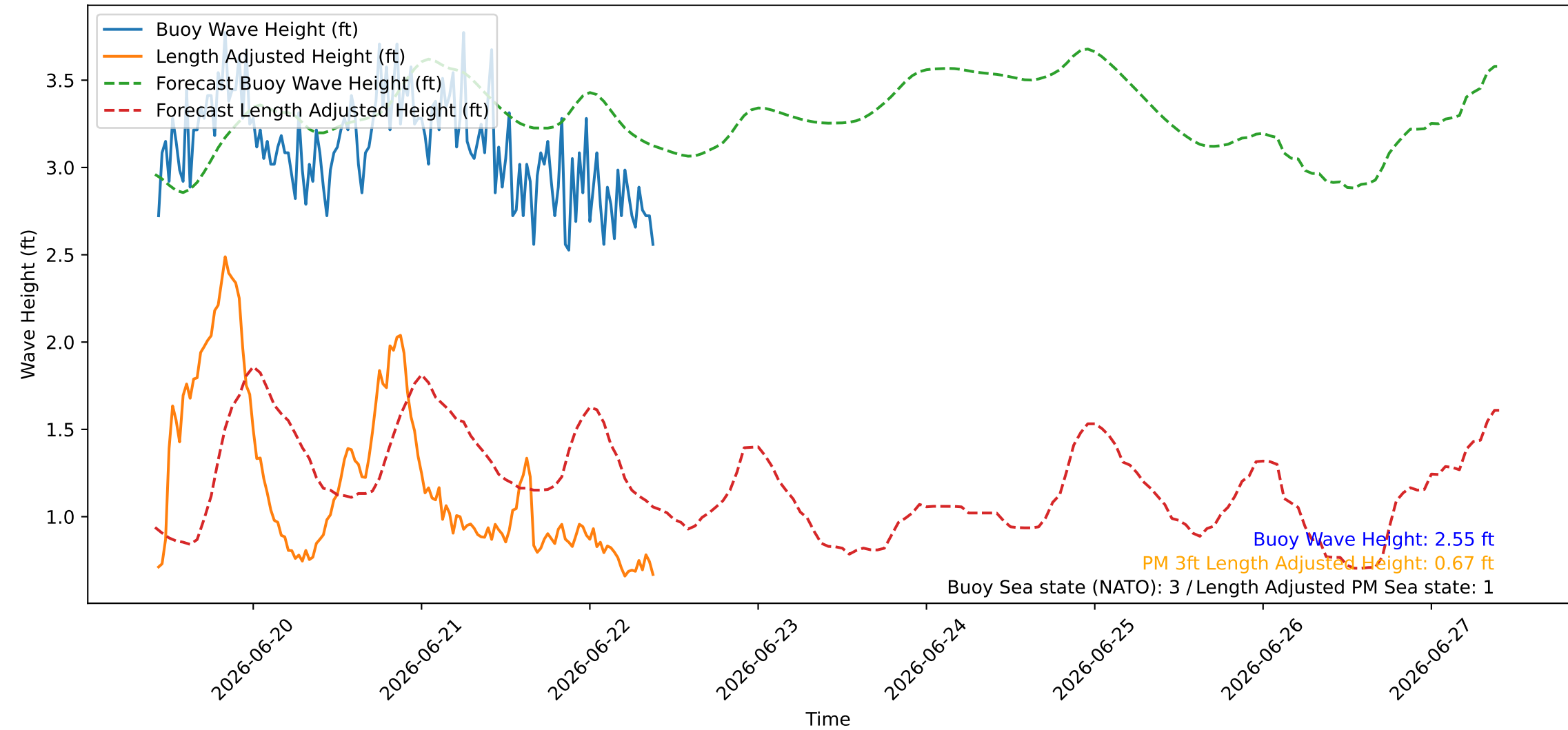
Wave Heights over Time for Red Beach at 2026-06-22 10:00:45
