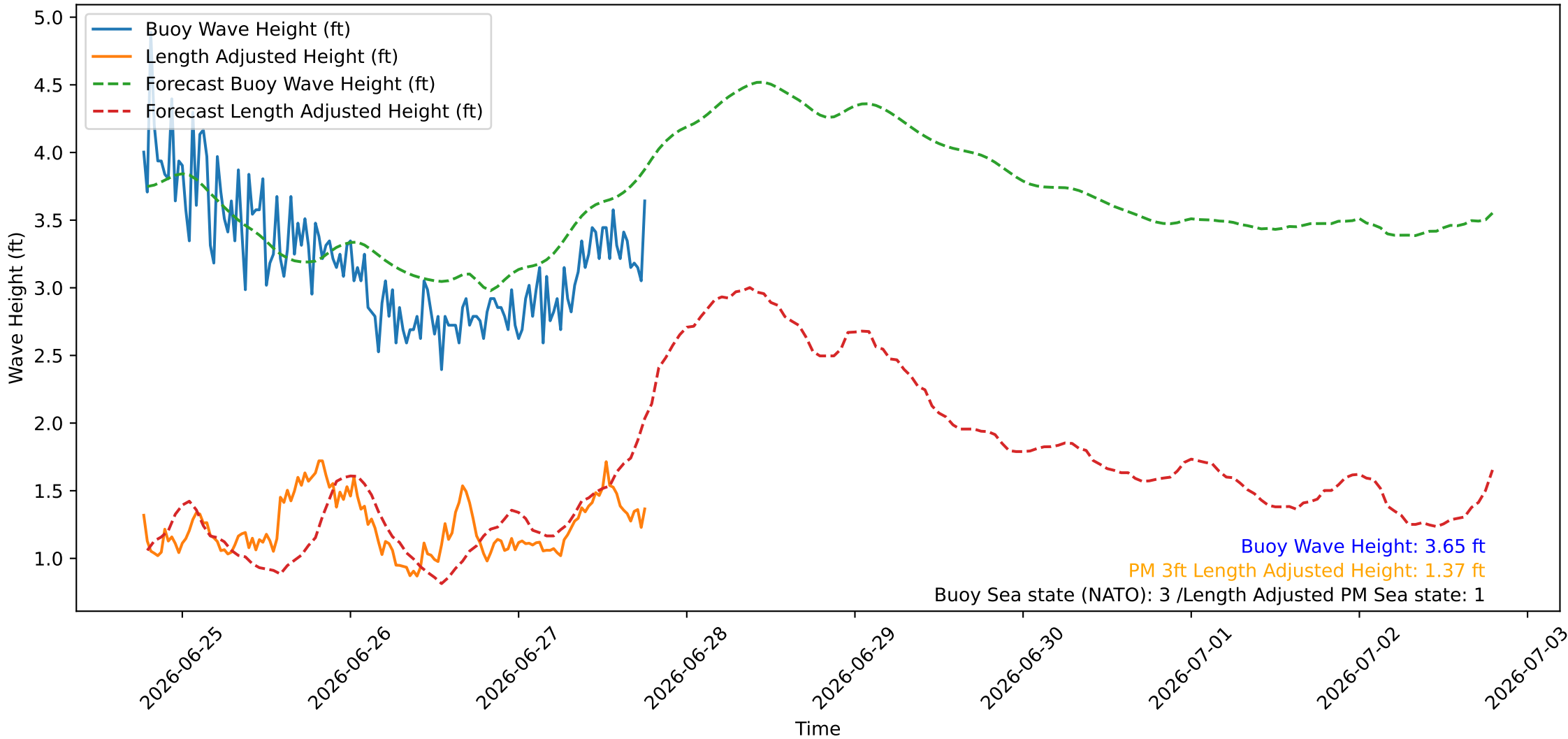
Wave Heights over Time for Oceanside Harbor at 2026-06-27 18:30:26
