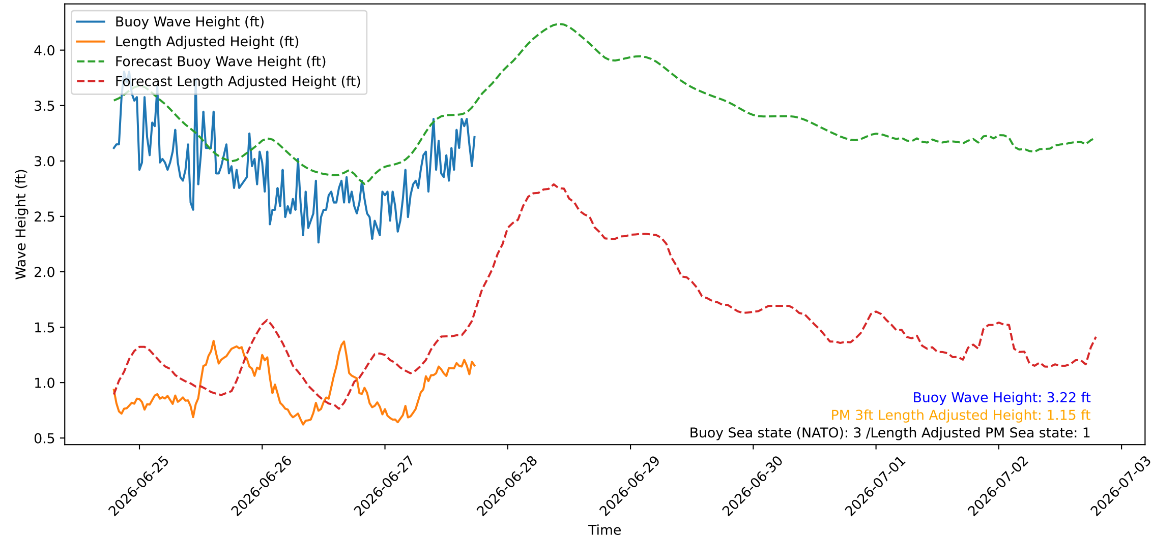
Wave Heights over Time for Red Beach at 2026-06-27 18:30:45
