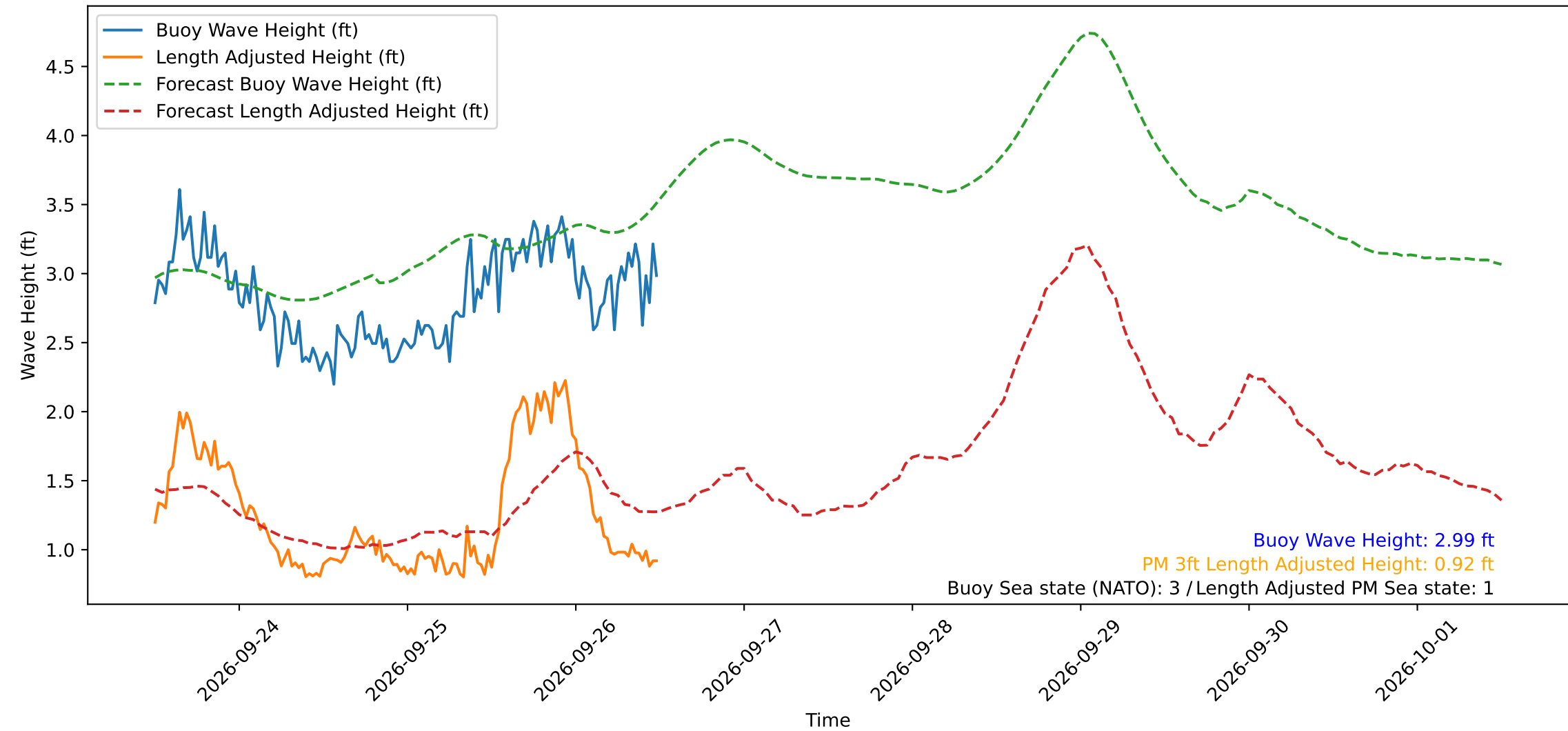
Wave Heights over Time for Oceanside Harbor at 2026-09-26 12:10:29
