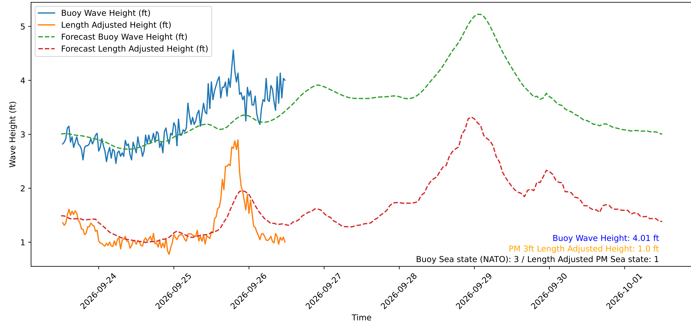
Wave Heights over Time for Green Beach at 2026-09-26 12:11:12
