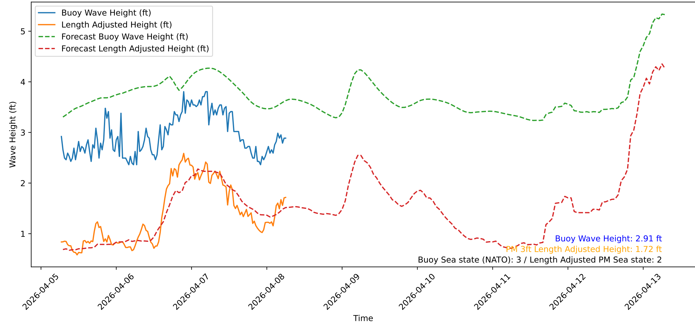
Wave Heights over Time for Green Beach at 2026-04-08 06:41:11
