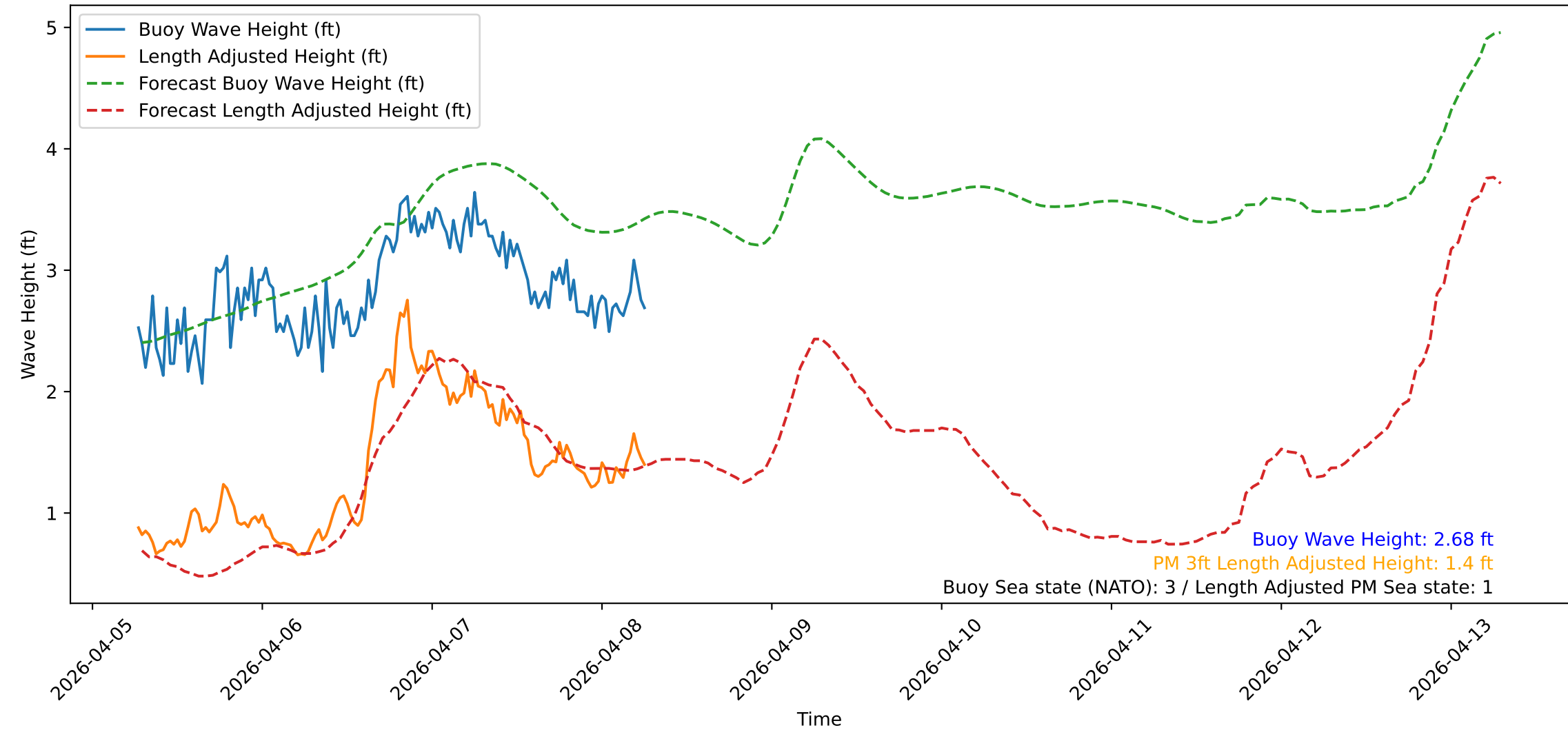
Wave Heights over Time for Oceanside Harbor at 2026-04-08 06:40:32
