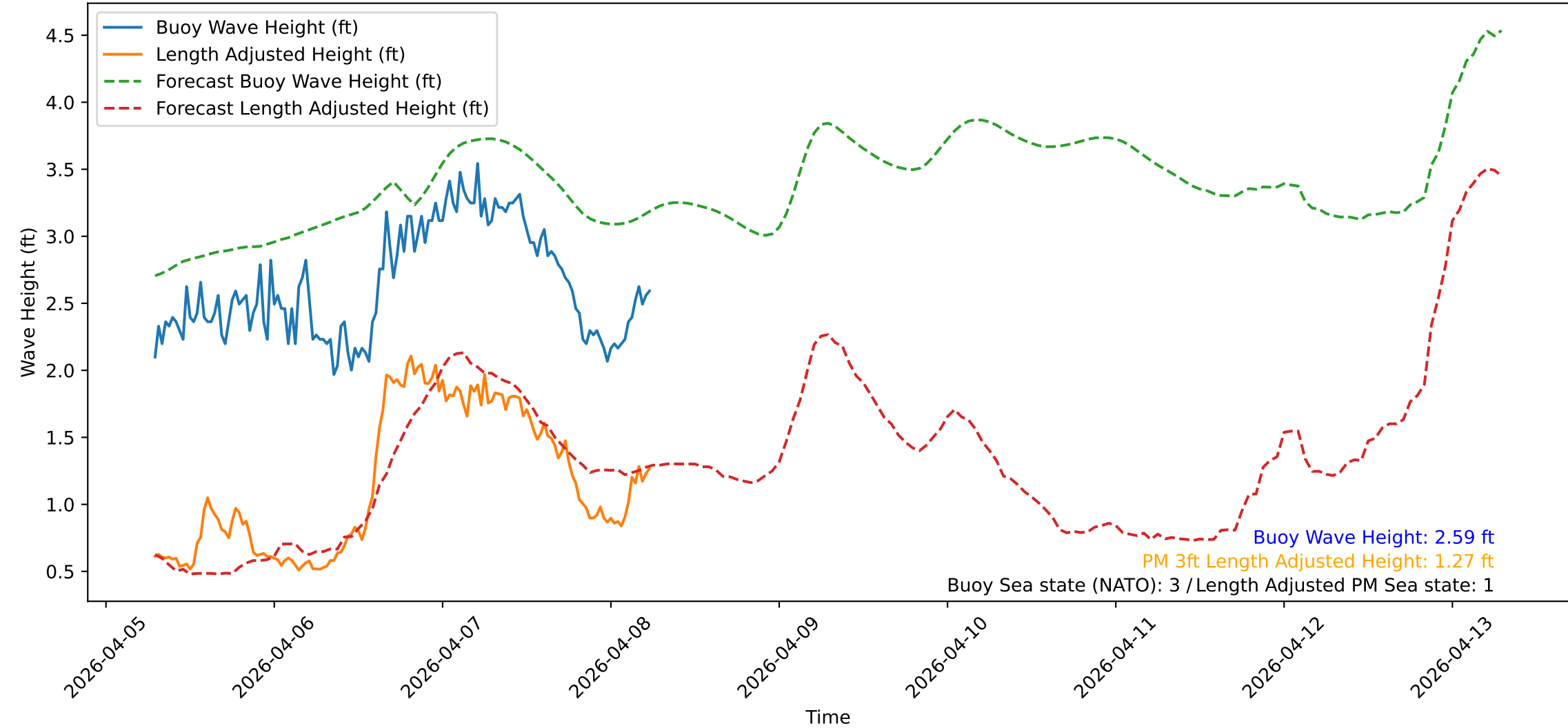
Wave Heights over Time for Red Beach at 2026-04-08 06:40:48
