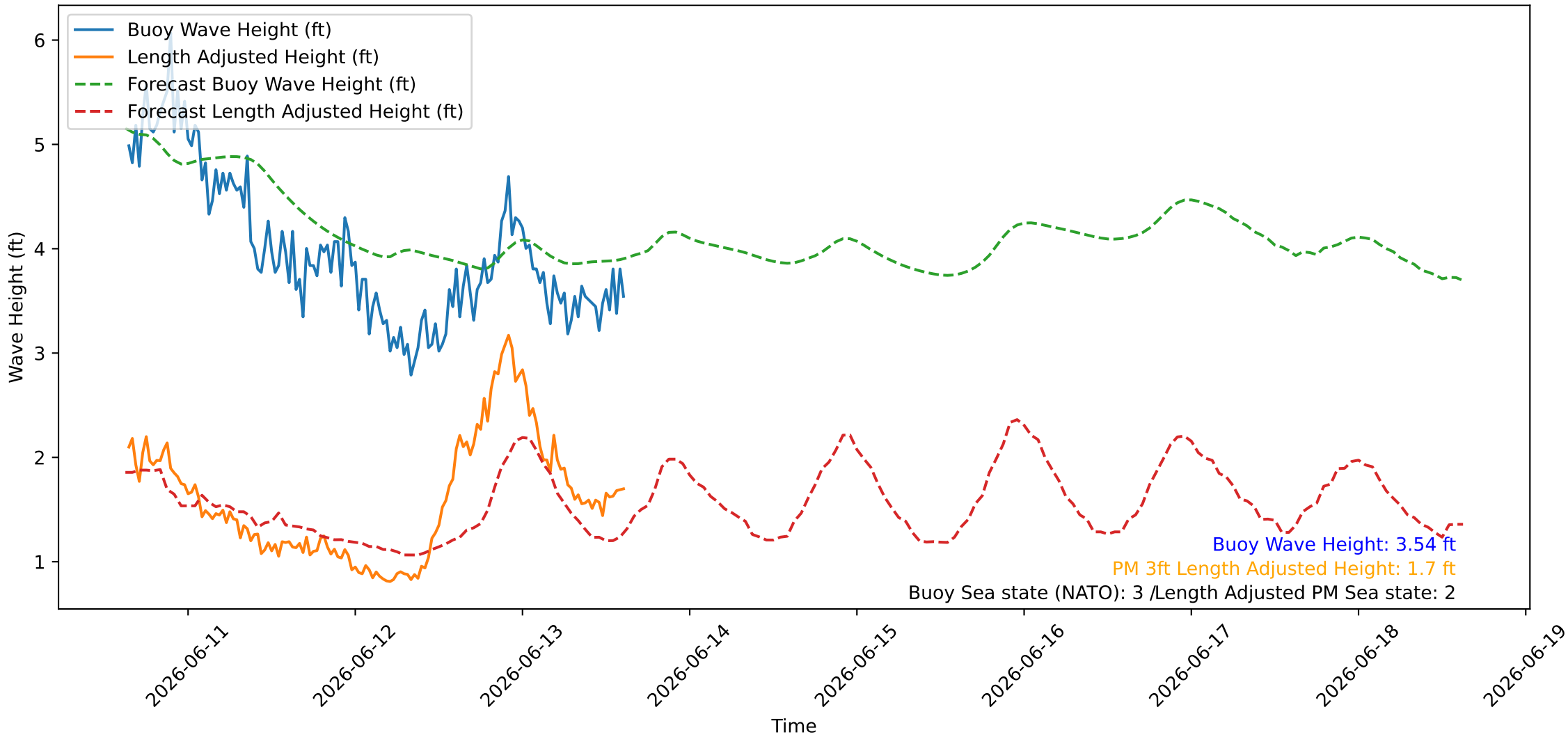
Wave Heights over Time for Oceanside Harbor at 2026-06-13 15:20:26
