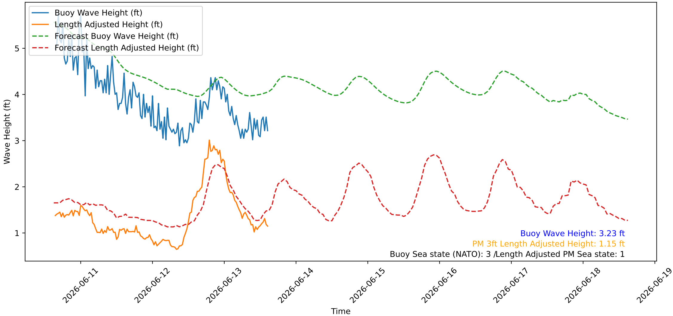
Wave Heights over Time for Green Beach at 2026-06-13 15:21:10
