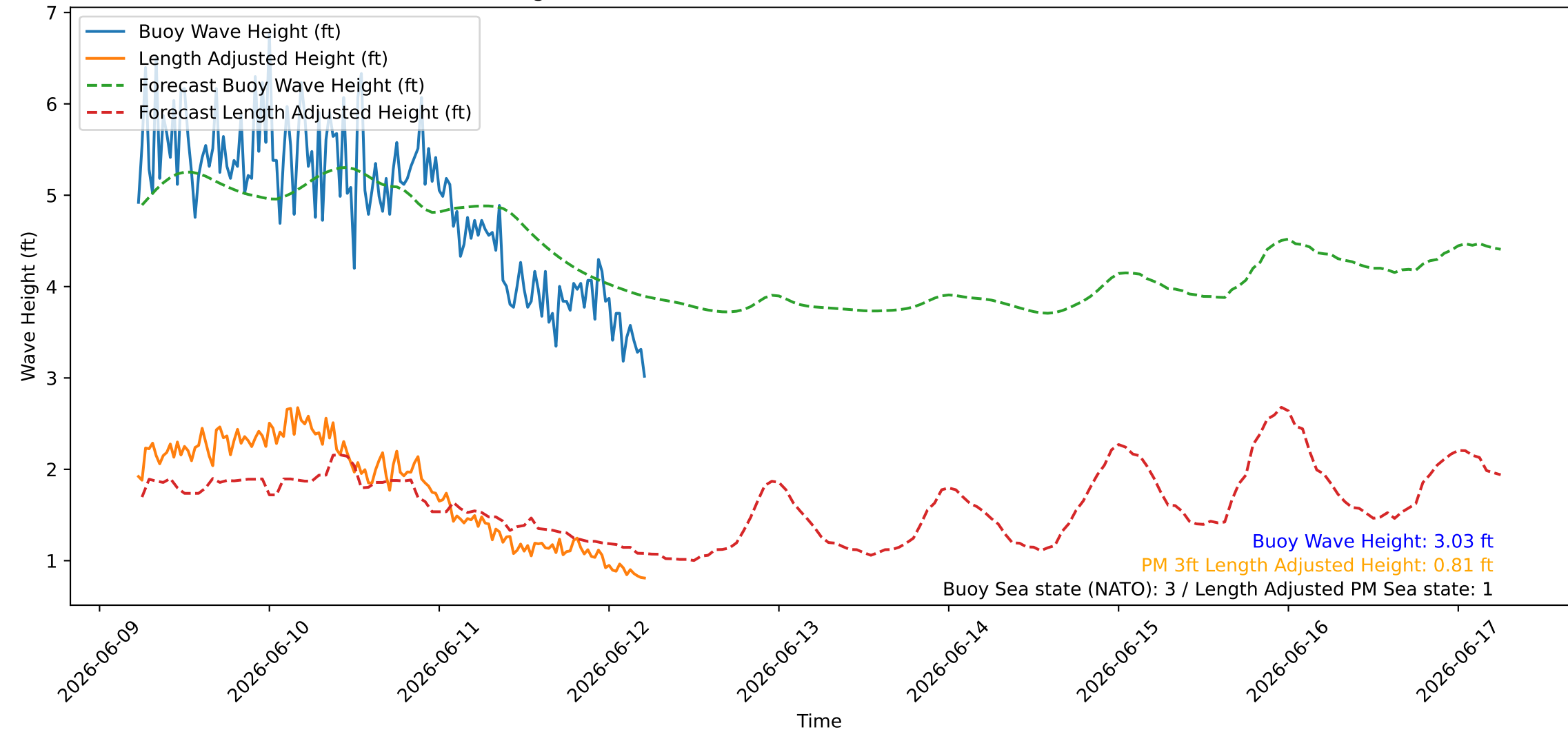
Wave Heights over Time for Oceanside Harbor at 2026-06-12 05:40:26
