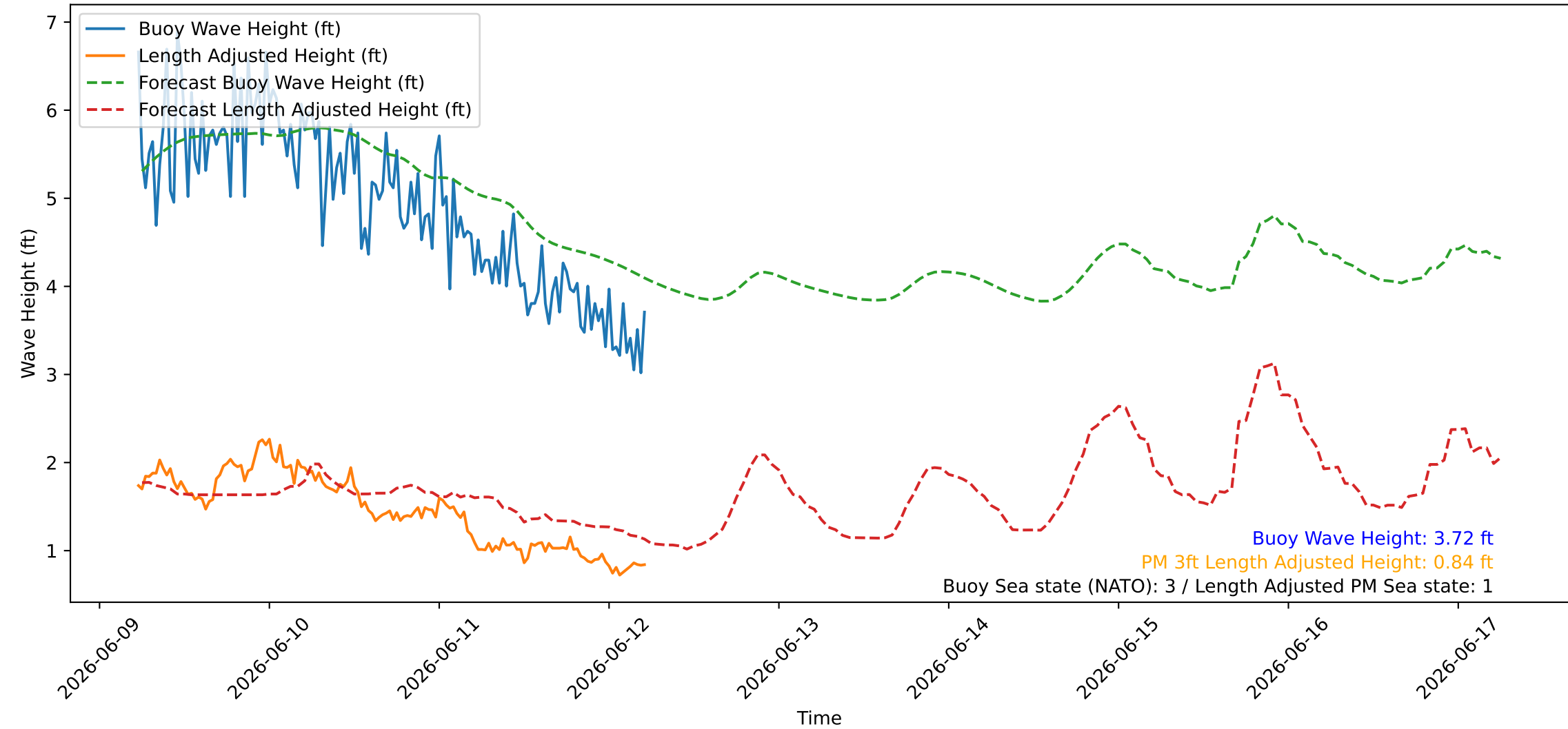
Wave Heights over Time for Green Beach at 2026-06-12 05:41:08
