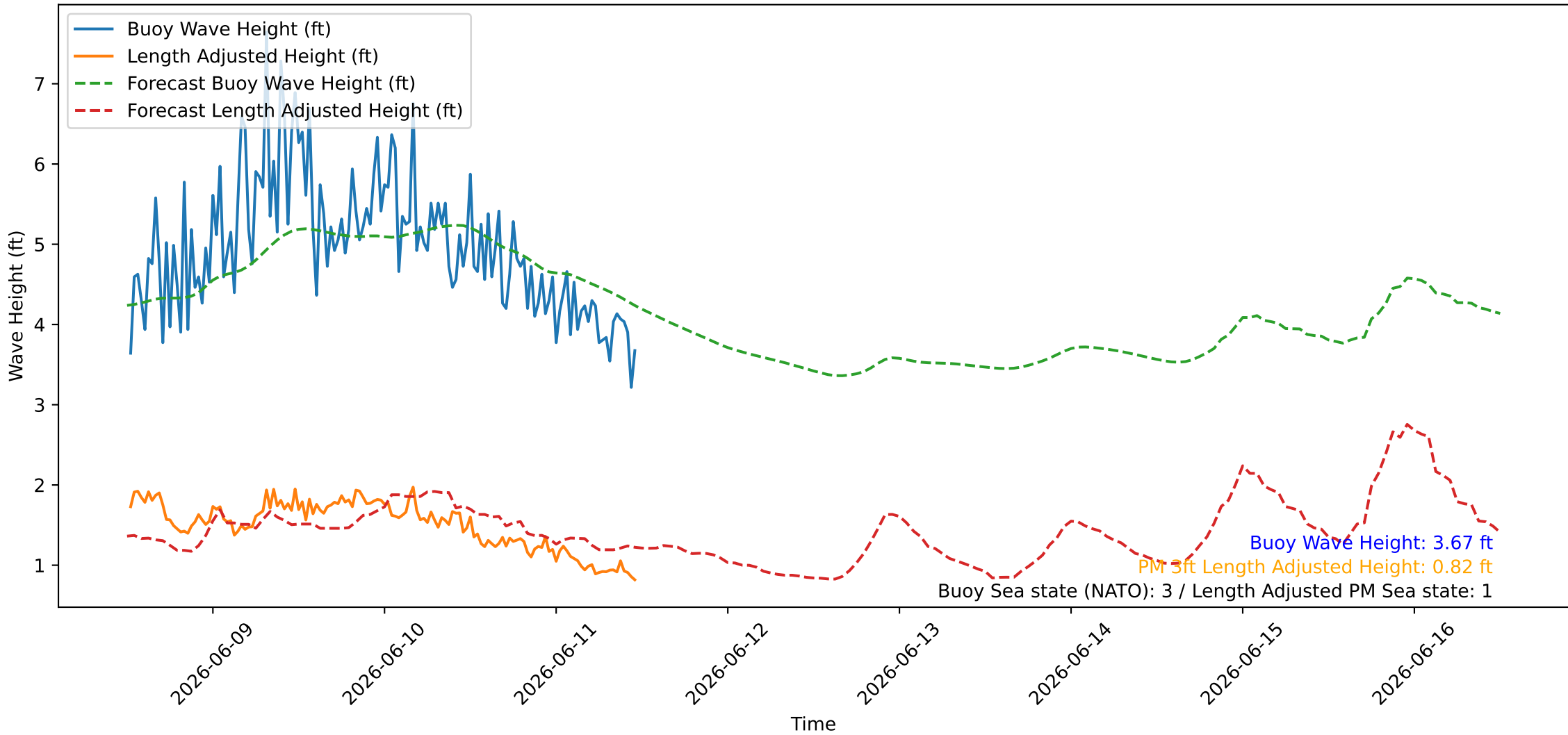
Wave Heights over Time for Red Beach at 2026-06-11 12:00:47
