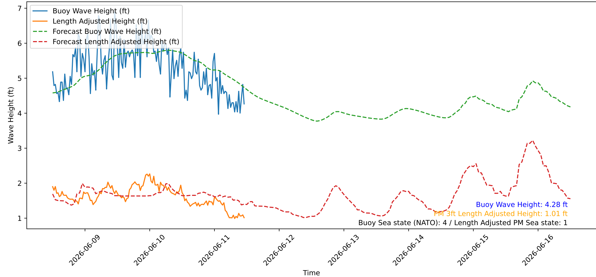
Wave Heights over Time for Green Beach at 2026-06-11 12:01:09
