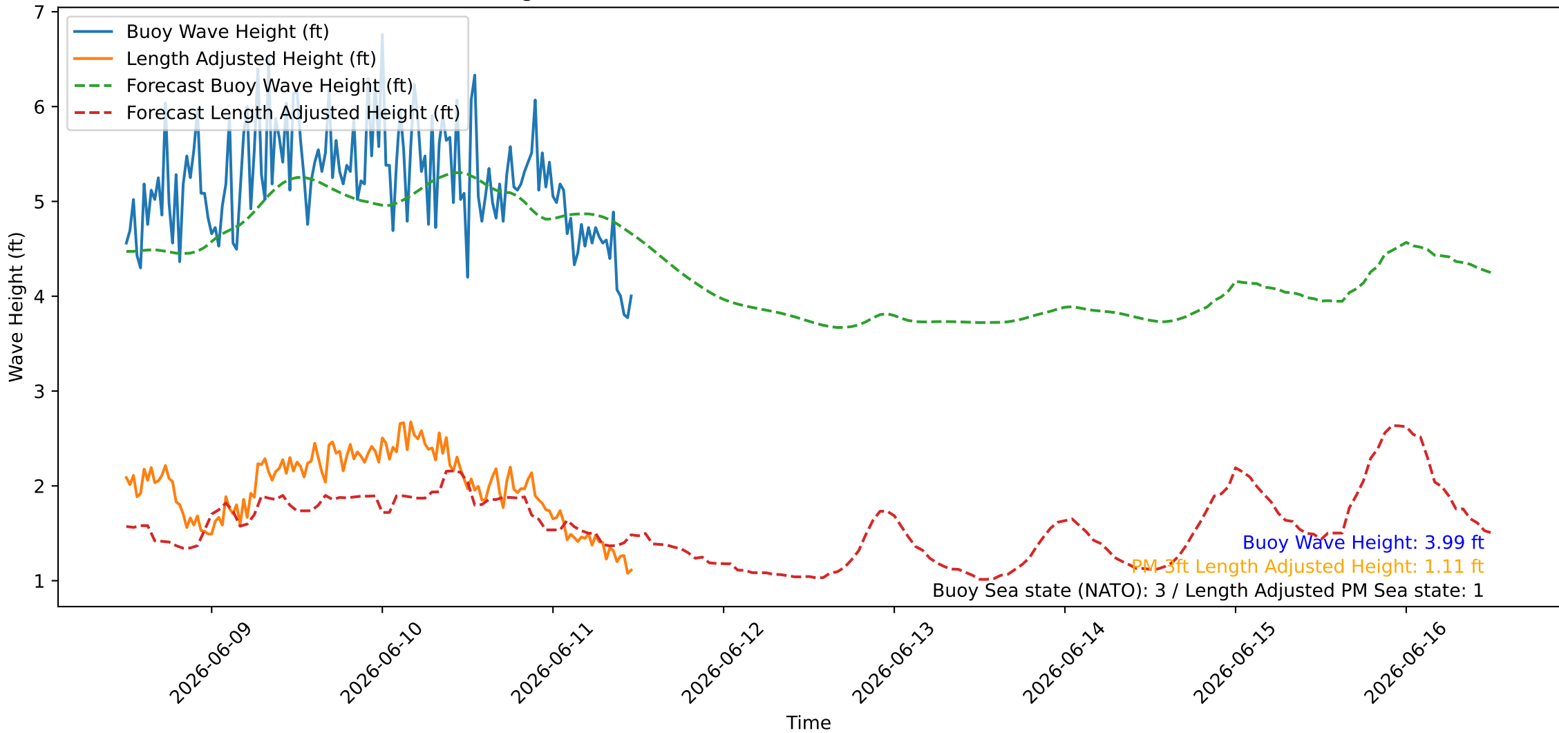
Wave Heights over Time for Oceanside Harbor at 2026-06-11 12:00:27
