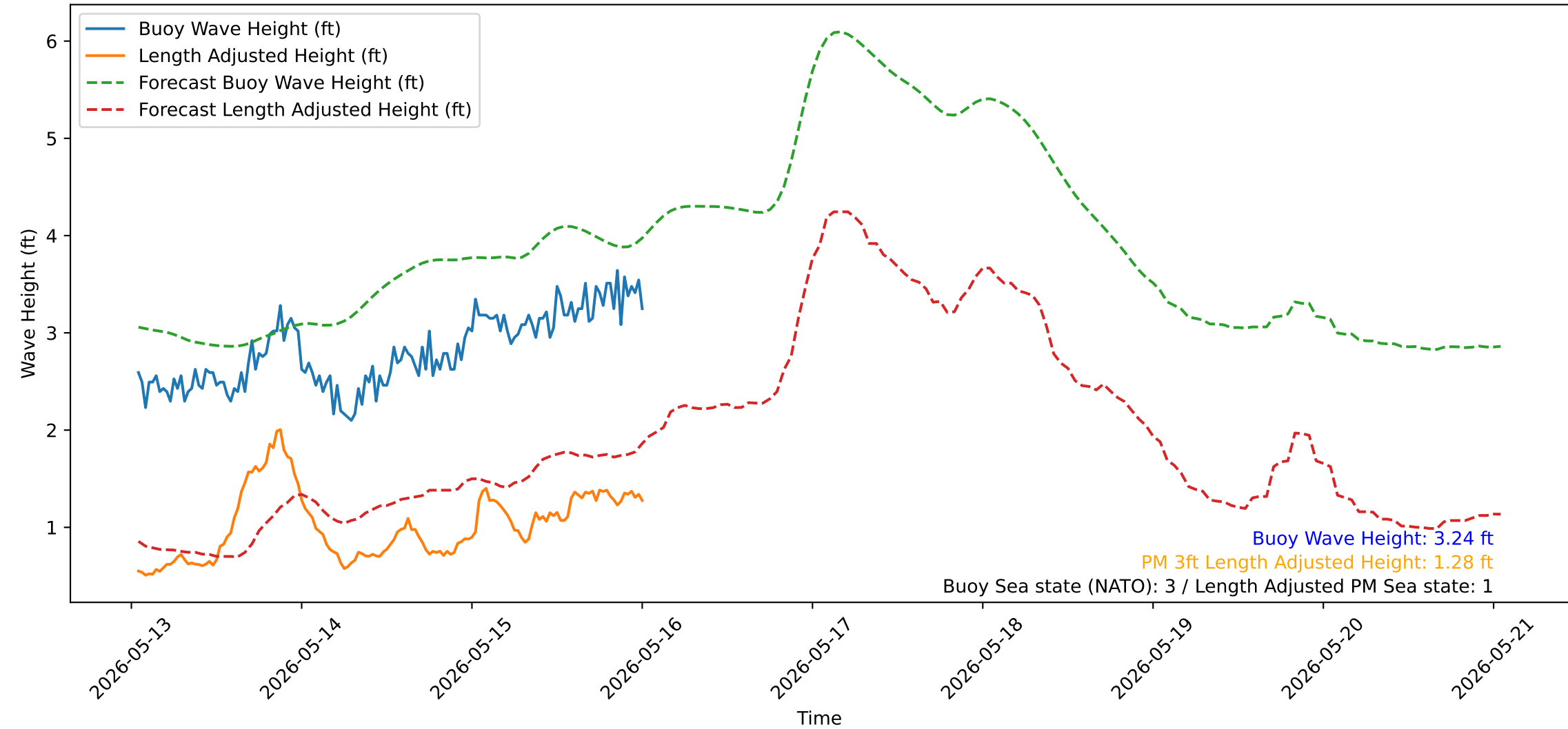
Wave Heights over Time for Green Beach at 2026-05-16 01:01:13
