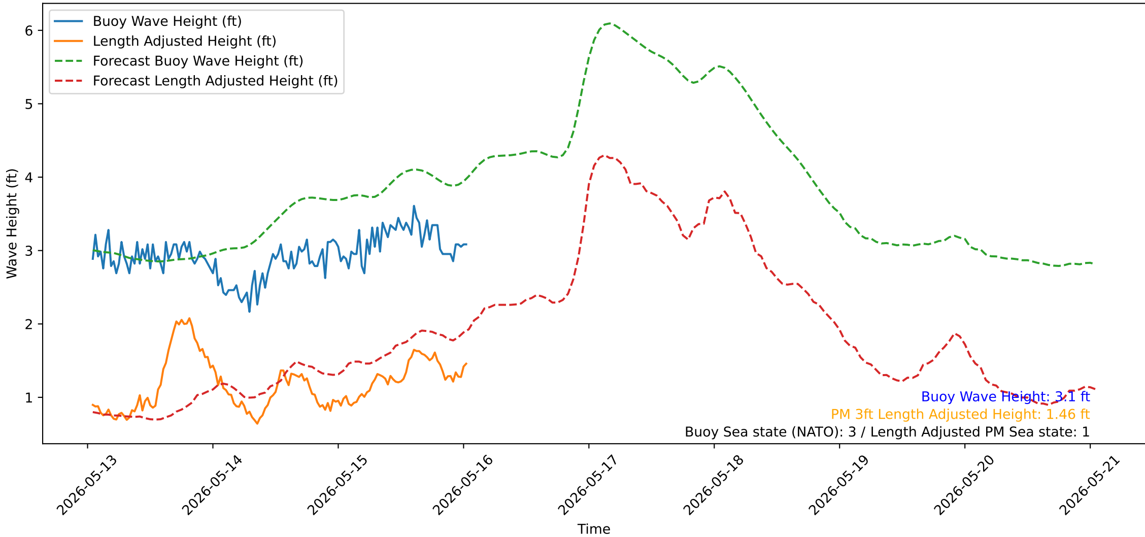
Wave Heights over Time for Oceanside Harbor at 2026-05-16 01:00:31
