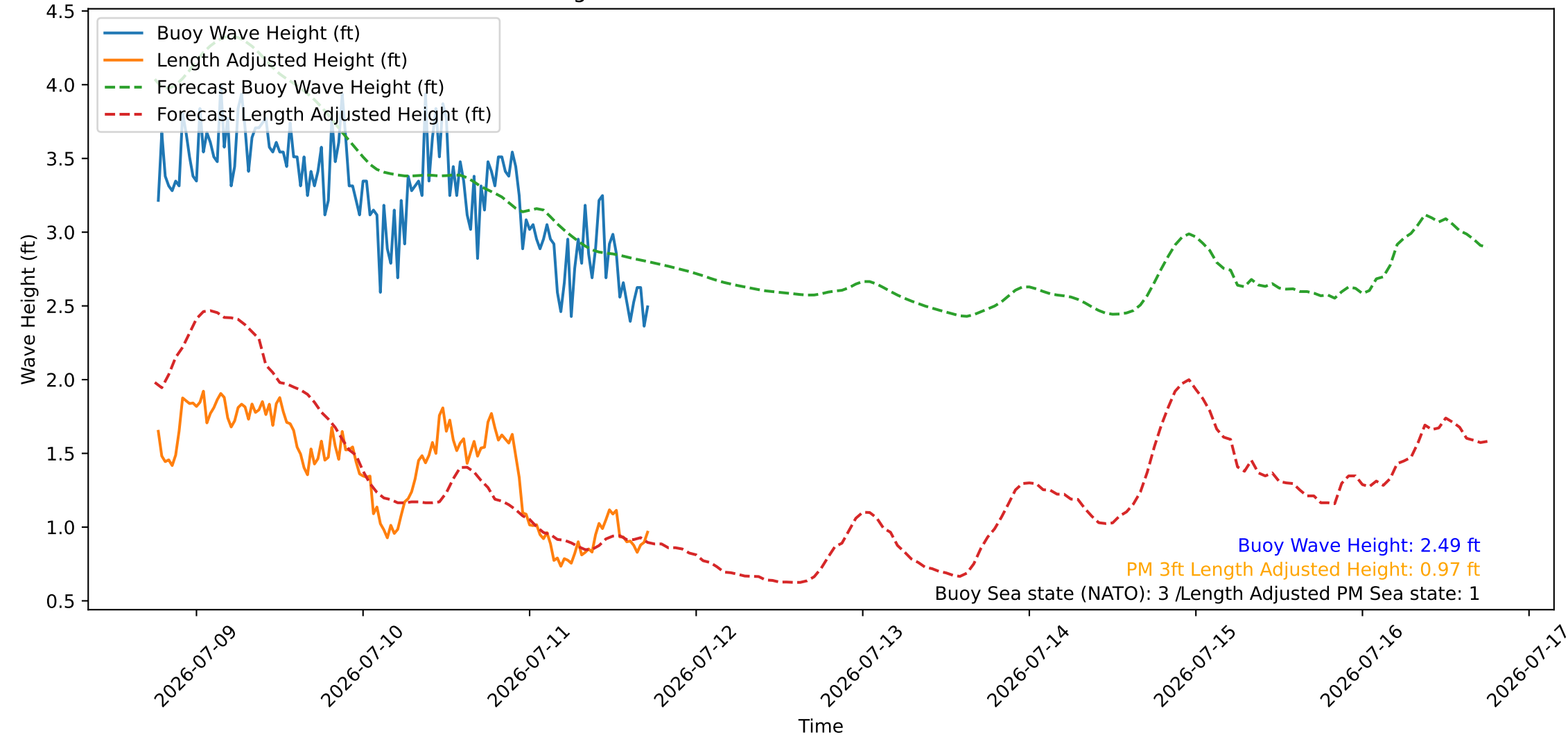
Wave Heights over Time for Red Beach at 2026-07-11 18:00:45
