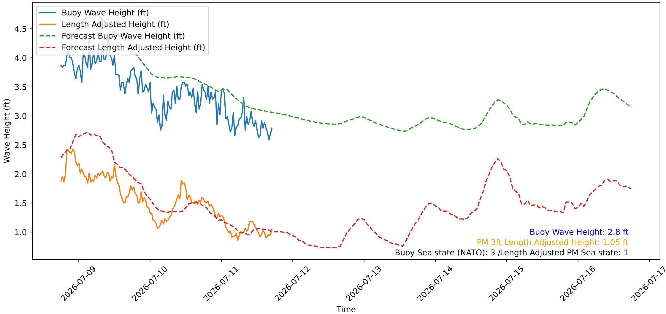
Wave Heights over Time for Green Beach at 2026-07-11 18:01:08
