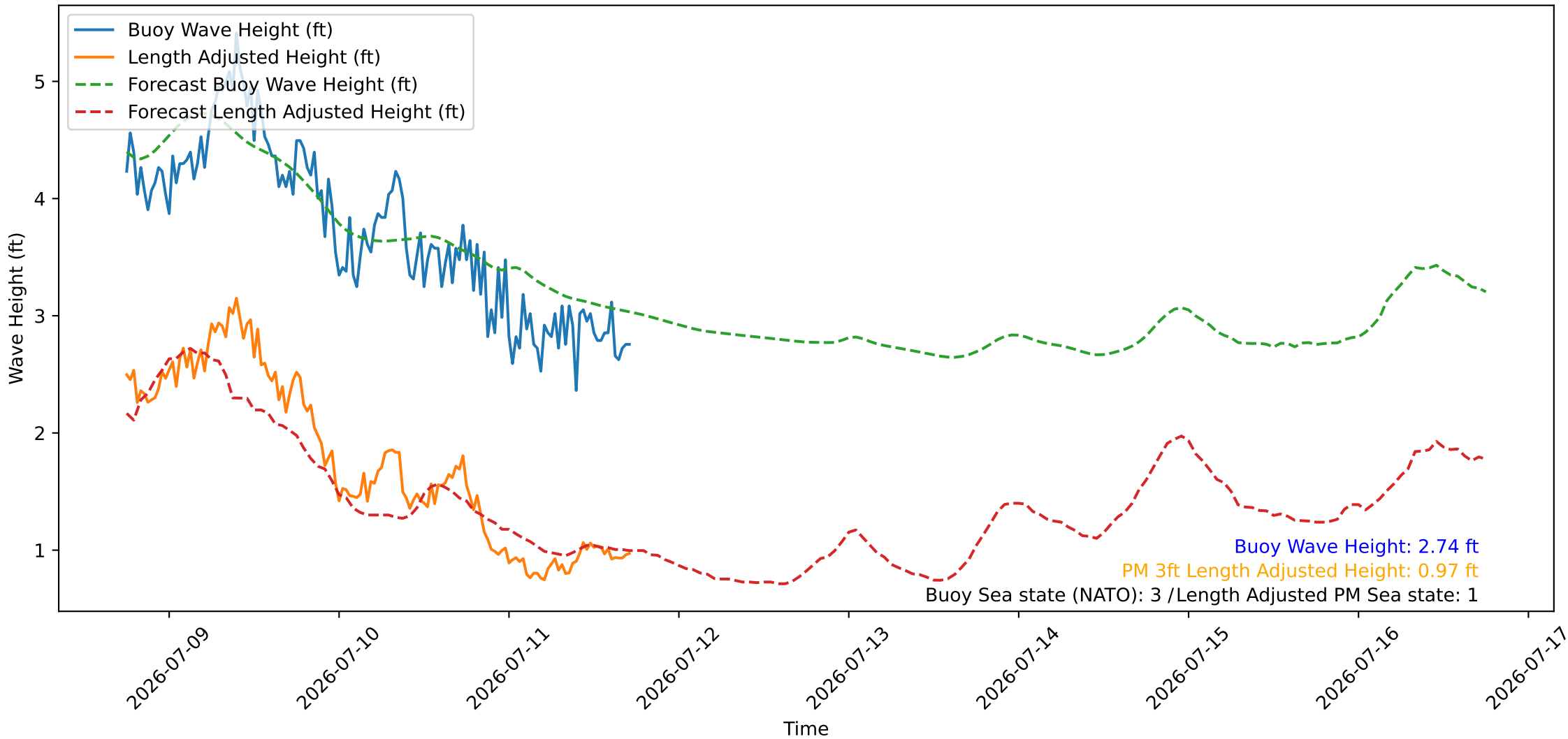
Wave Heights over Time for Oceanside Harbor at 2026-07-11 18:00:26
