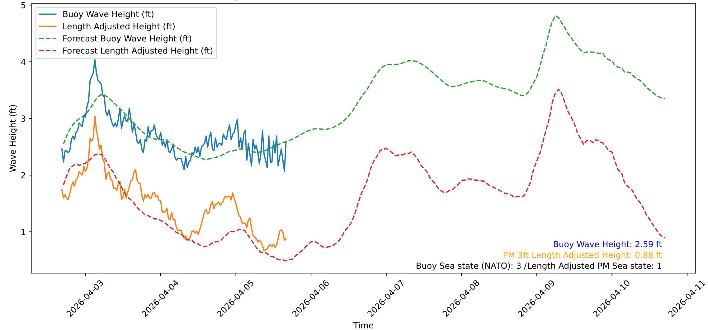
Wave Heights over Time for Oceanside Harbor at 2026-04-05 16:40:34
