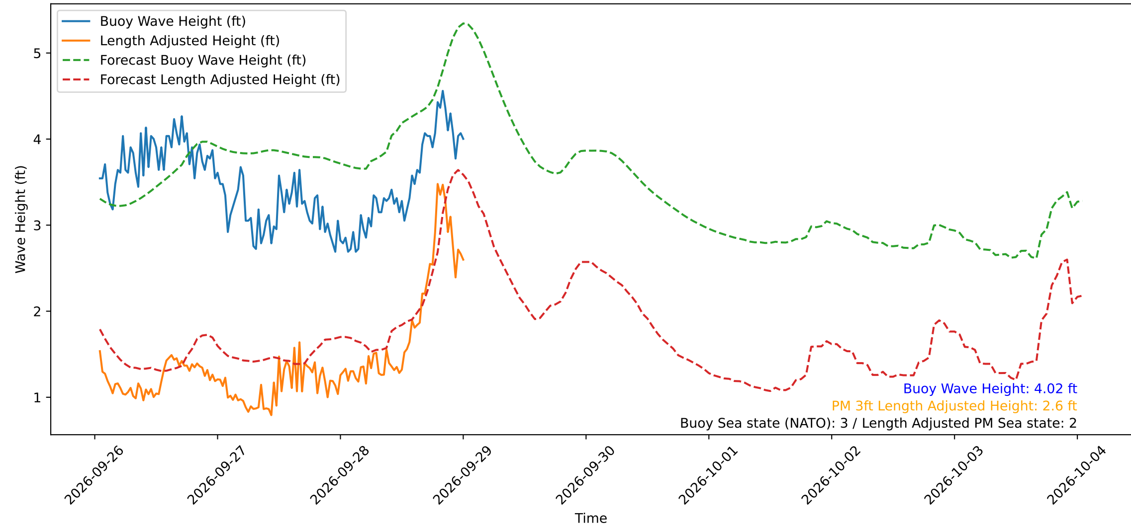
Wave Heights over Time for Green Beach at 2026-09-29 00:51:15
