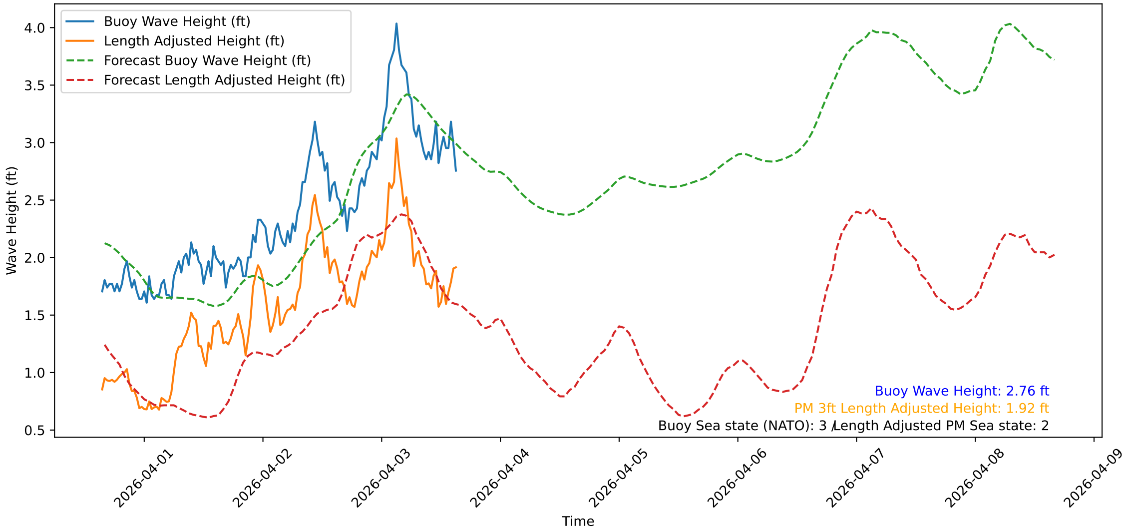
Wave Heights over Time for Oceanside Harbor at 2026-04-03 15:40:32
