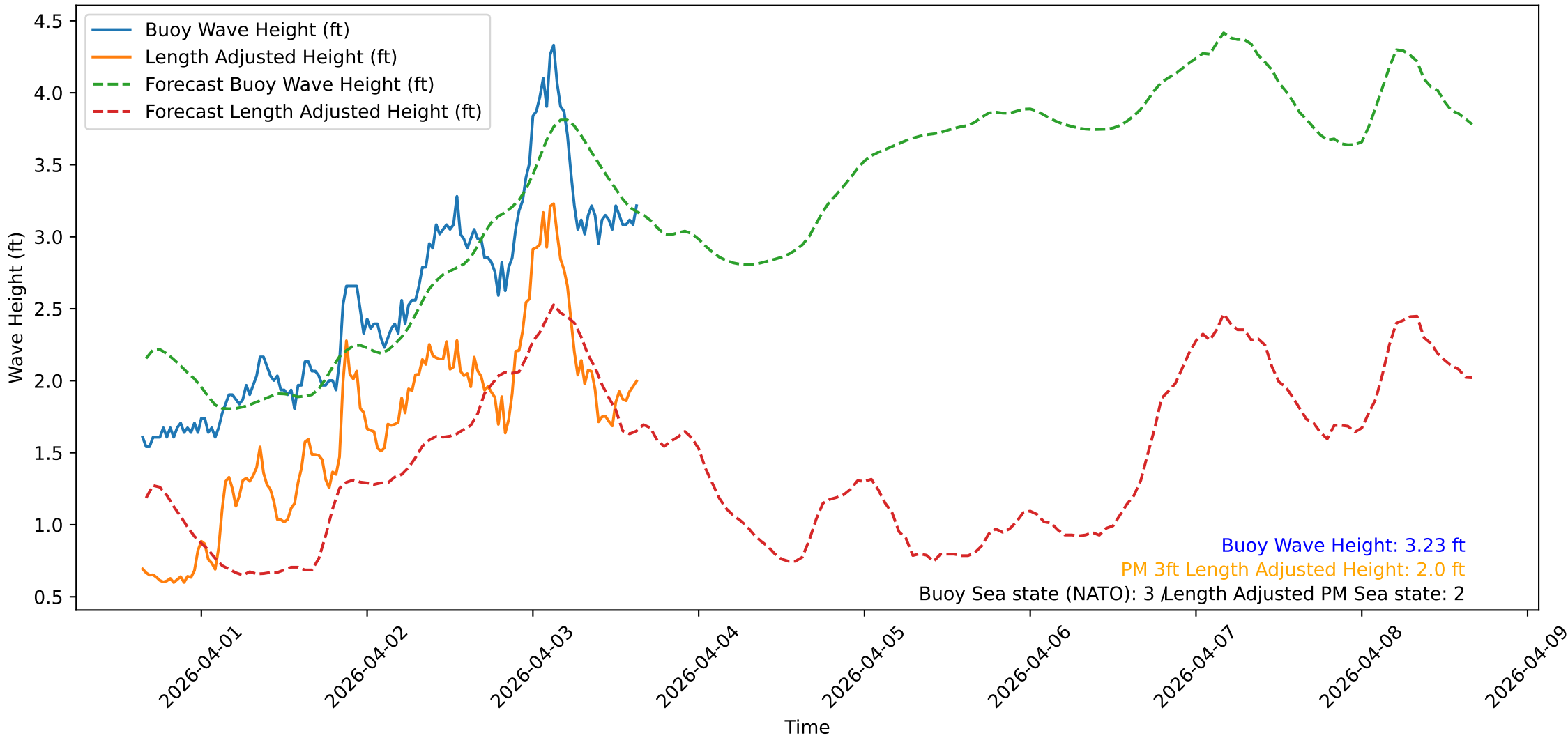
Wave Heights over Time for Green Beach at 2026-04-03 15:41:11
