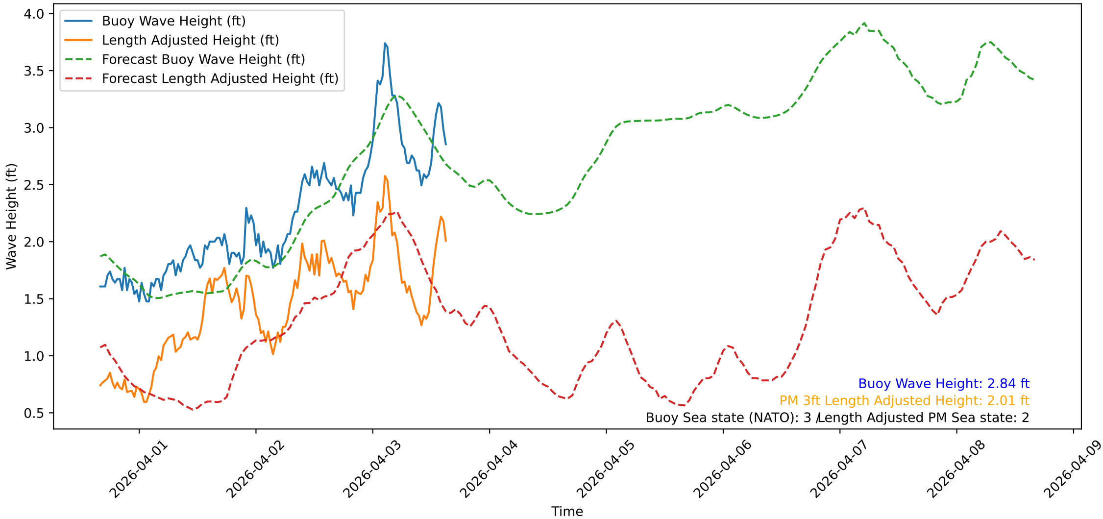
Wave Heights over Time for Red Beach at 2026-04-03 15:40:49
