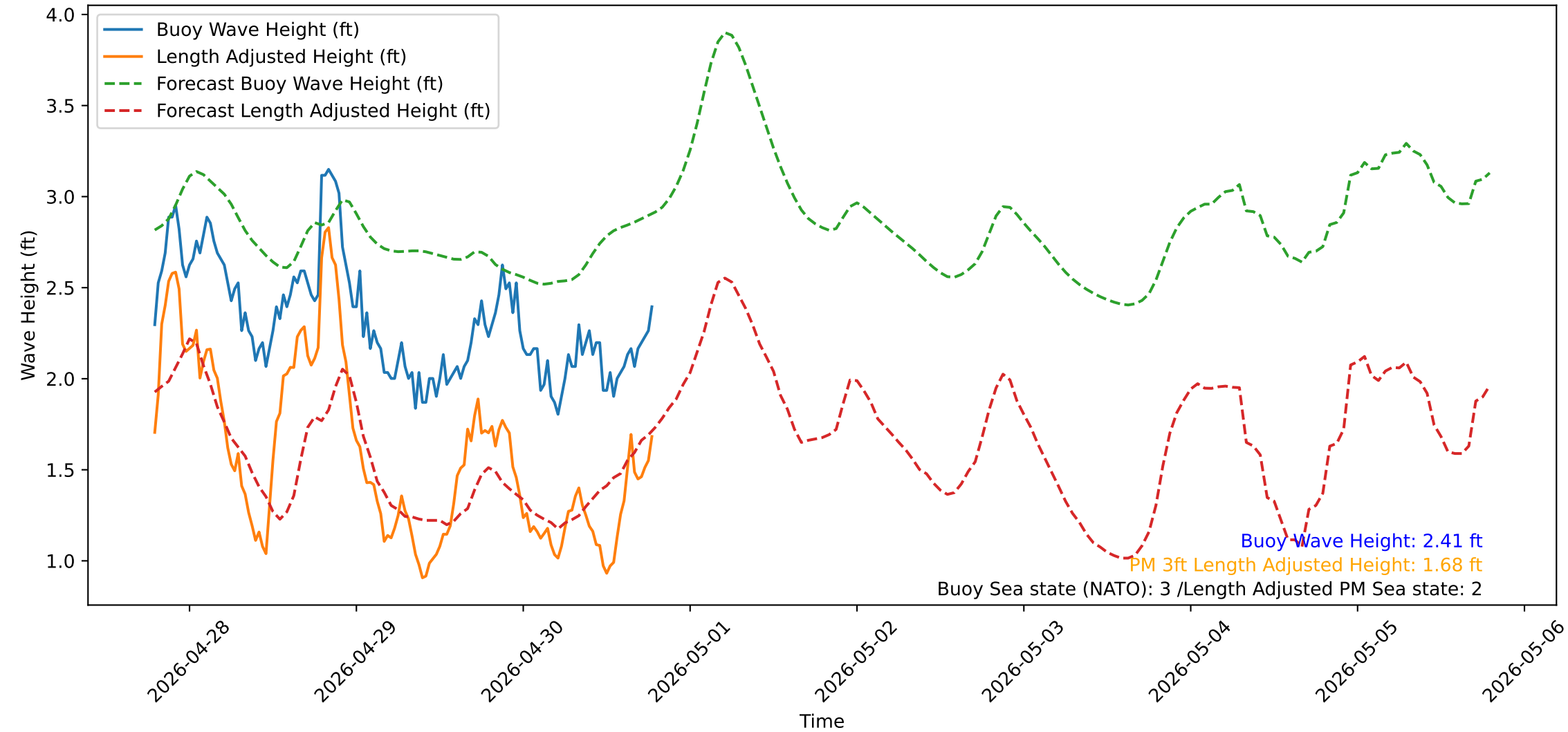
Wave Heights over Time for Green Beach at 2026-04-30 19:11:12
