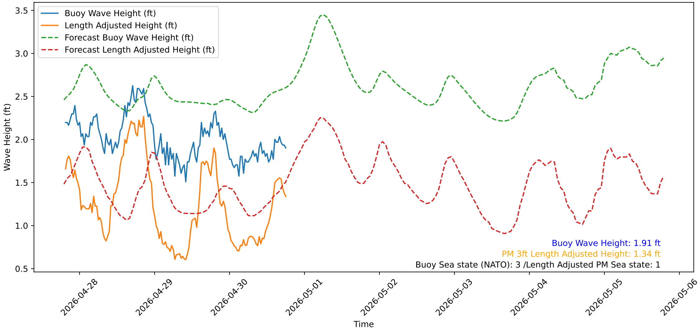
Wave Heights over Time for Red Beach at 2026-04-30 19:10:50
