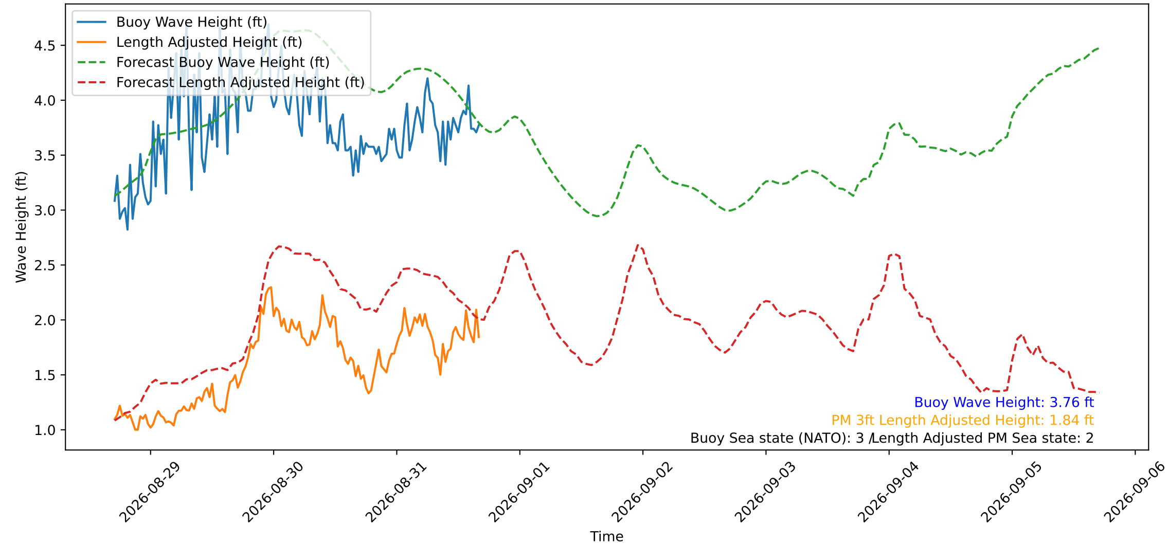
Wave Heights over Time for Red Beach at 2026-08-31 16:40:49
