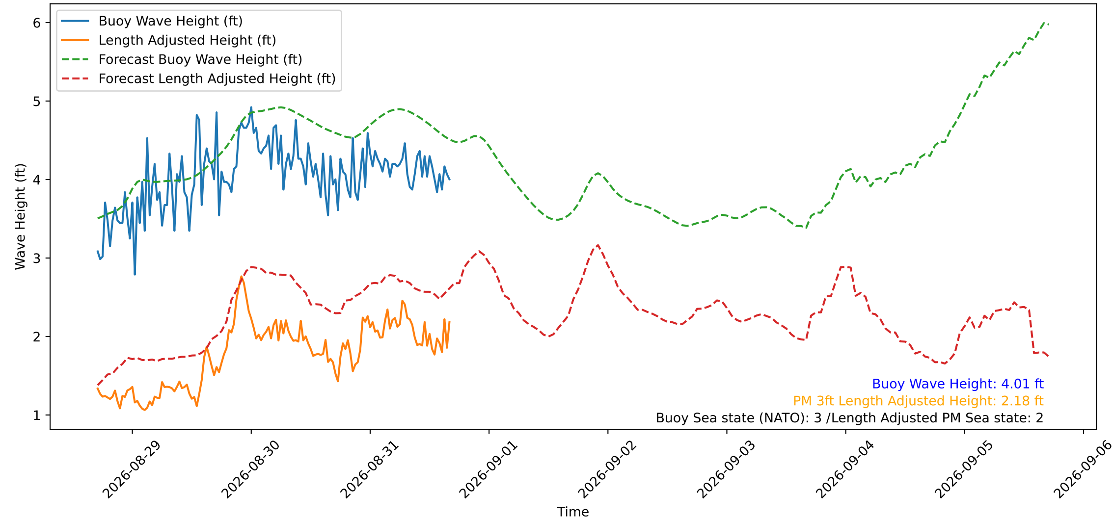
Wave Heights over Time for Green Beach at 2026-08-31 16:41:12
