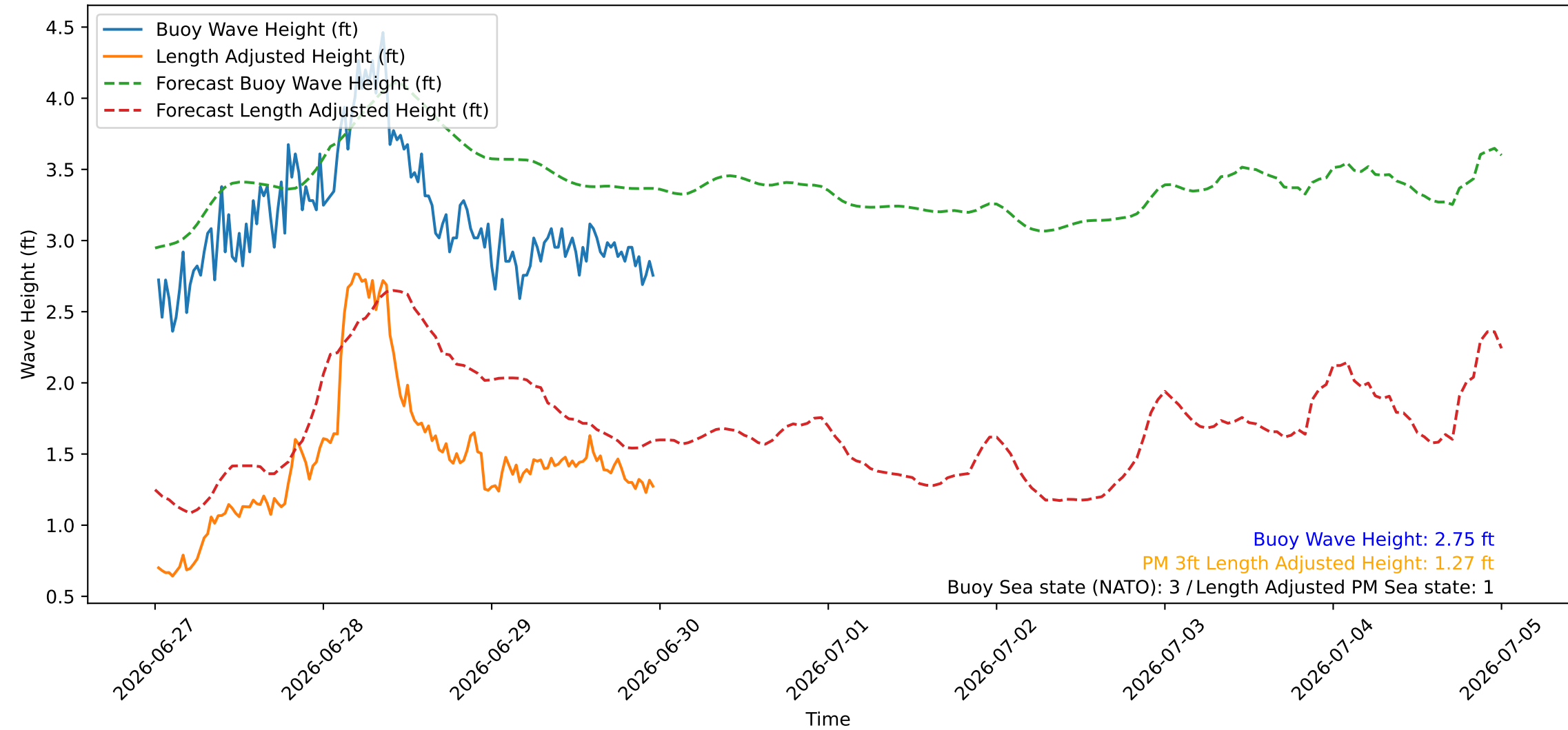
Wave Heights over Time for Red Beach at 2026-06-30 00:00:44
