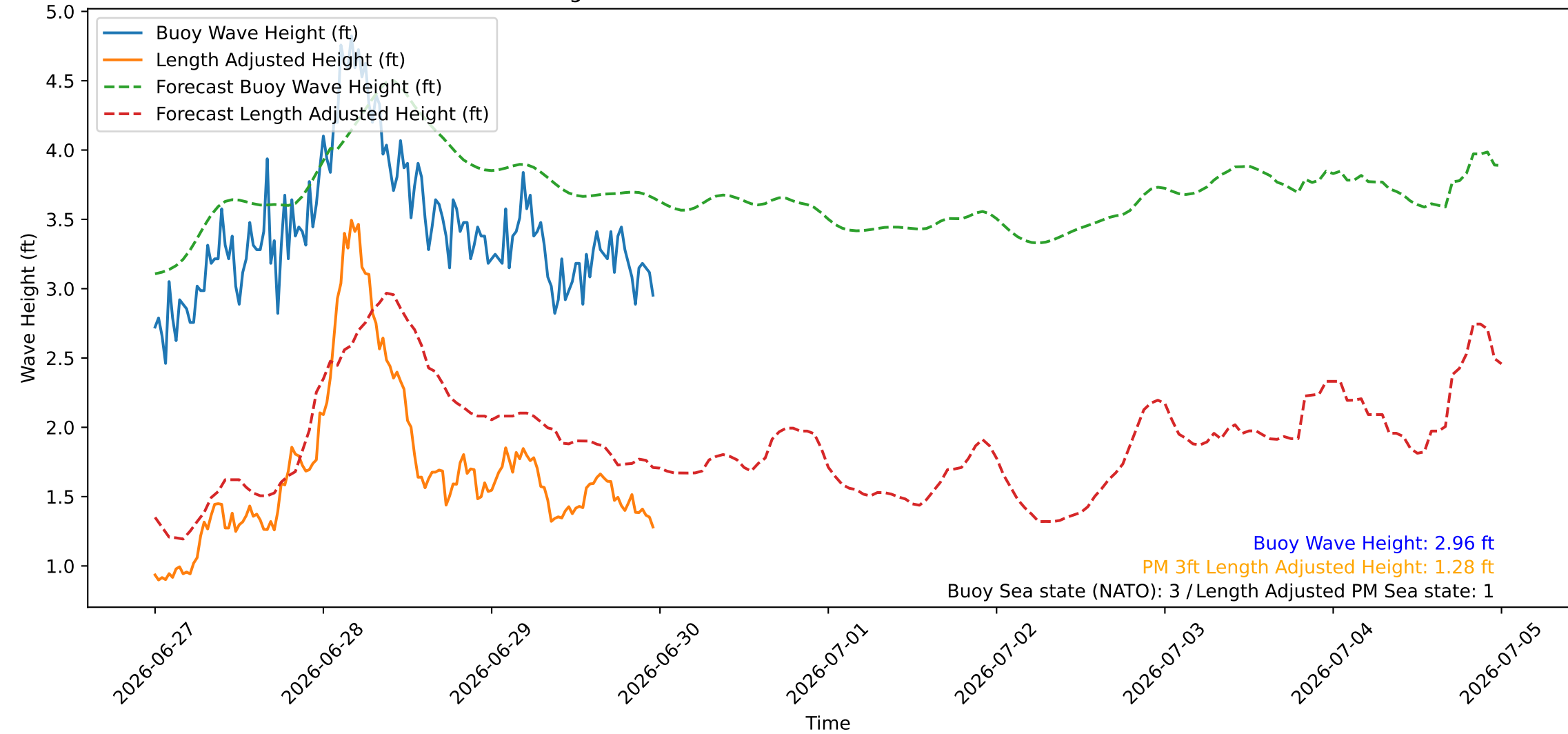
Wave Heights over Time for Green Beach at 2026-06-30 00:01:06
