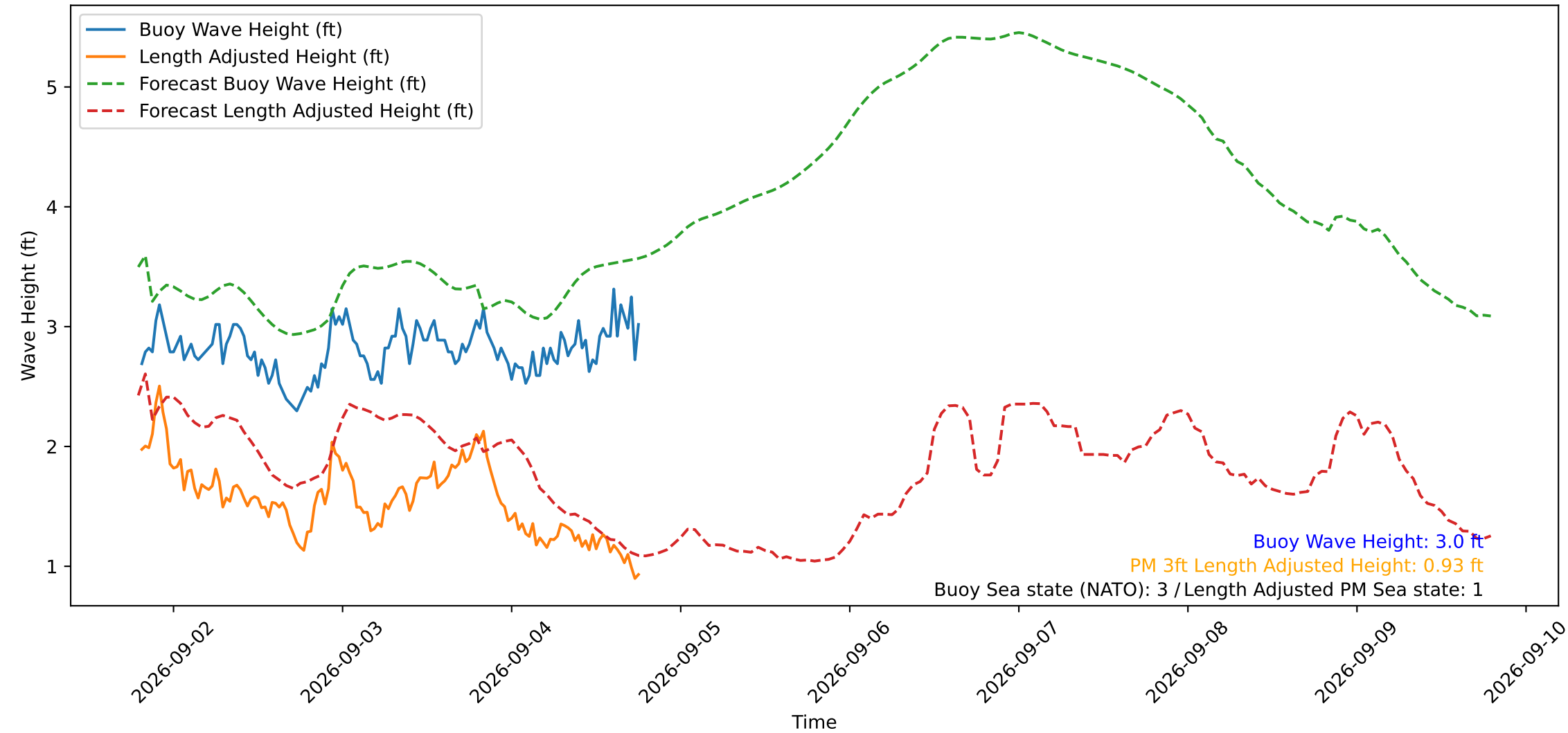
Wave Heights over Time for Red Beach at 2026-09-04 19:00:50
