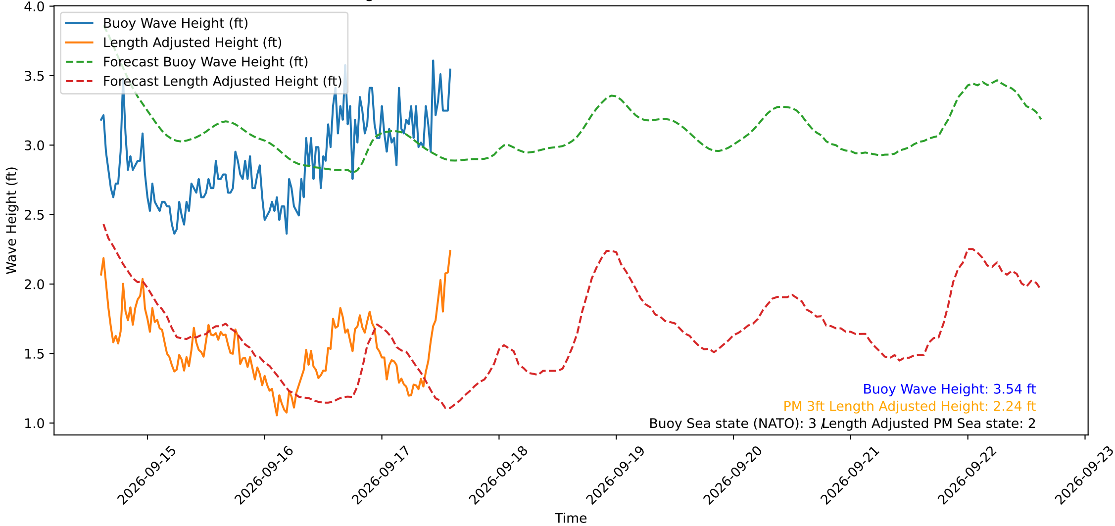
Wave Heights over Time for Oceanside Harbor at 2026-09-17 14:40:29
