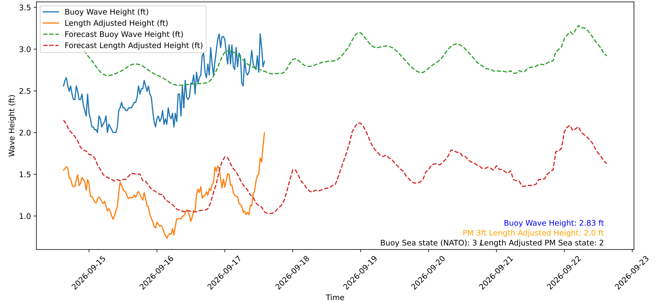
Wave Heights over Time for Red Beach at 2026-09-17 14:40:49
