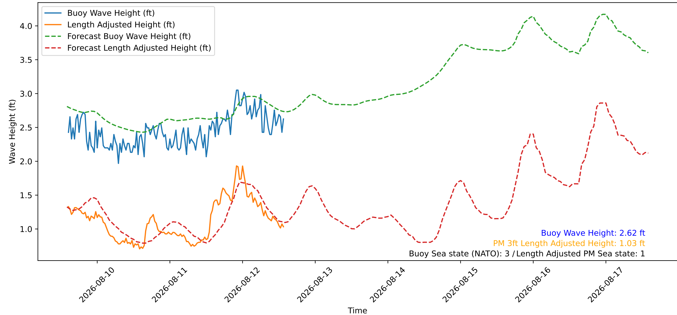
Wave Heights over Time for Oceanside Harbor at 2026-08-12 14:20:27
