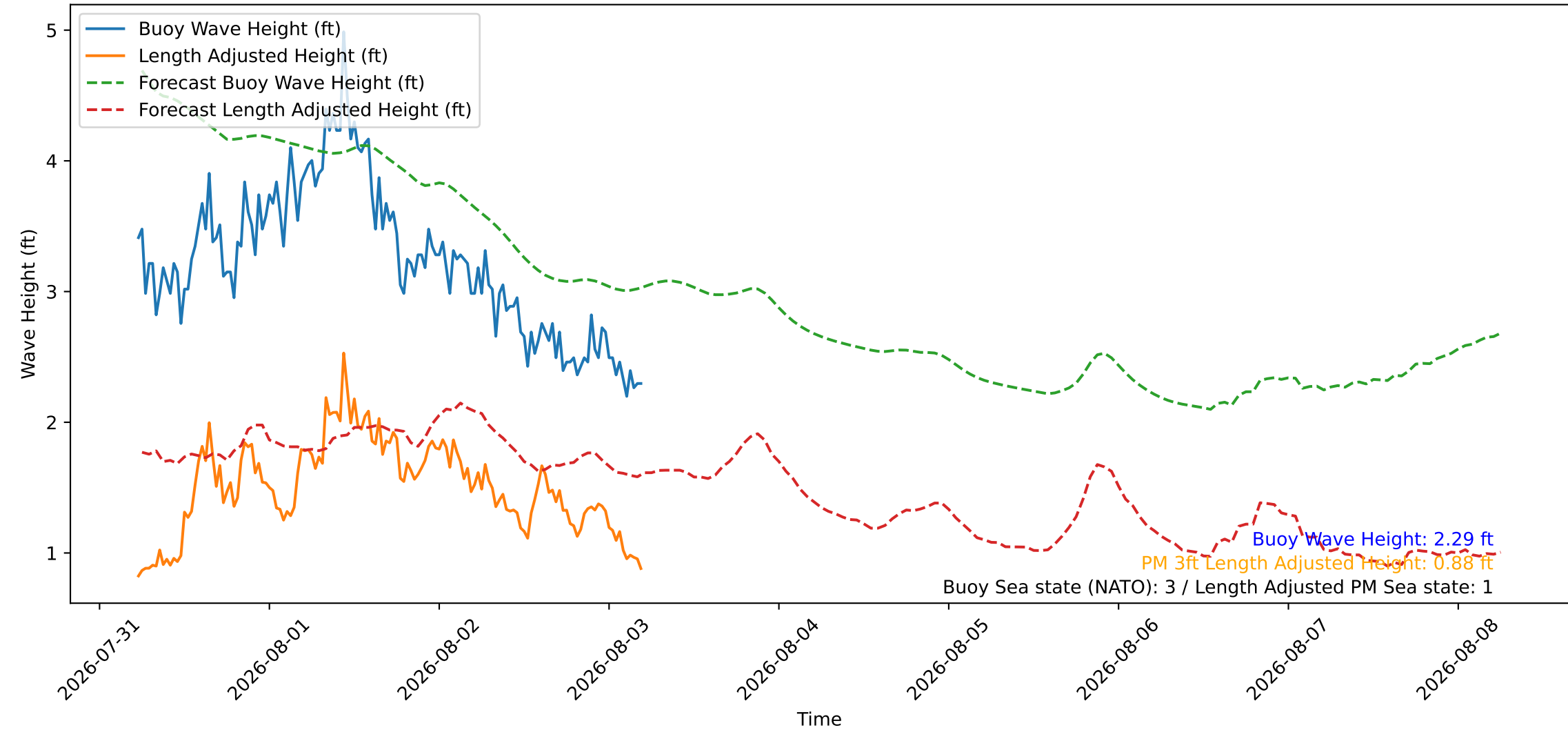
Wave Heights over Time for Green Beach at 2026-08-03 05:31:07
