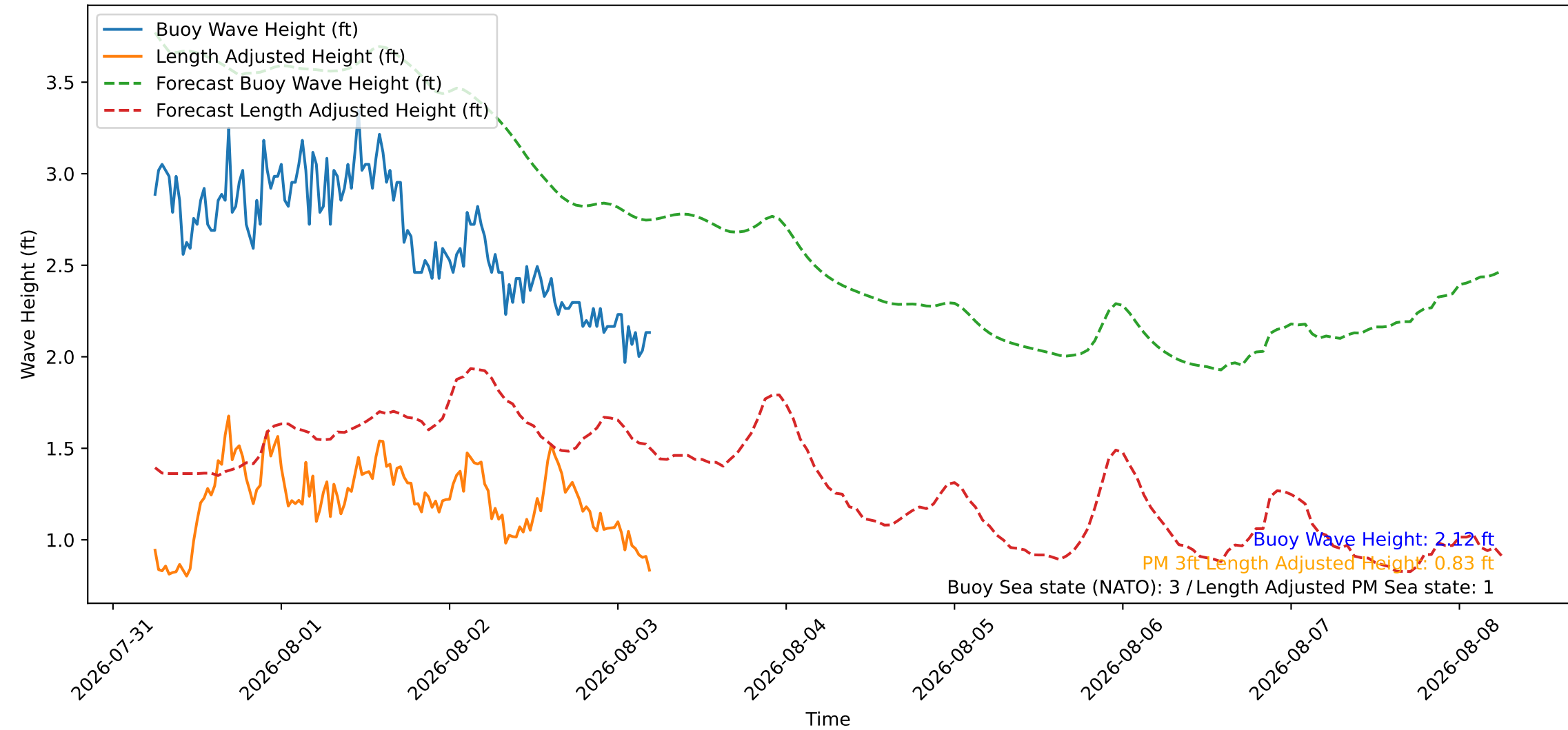
Wave Heights over Time for Red Beach at 2026-08-03 05:30:45
