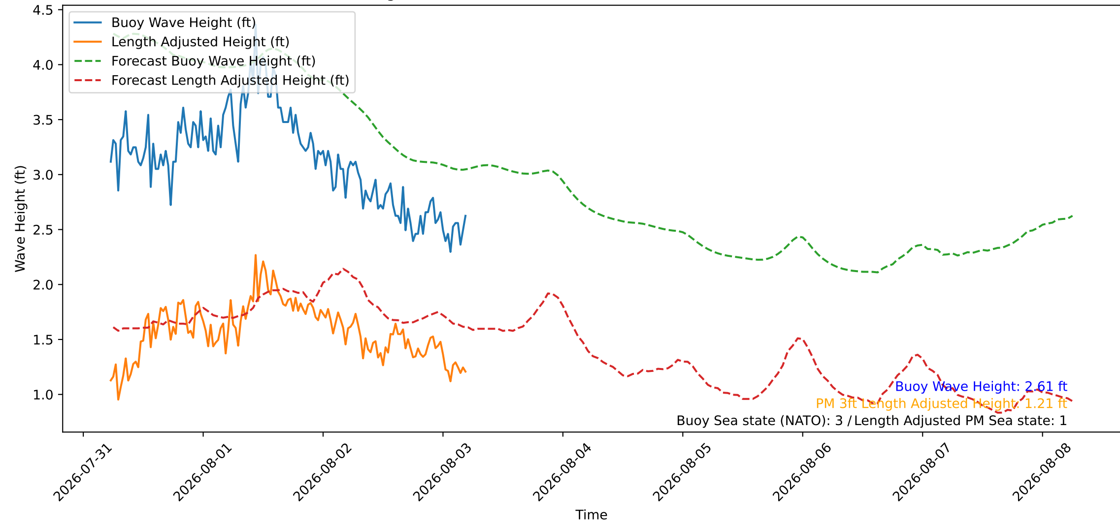
Wave Heights over Time for Oceanside Harbor at 2026-08-03 05:30:26
