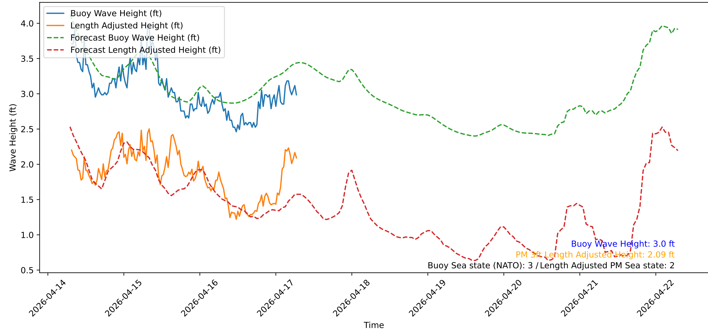
Wave Heights over Time for Green Beach at 2026-04-17 07:21:14
