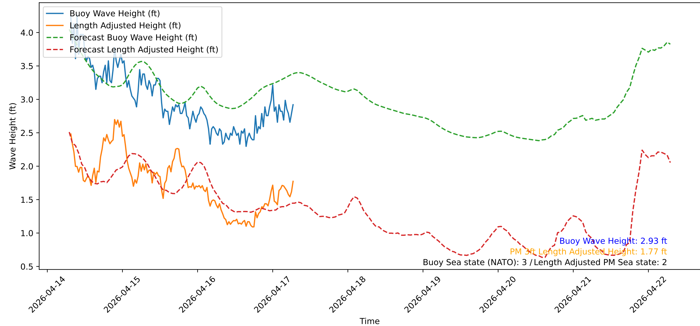
Wave Heights over Time for Oceanside Harbor at 2026-04-17 07:20:31
