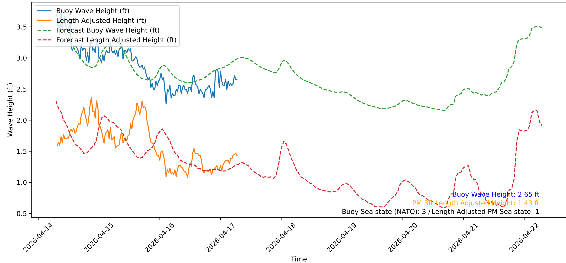
Wave Heights over Time for Red Beach at 2026-04-17 07:20:51
