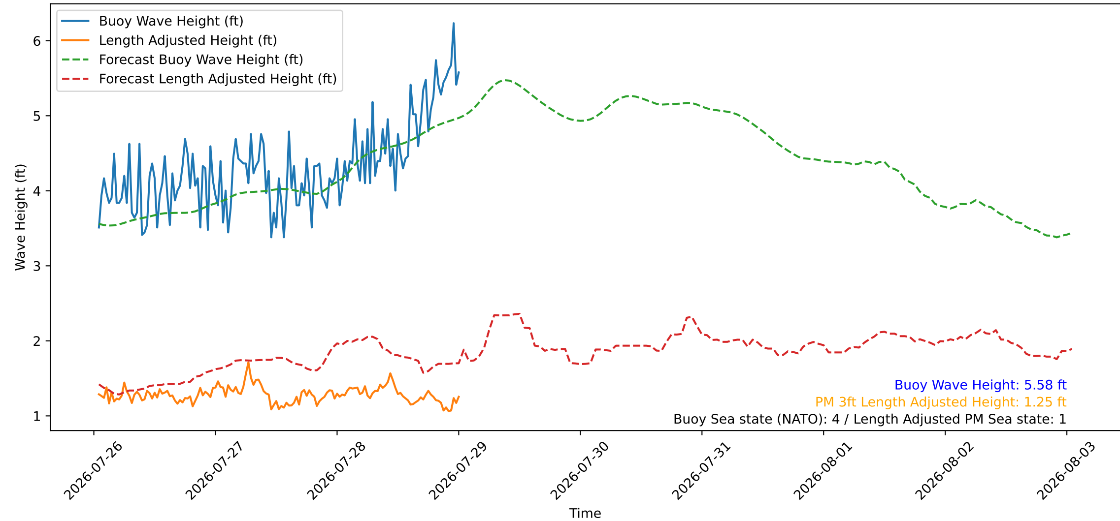
Wave Heights over Time for Green Beach at 2026-07-29 01:01:08
