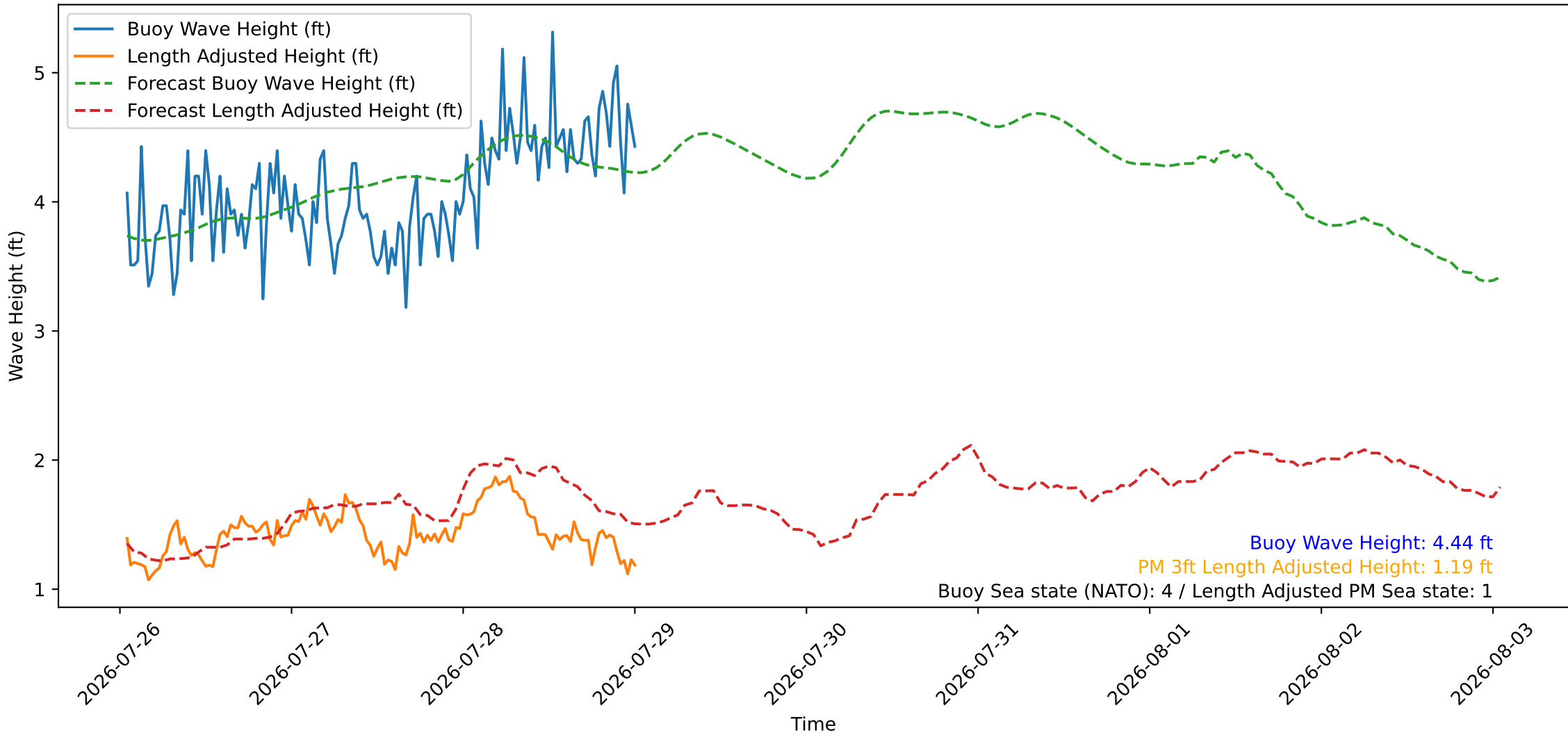
Wave Heights over Time for Oceanside Harbor at 2026-07-29 01:00:26
