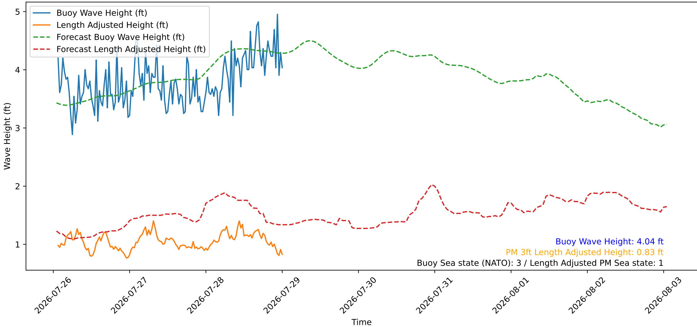
Wave Heights over Time for Red Beach at 2026-07-29 01:00:46
