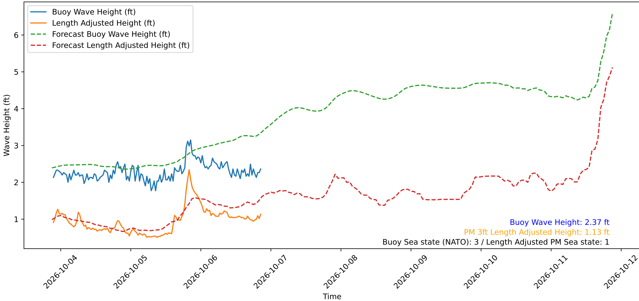
Wave Heights over Time for Green Beach at 2026-10-06 21:21:14
