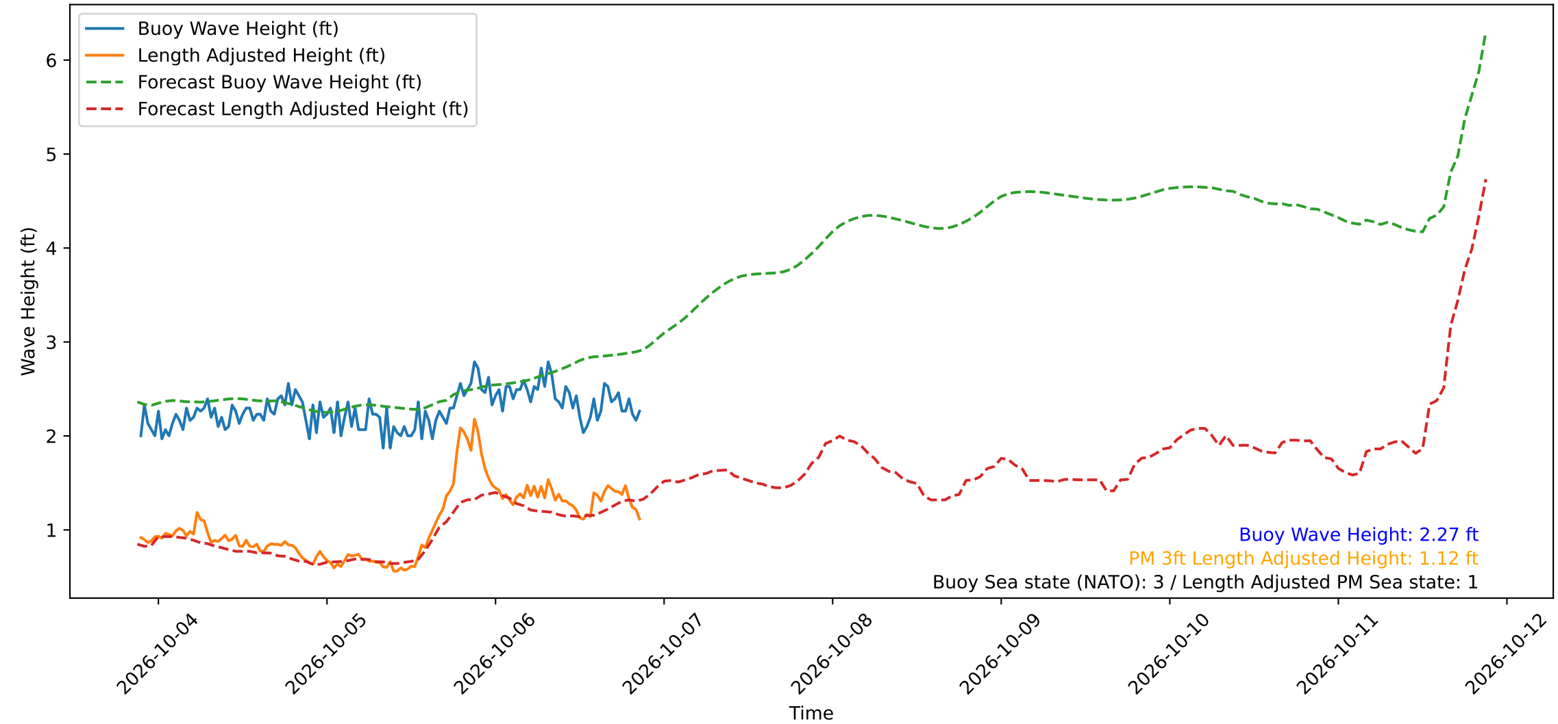
Wave Heights over Time for Oceanside Harbor at 2026-10-06 21:20:29
