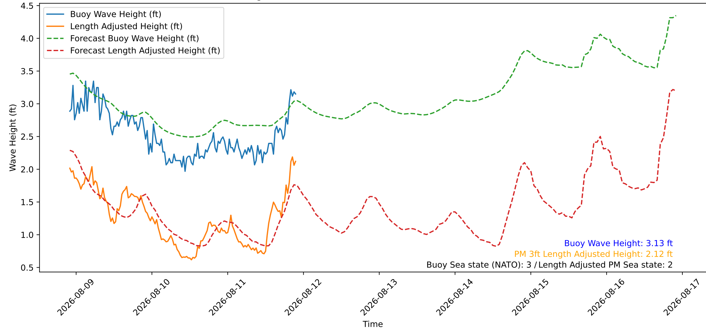
Wave Heights over Time for Green Beach at 2026-08-11 22:11:08
