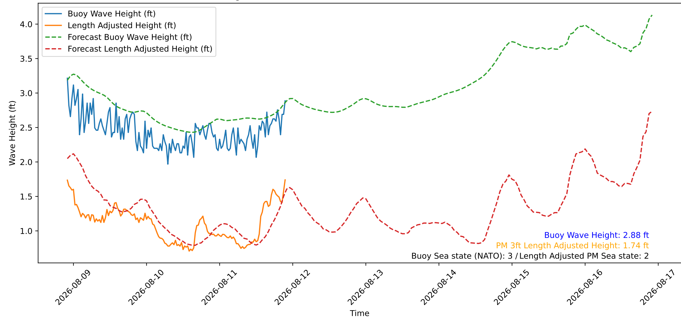
Wave Heights over Time for Oceanside Harbor at 2026-08-11 22:10:26
