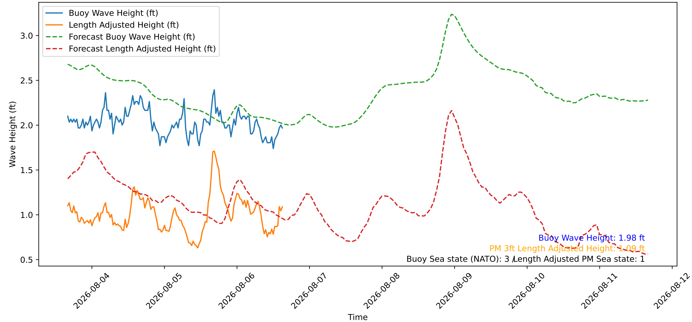
Wave Heights over Time for Red Beach at 2026-08-06 15:50:47
