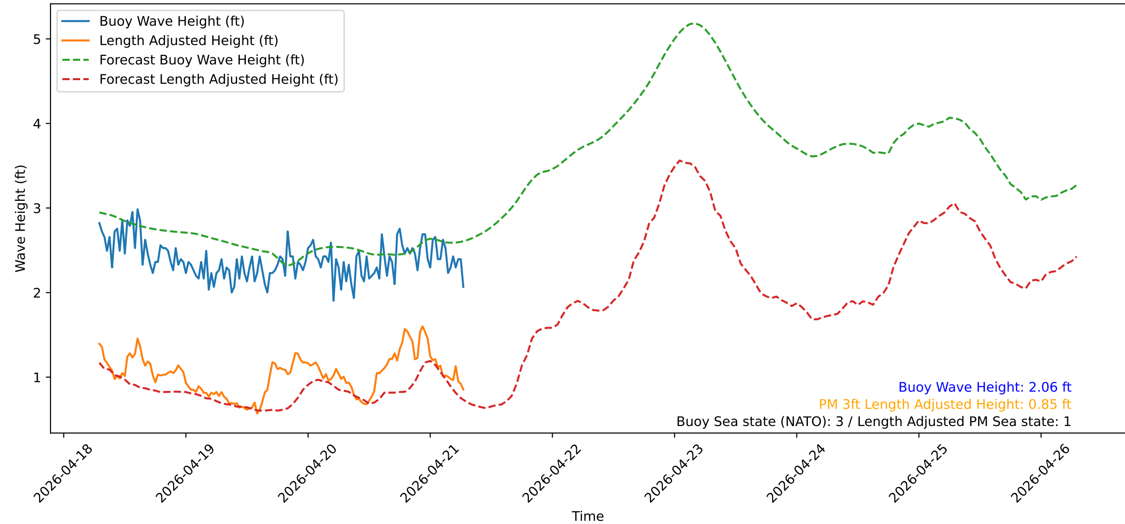
Wave Heights over Time for Oceanside Harbor at 2026-04-21 07:00:32
