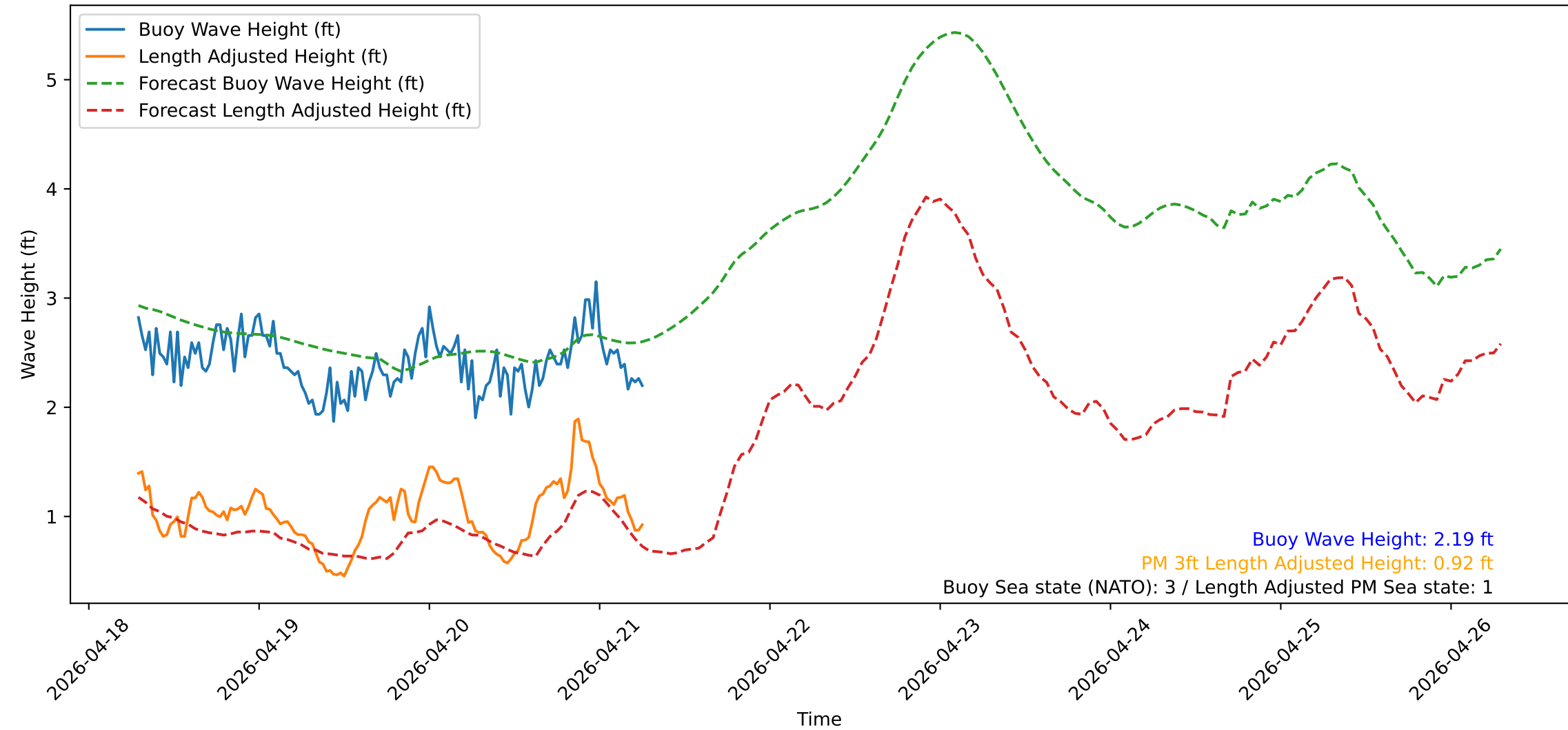
Wave Heights over Time for Green Beach at 2026-04-21 07:01:15
