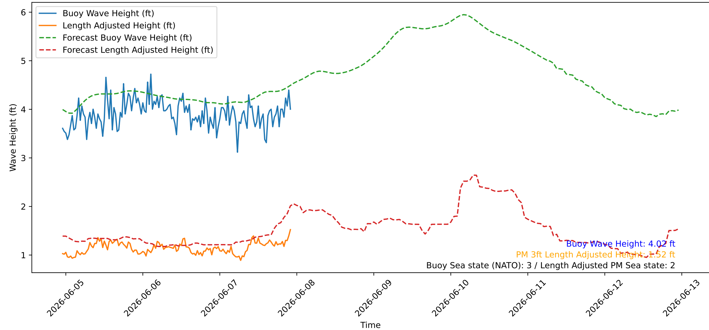
Wave Heights over Time for Green Beach at 2026-06-07 22:51:10
