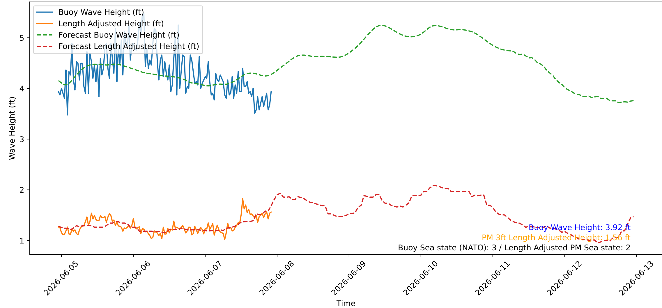
Wave Heights over Time for Oceanside Harbor at 2026-06-07 22:50:26
