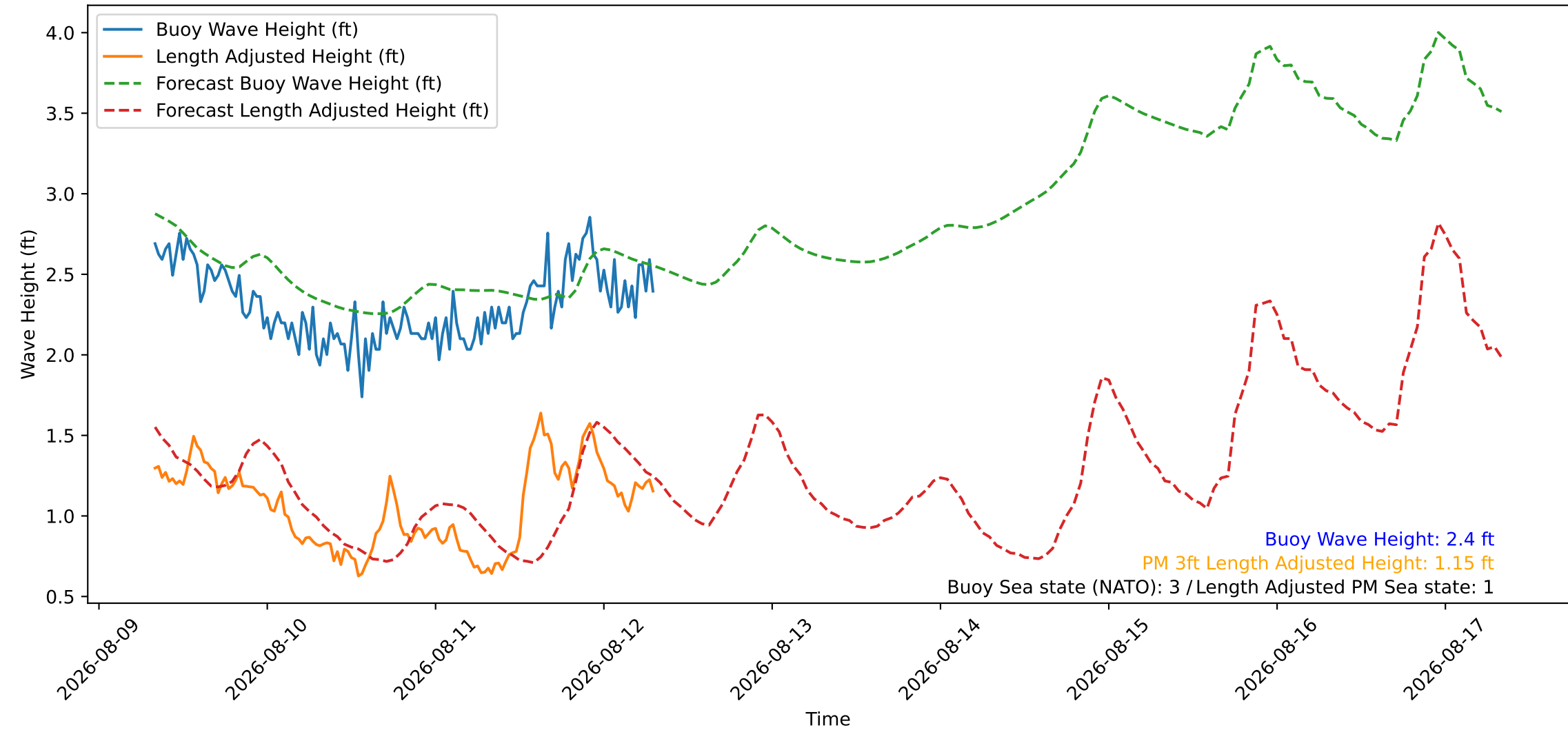
Wave Heights over Time for Red Beach at 2026-08-12 07:50:48
