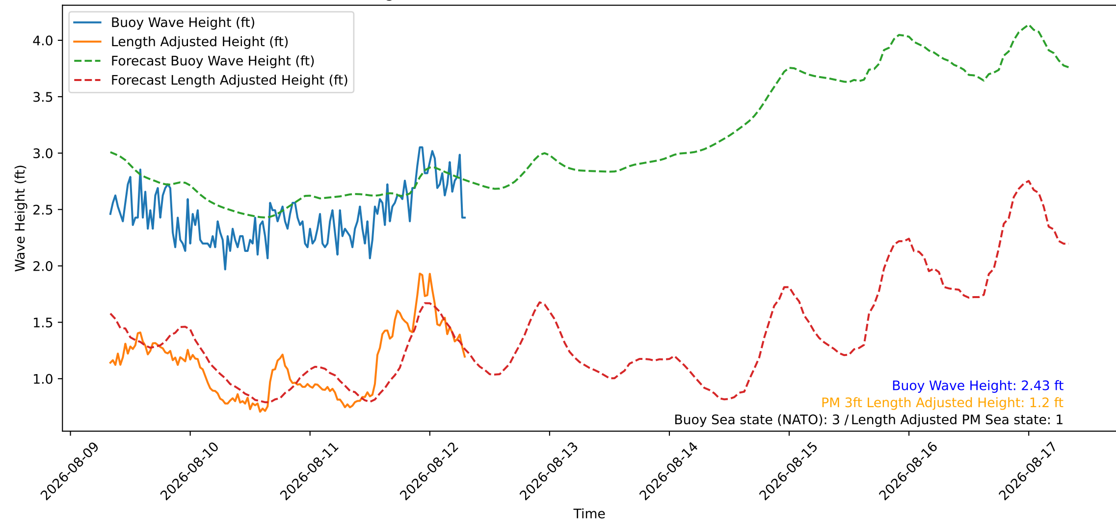
Wave Heights over Time for Oceanside Harbor at 2026-08-12 07:50:27
