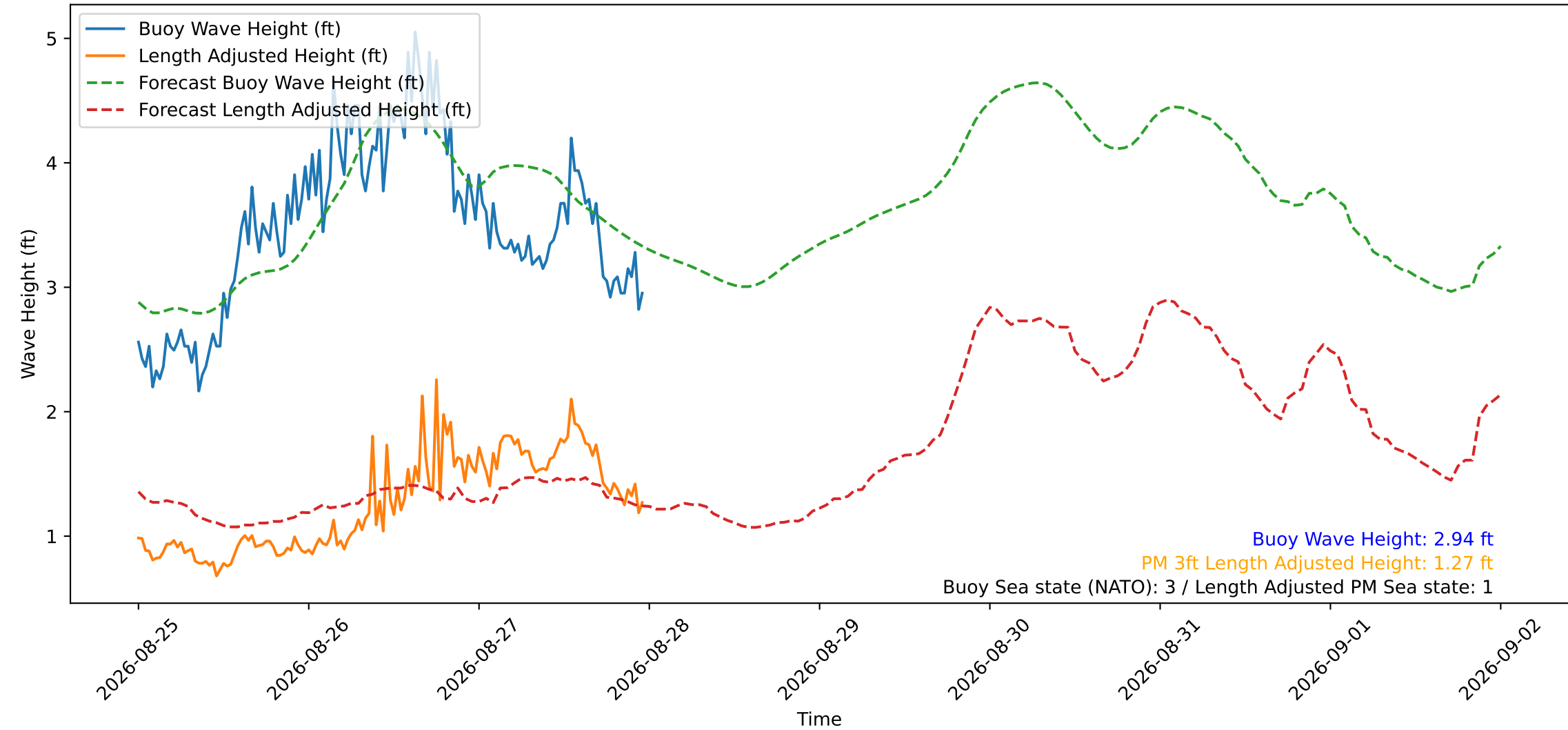
Wave Heights over Time for Red Beach at 2026-08-27 23:40:49
