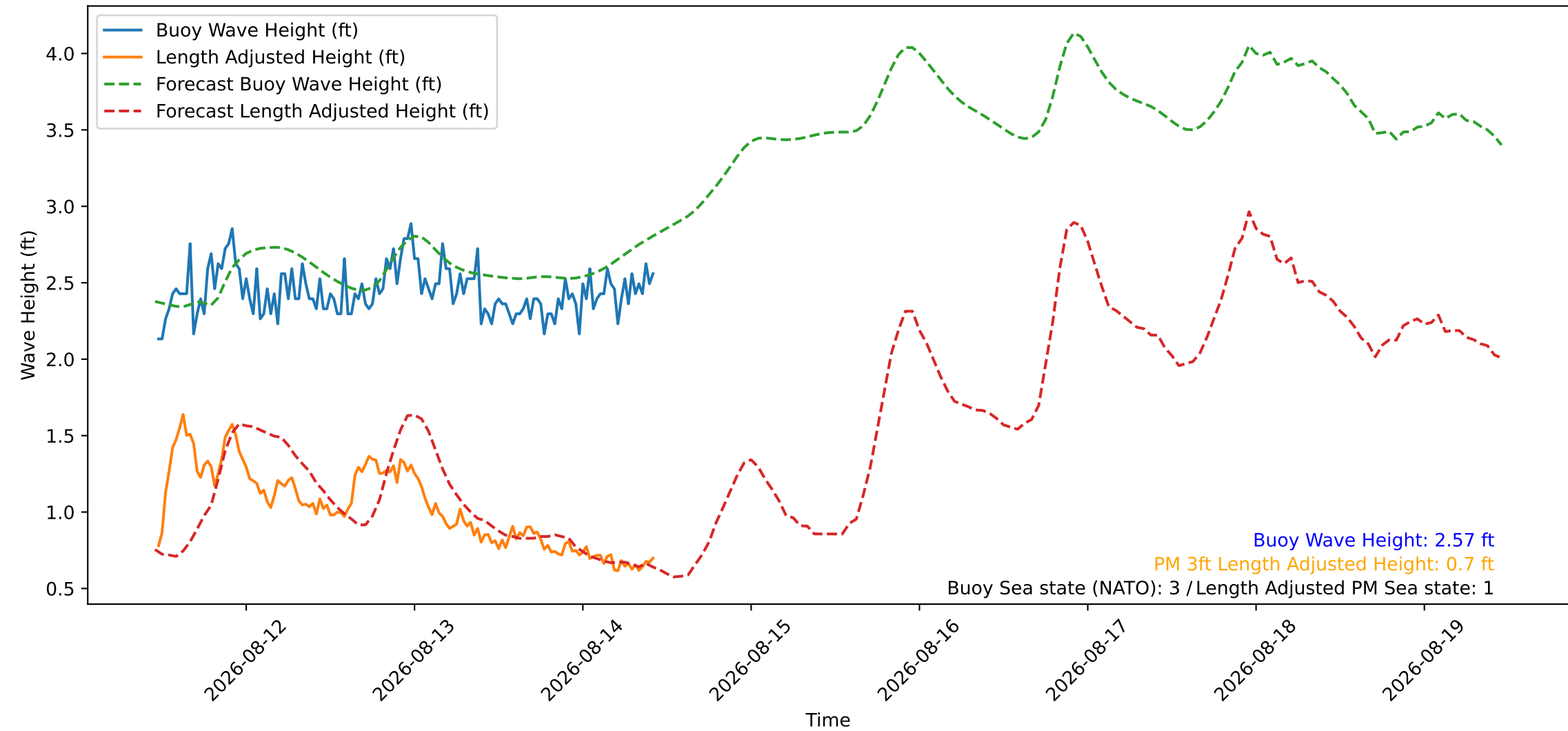
Wave Heights over Time for Red Beach at 2026-08-14 11:10:47
