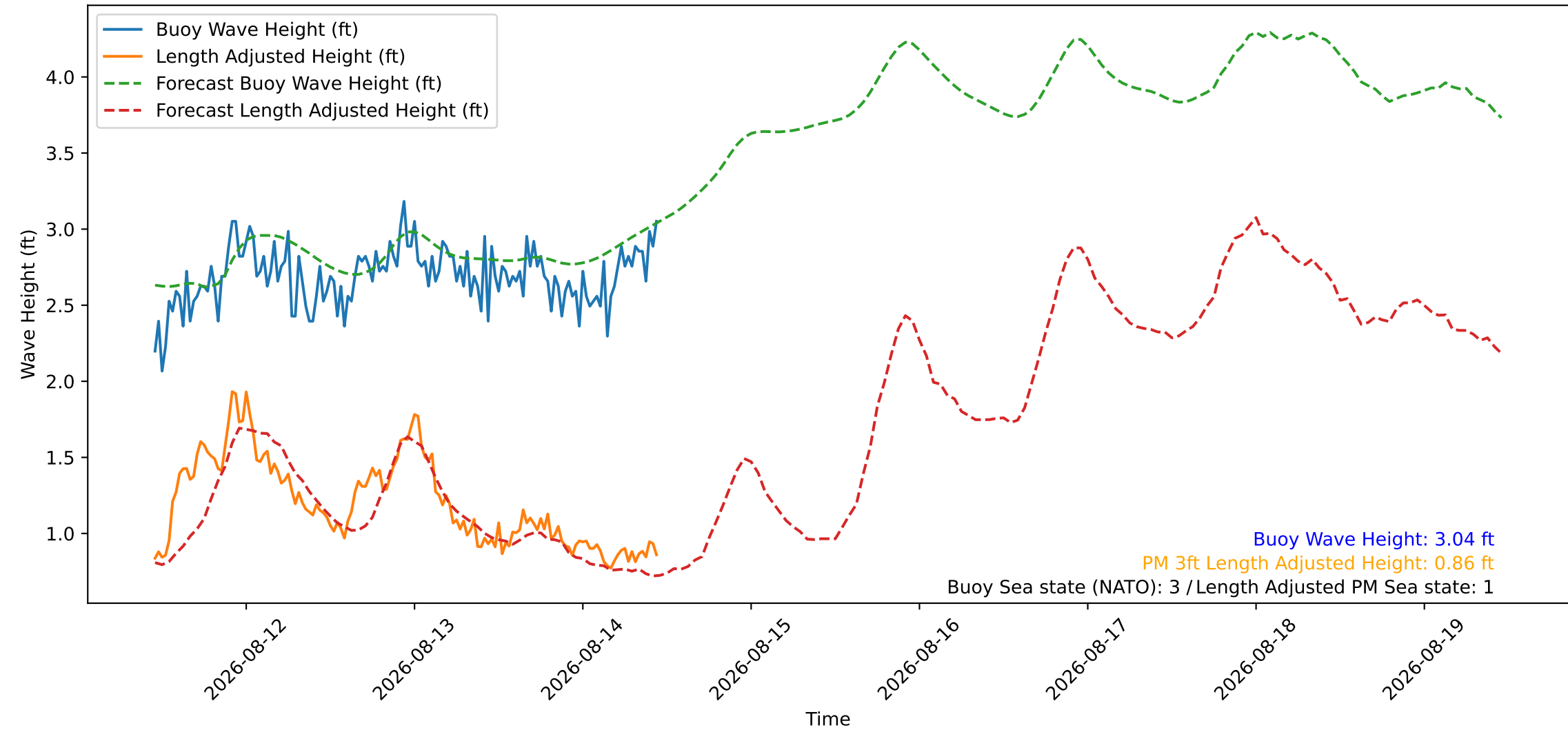
Wave Heights over Time for Oceanside Harbor at 2026-08-14 11:10:27
