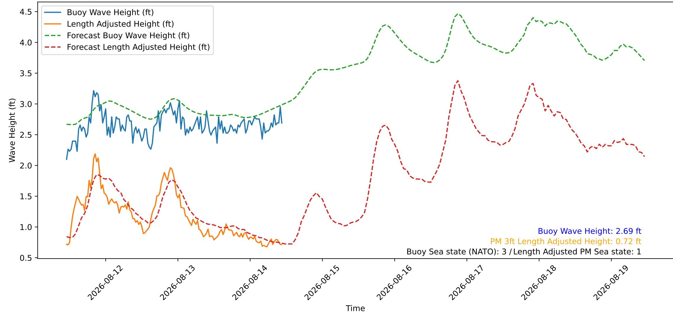
Wave Heights over Time for Green Beach at 2026-08-14 11:11:09
