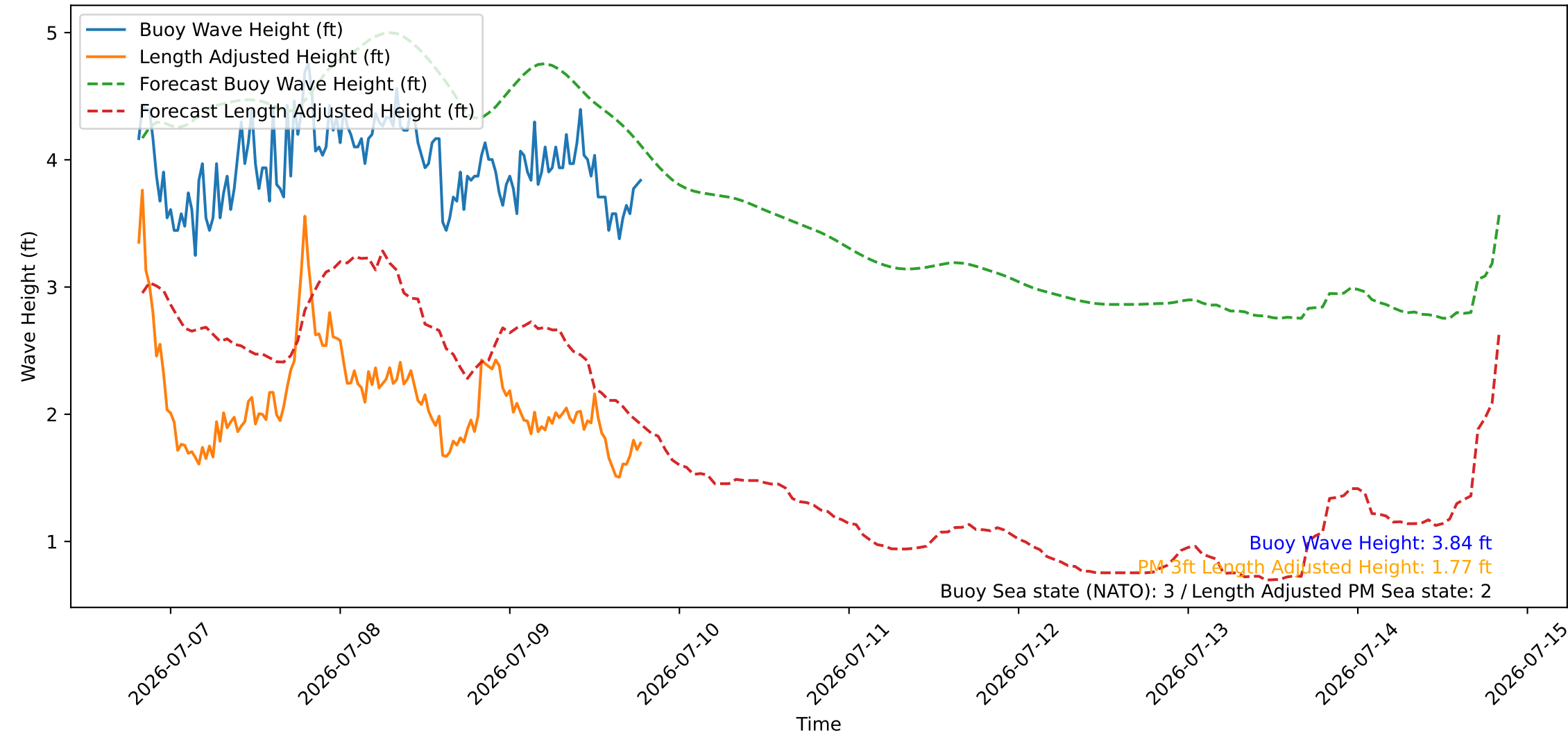
Wave Heights over Time for Green Beach at 2026-07-09 19:31:08
