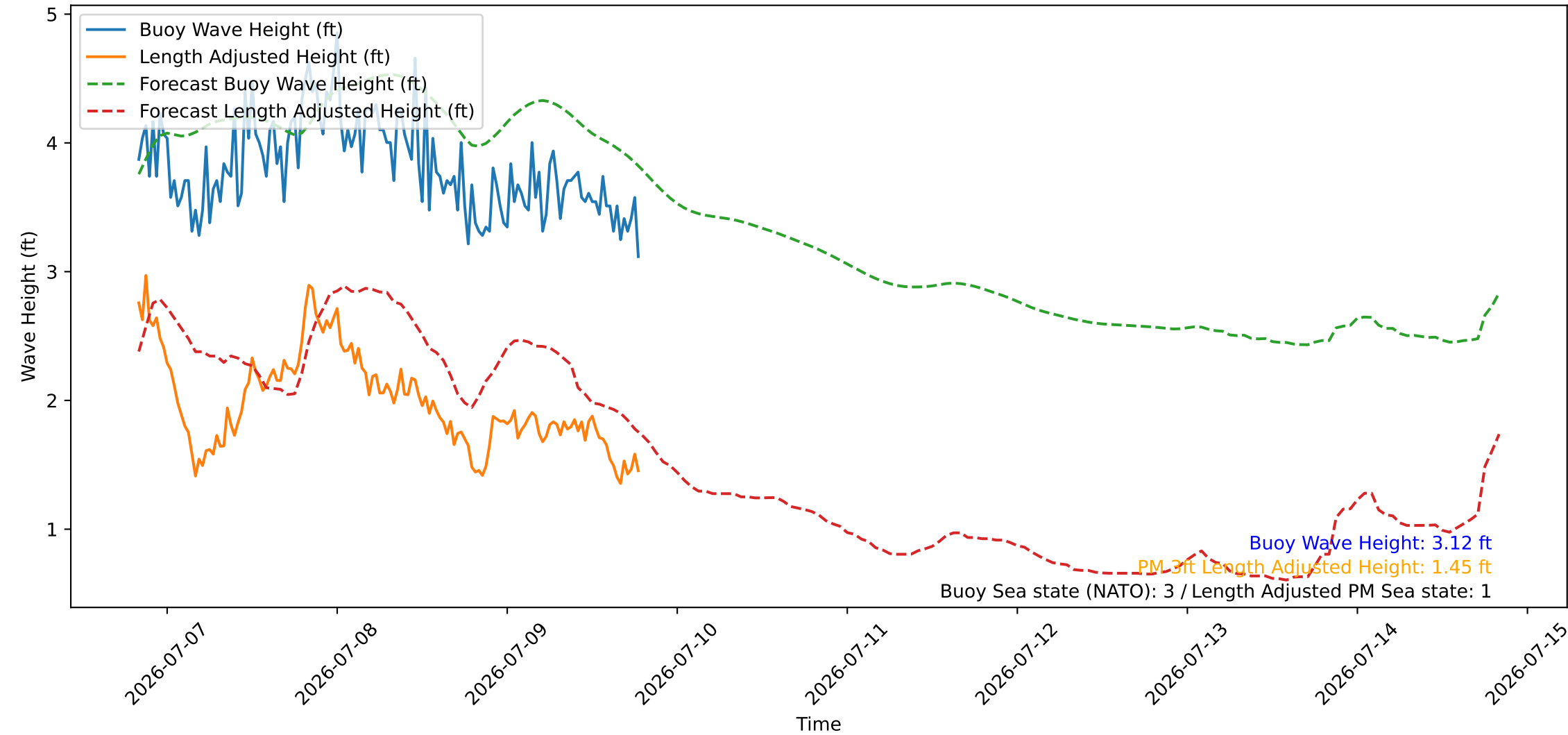
Wave Heights over Time for Red Beach at 2026-07-09 19:30:46
