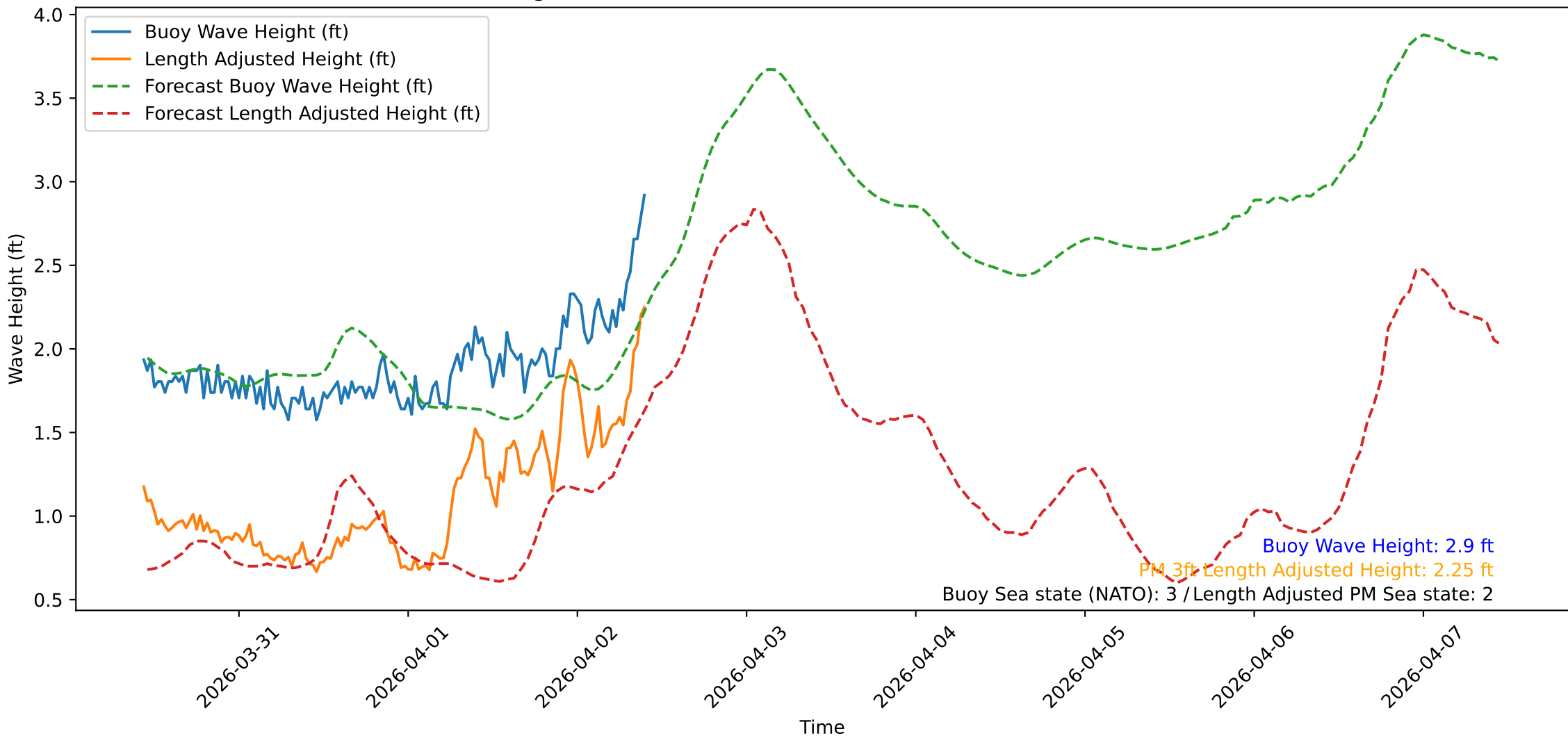
Wave Heights over Time for Oceanside Harbor at 2026-04-02 10:30:32
