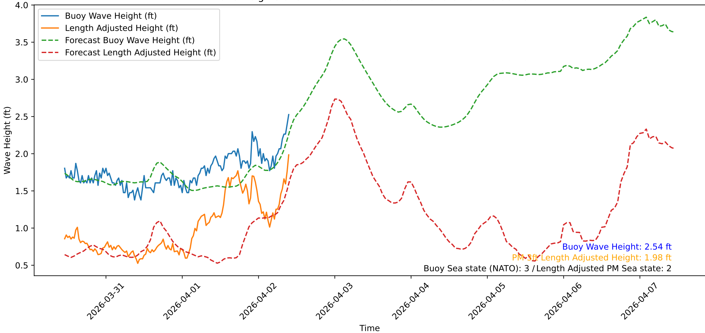
Wave Heights over Time for Red Beach at 2026-04-02 10:30:48
