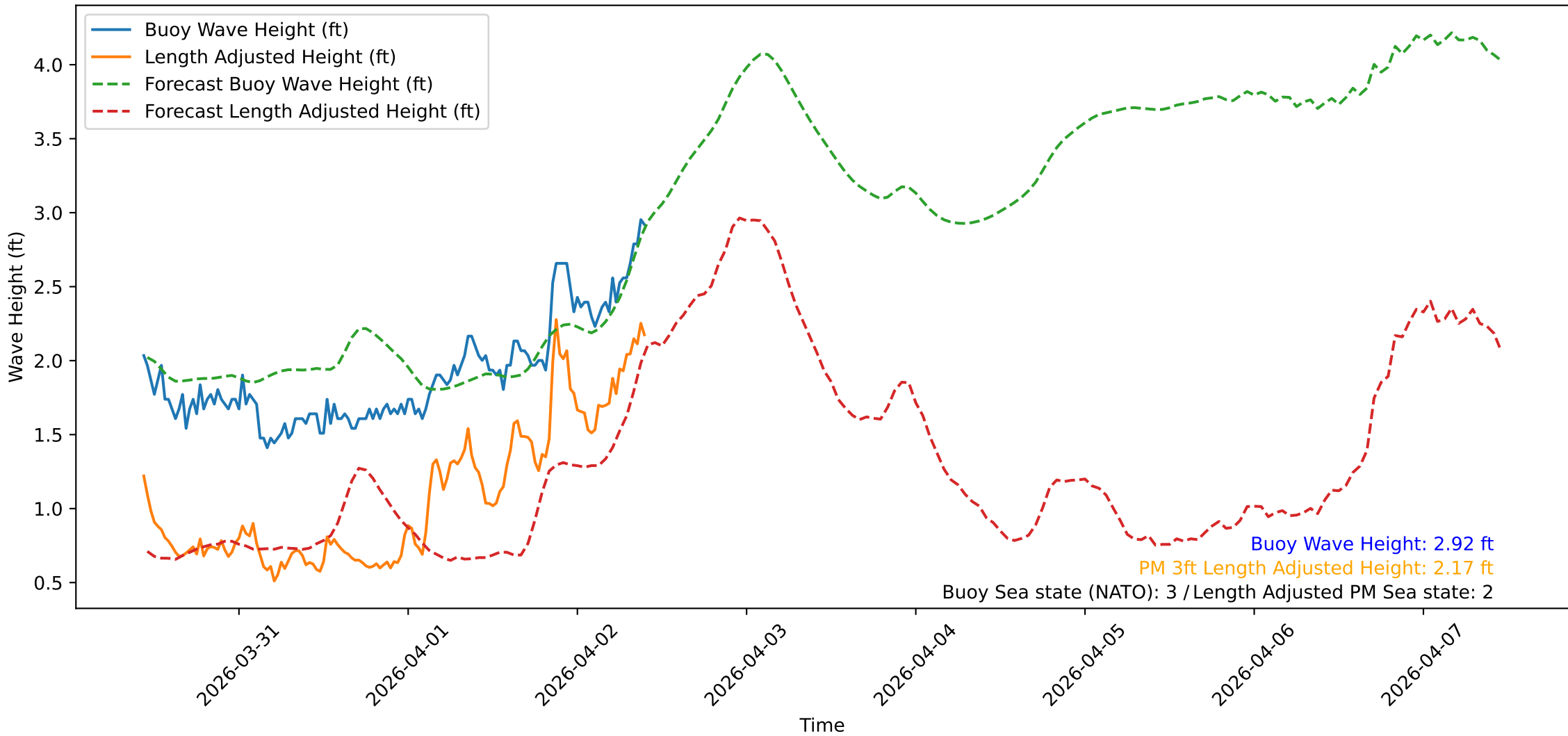
Wave Heights over Time for Green Beach at 2026-04-02 10:31:11
