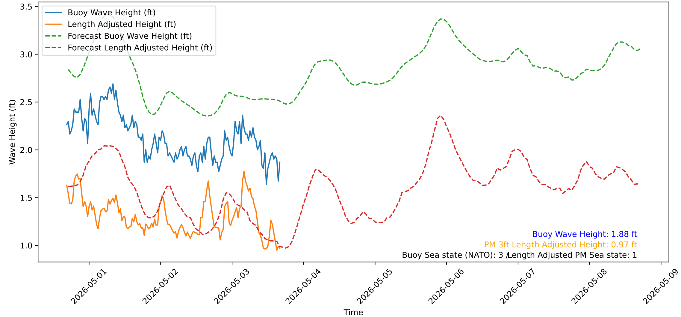
Wave Heights over Time for Oceanside Harbor at 2026-05-03 16:40:31
