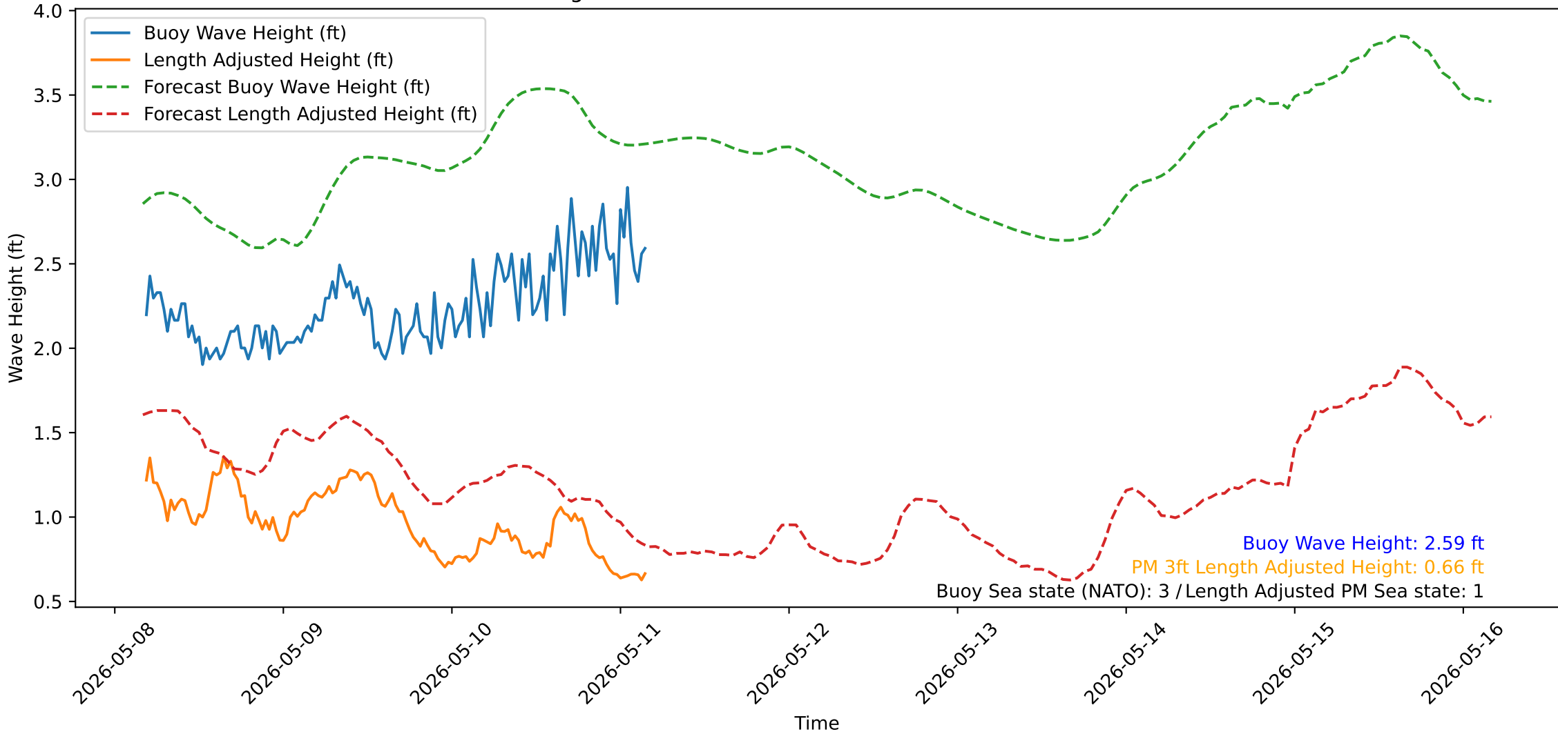
Wave Heights over Time for Red Beach at 2026-05-11 04:20:51
