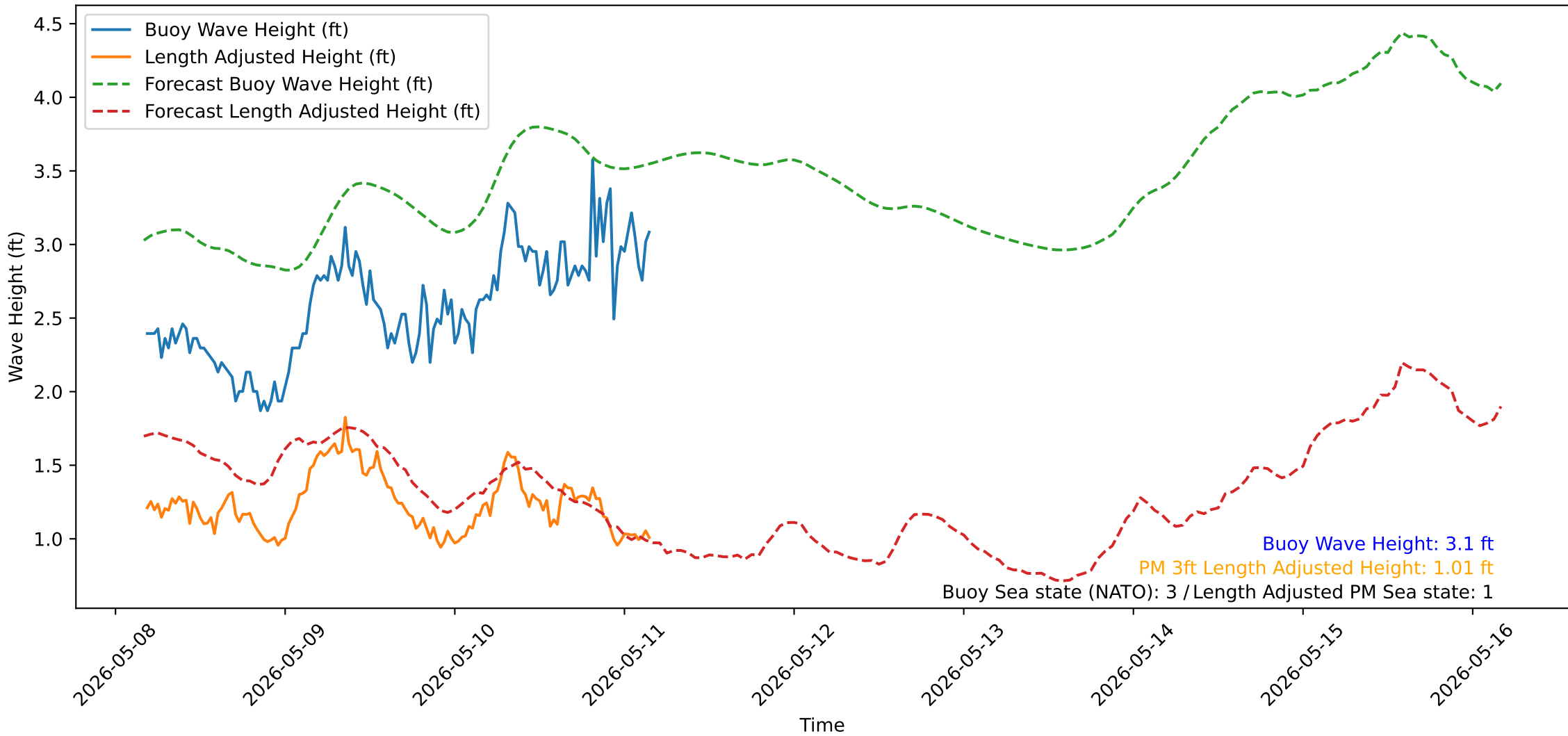
Wave Heights over Time for Oceanside Harbor at 2026-05-11 04:20:31
