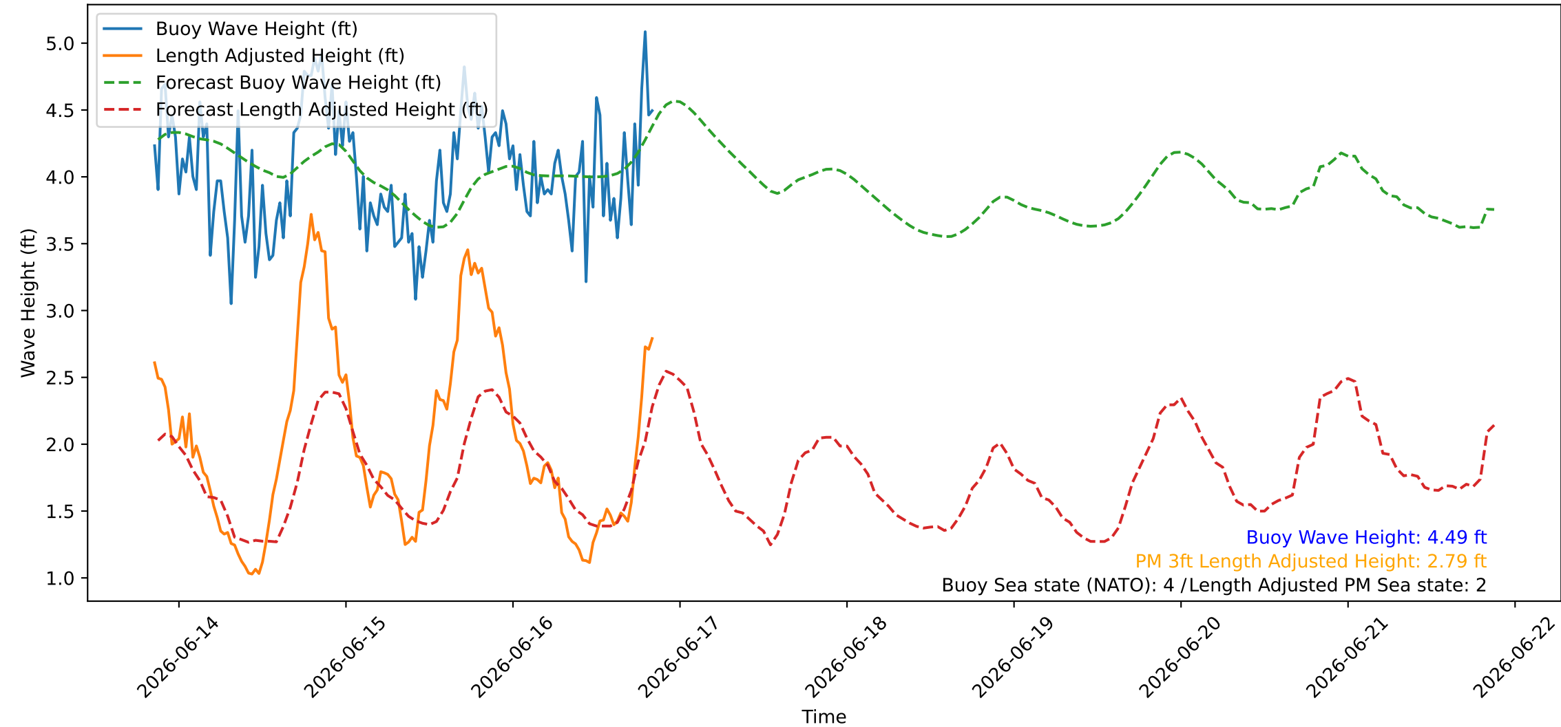
Wave Heights over Time for Green Beach at 2026-06-16 20:41:13
