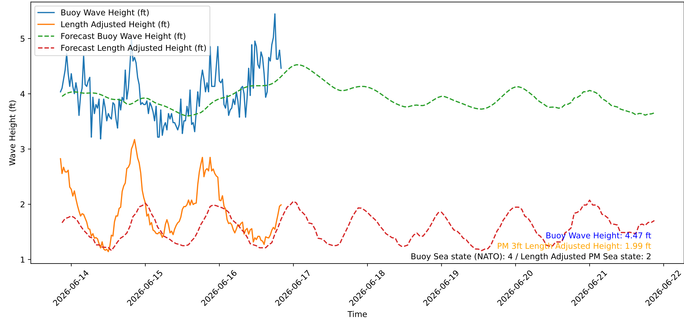
Wave Heights over Time for Oceanside Harbor at 2026-06-16 20:40:27
