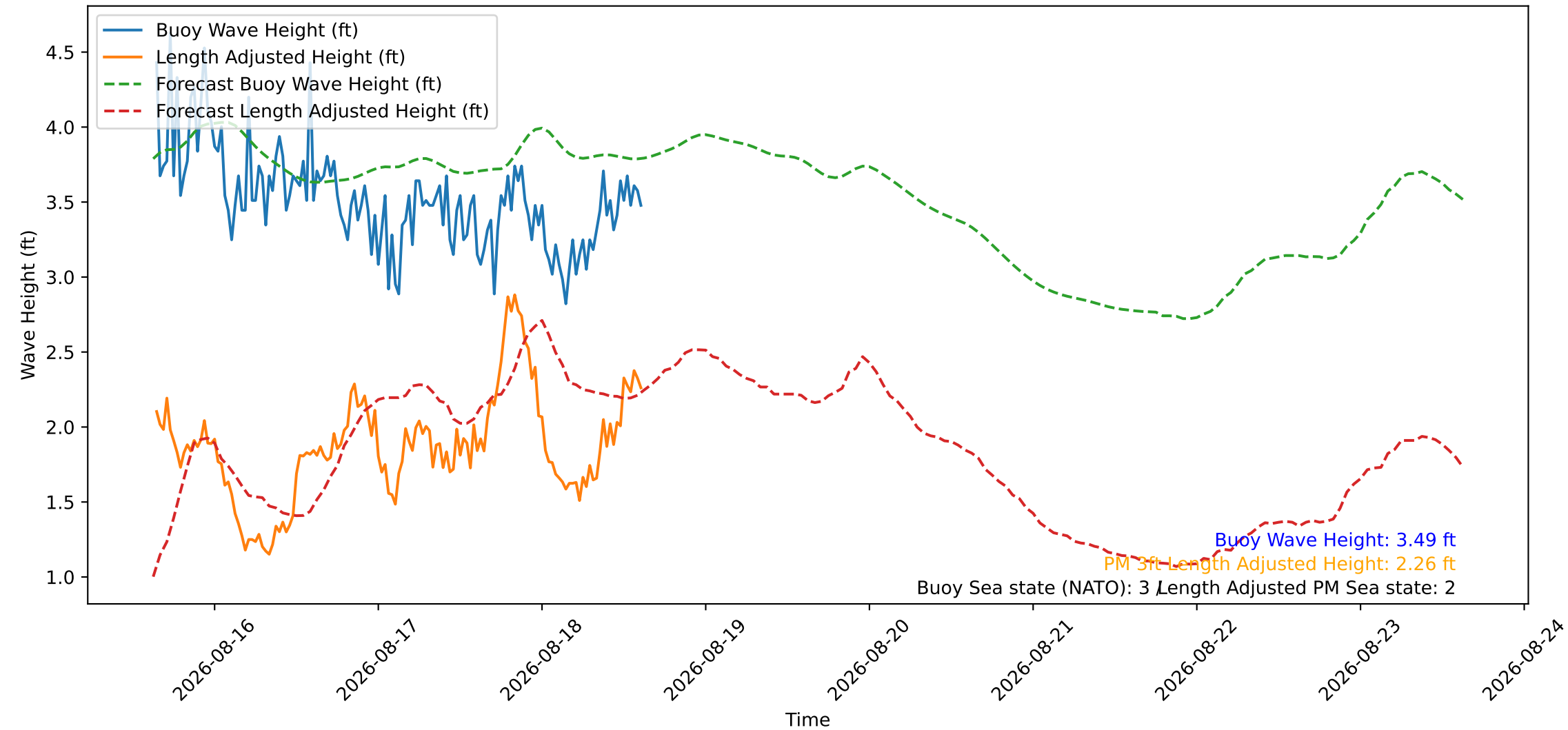
Wave Heights over Time for Oceanside Harbor at 2026-08-18 15:20:25
