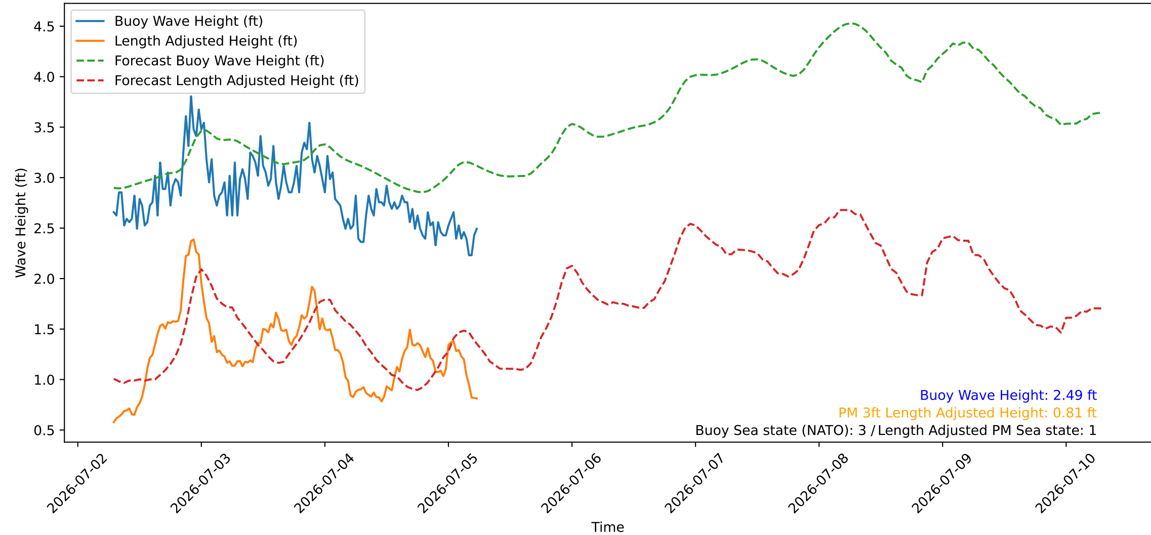
Wave Heights over Time for Red Beach at 2026-07-05 06:30:46
