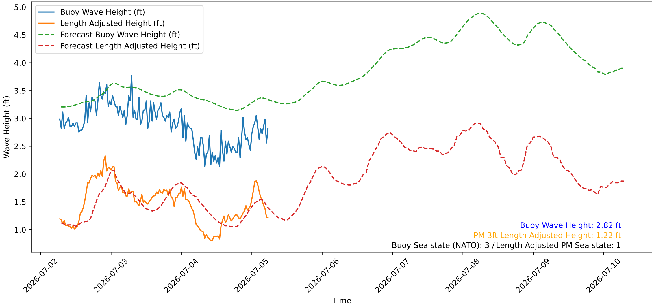
Wave Heights over Time for Oceanside Harbor at 2026-07-05 06:30:26
