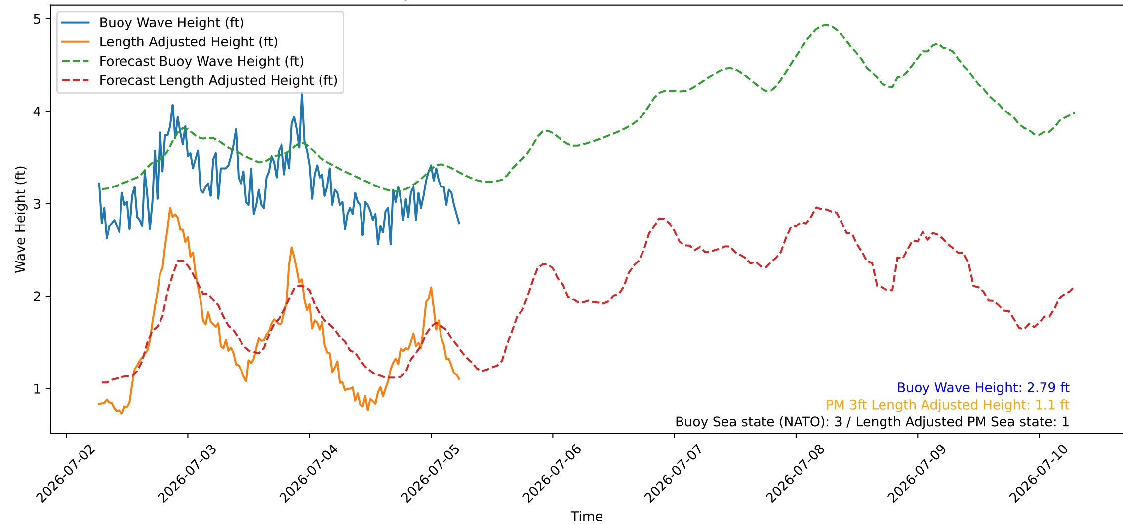
Wave Heights over Time for Green Beach at 2026-07-05 06:31:08
