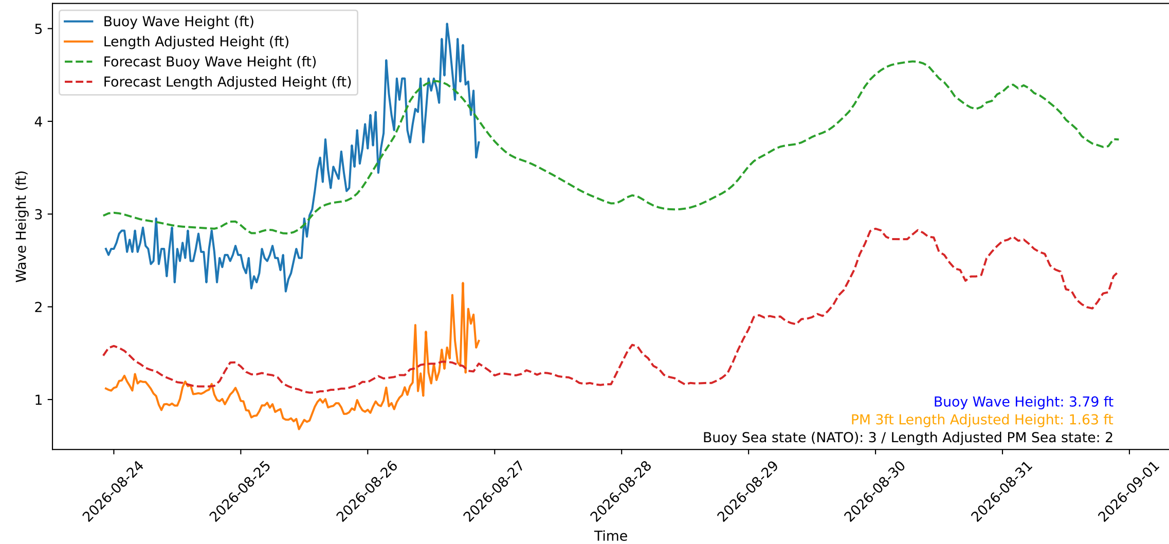
Wave Heights over Time for Red Beach at 2026-08-26 22:00:49
