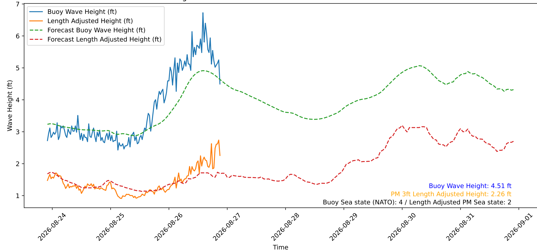
Wave Heights over Time for Oceanside Harbor at 2026-08-26 22:00:30
