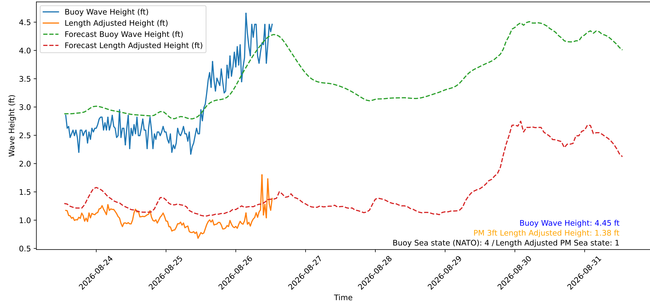
Wave Heights over Time for Red Beach at 2026-08-26 13:20:53
