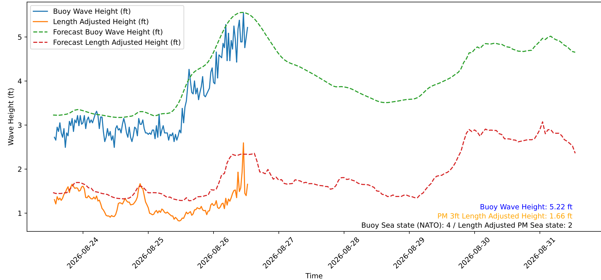
Wave Heights over Time for Green Beach at 2026-08-26 13:21:18
