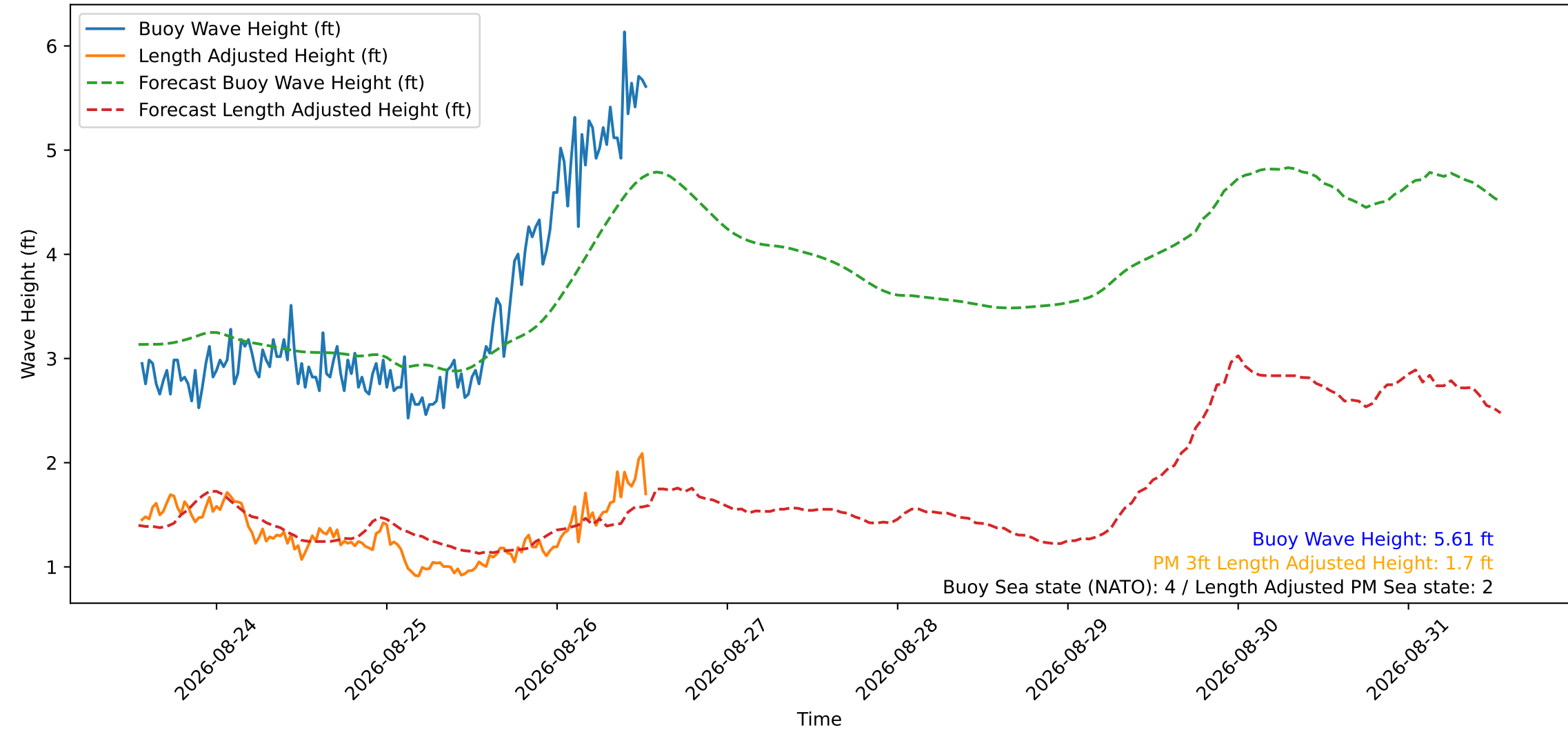
Wave Heights over Time for Oceanside Harbor at 2026-08-26 13:20:31
