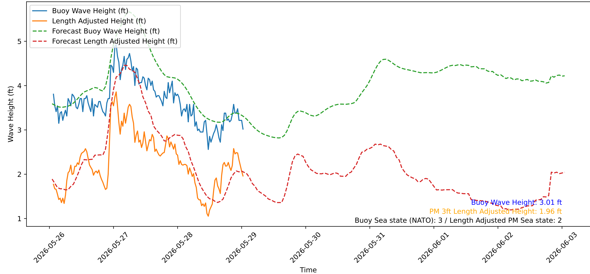
Wave Heights over Time for Green Beach at 2026-05-29 01:21:03
