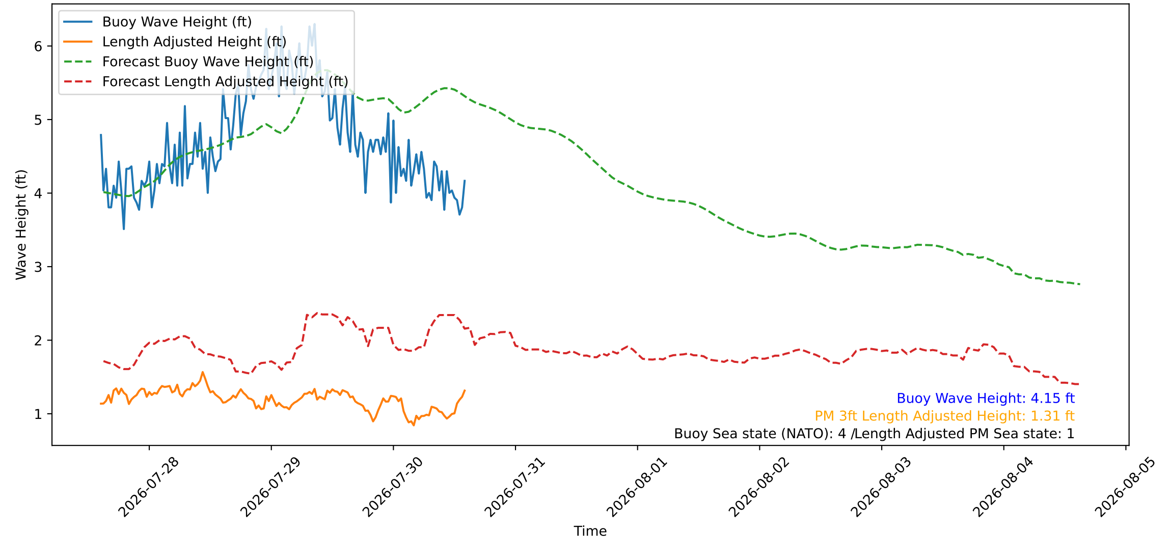
Wave Heights over Time for Green Beach at 2026-07-30 14:41:09
