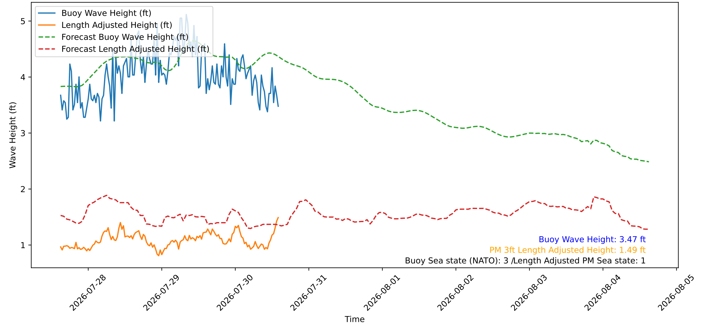
Wave Heights over Time for Red Beach at 2026-07-30 14:40:47
