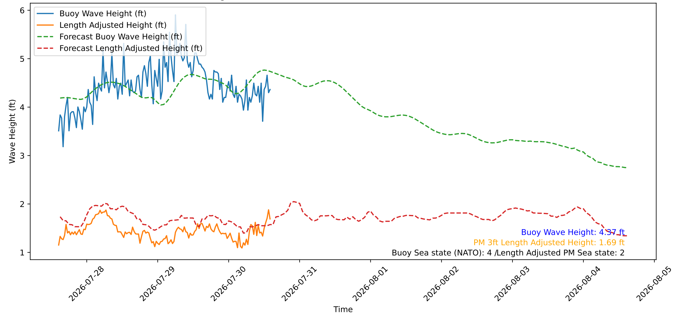
Wave Heights over Time for Oceanside Harbor at 2026-07-30 14:40:27
