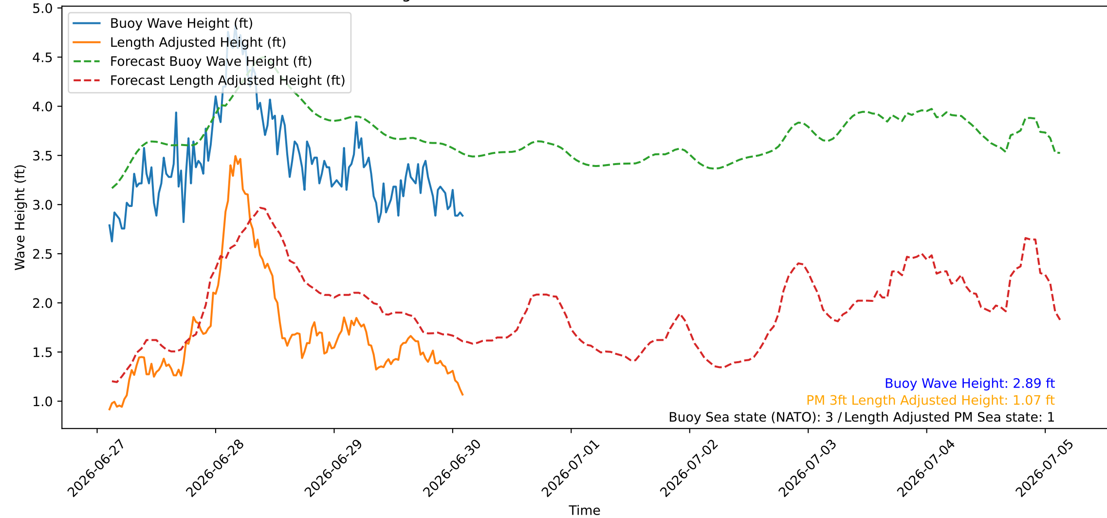
Wave Heights over Time for Green Beach at 2026-06-30 02:41:09
