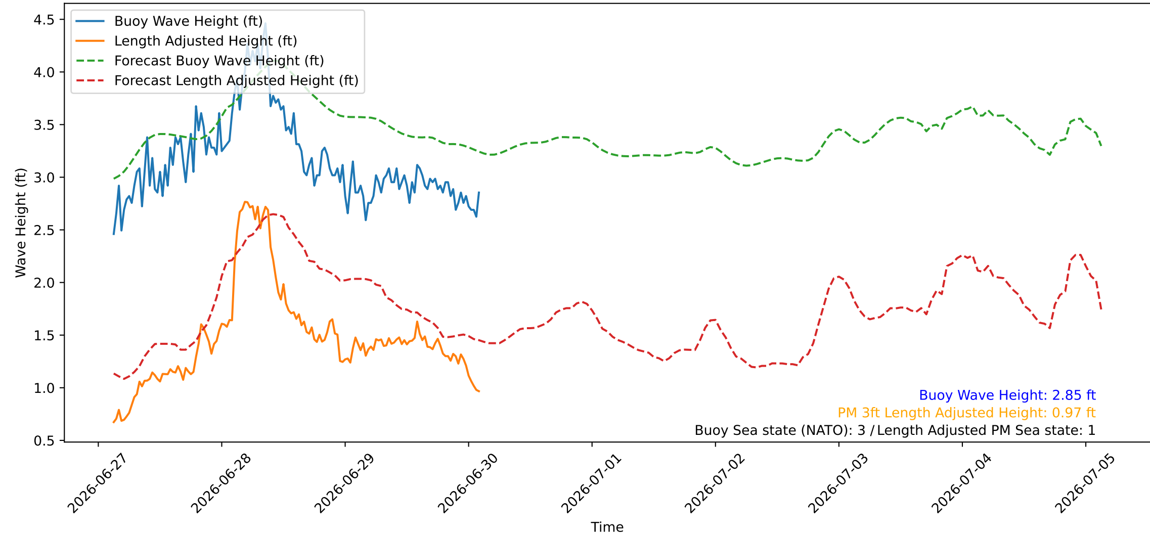
Wave Heights over Time for Red Beach at 2026-06-30 02:40:46
